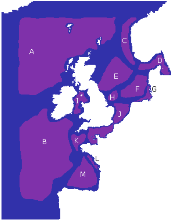
Figure 7. The 13 key regions drawn from identified based on the regionalisation found in Fig. 6, labelled A-M (purple). Each region aims to cover an area with few intersecting boundaries, without crossing locations with a high number of boundaries. Any area not assigned to one of these regions (blue) is due to uncertainty resulting from either domain boundaries or region boundaries.
