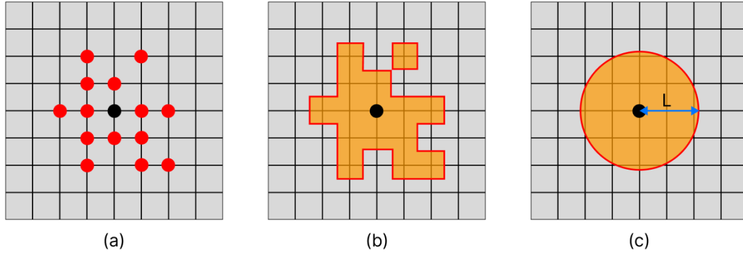
Figure 3. Method for calculating the lengthscale-length-scale of a given node in a network representing the horizontal connectivity of a variable. Panel (a) shows the target node (black) and each of the nodes on the grid that it is linked with (red). Panel (b) shows the area represented by each of the nodes linked to the current target node. Panel (c) shows a circle with equivalent area to the area covered in Panel (b), and the radius L , provides us with our approximation of the lengthscale-length-scale at this point.
