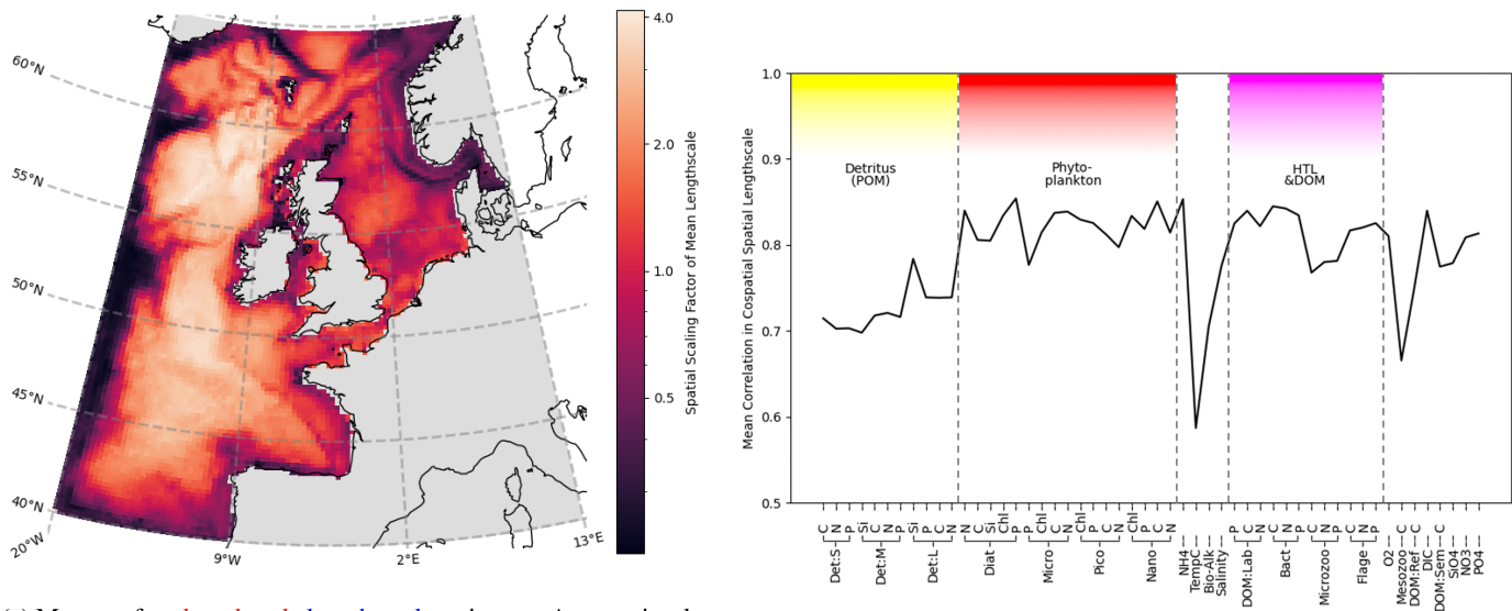
(a) Mean surface lengthscale-length-scale estimates. Average is taken over the full set of ERSEM variables. Correlation threshold is dynamically adjusted for each variable as described in Sect. 2.2.3. (b) Mean Pearson's correlation between co-spatial horizontal lengthscale-length-scales of each variable to every other variable.
