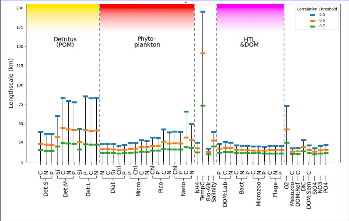
Figure 4. Estimate of mean horizontal length scales on length scales for each ERSEM variable on the shelf (as shown in Fig. 2 for diatoms chlorophyll with threshold 0.5) from 300 sample locations , using correlation metrics to determine distance at which mean correlation drops below thresholds of 0.5, 0.6 and 0.7.
