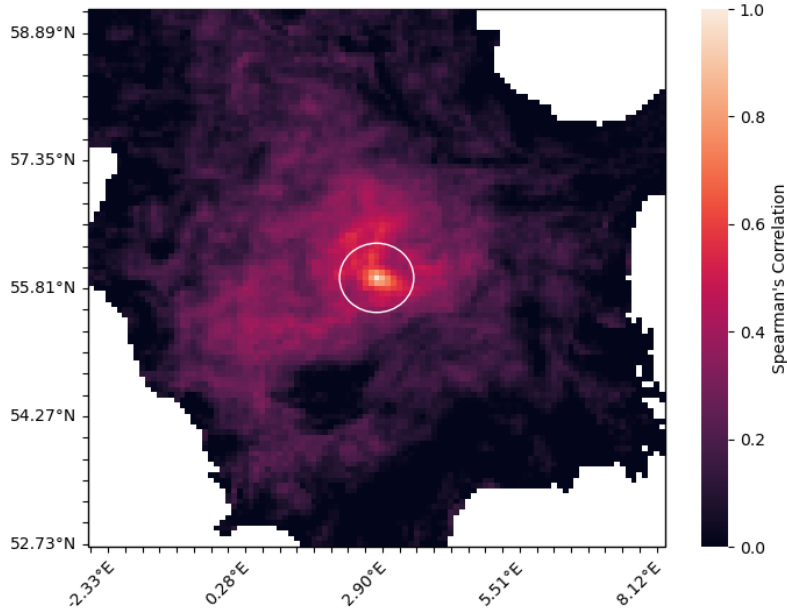
Figure 2. Lengthscale Horizontal length-scale estimate, \ell = 45.5 km shown as a white circle, calculated for Diat-Chl with correlation threshold set at 0.5, for the a reference point with coordinates 56.10^\circ N , 3.20^\circ E . The colours represent the simultaneous Spearman correlation of each grid point with the central grid point (which is of value 1, as it perfectly correlates with itself).
