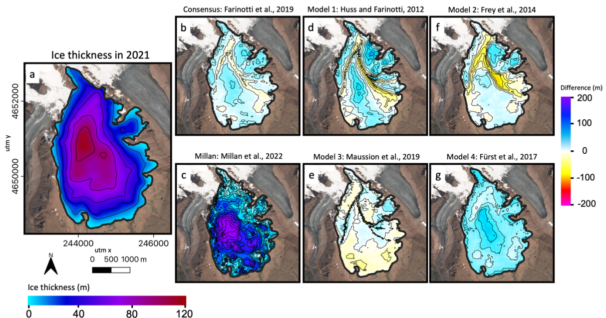
185 Figure 3: (a) Ice thickness of the Grigoriev ice cap in August 2021. The coordinate system corresponds to the EPSG:32644 WGS 84 / UTM zone 44N. (b-g) Difference between the created ice thickness distribution and the consensus estimate (b), the different models used to compile the consensus estimate (d,e,f,g) and the Millan dataset (c). The different ice thickness datasets are corrected to represent the state in 2021 for a proper comparison with our own reconstruction (panel a). The background of the seven panels is from Sentinel-2 in July 2021. Contours are added for every 20 m.
