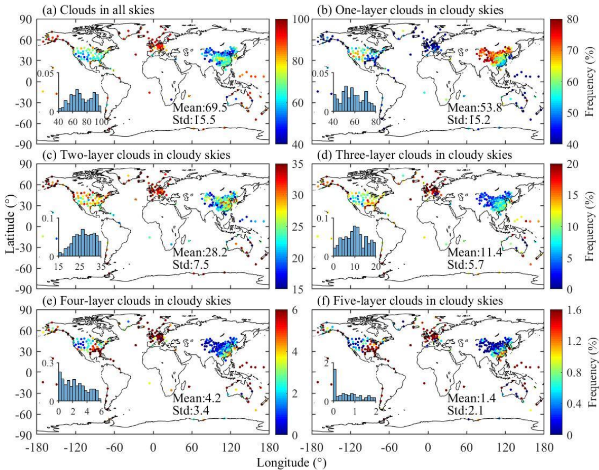
Figure 12. The geographic distributions of the occurrence frequencies of (a) clouds in all skies and (b–f) one-, two-, three-, four-, and five-layer clouds in cloudy skies at 1200 UTC during the period of 2018–2019. It should be noted that the range of the color bar differ a lot in order to improve the visual interpretation. Also shown are the histograms of probability distributions for the cloud occurrence frequencies in each panel.
