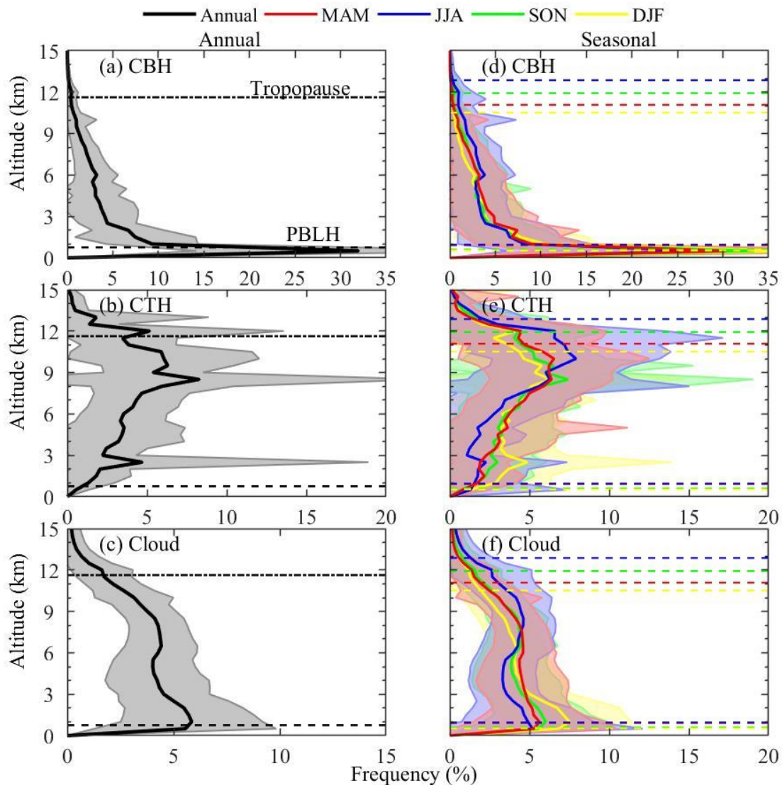
1115 Figure 8. Near-global mean vertical distributions of (a-c) annual and (d-f) seasonal occurrence frequencies of CBHs, CTHs, and clouds as detected by radiosonde data at 1200 UTC during the period of 2018–2019, respectively. The annual, MAM, JJA, SON, and DJF are marked in black, red, blue, green, and yellow, respectively. Samples are vertically divided with a resolution of 500 m. The percentage for a given altitude is defined as the ratio of cloudy samples on that altitude to all cloudy samples. The solid lines are the mean values and shadows are the one standard deviation at annual or a given season. The planetary boundary layer height (PBLH) 1120 is determined with the method proposed by Vogelezang and Holtslag (1996), marked in dot-hyphen, and the tropopause is defined with the method from WMO (1957), marked in hyphen. The determination of PBLH and tropopause are detailed in the Supplementary Information.
