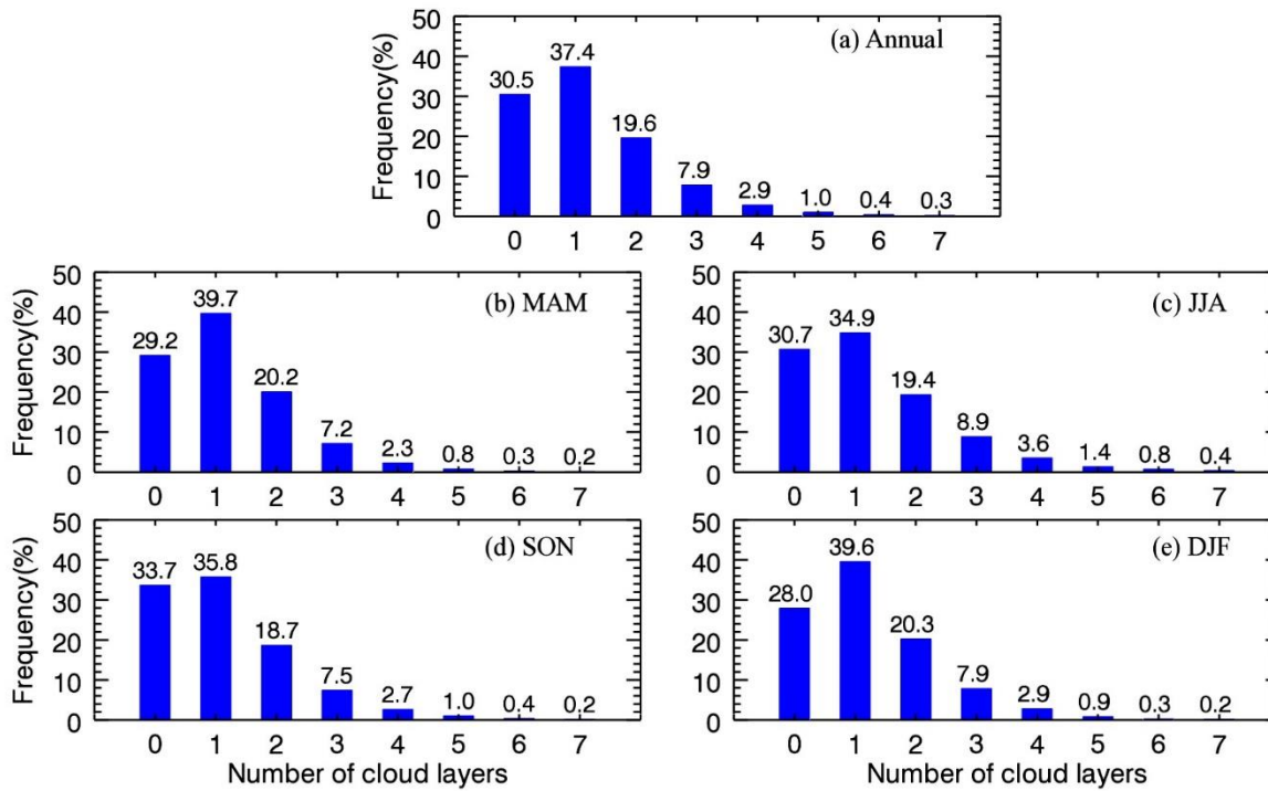
1105 Figure 6. Near-global mean occurrence frequencies of clouds with a variety of number of layers ranging from 0 to 7 as detected by high-resolution radiosonde measurements at 1200 UTC during the period of 2018–2019: (a) annual, (b) March–April–May (MAM), (c) June–July–August (JJA), (d) September–October–November (SON), and (e) December–January–February (DJF). Also marked is the probability for the specified cloud type at the top of each bar.
