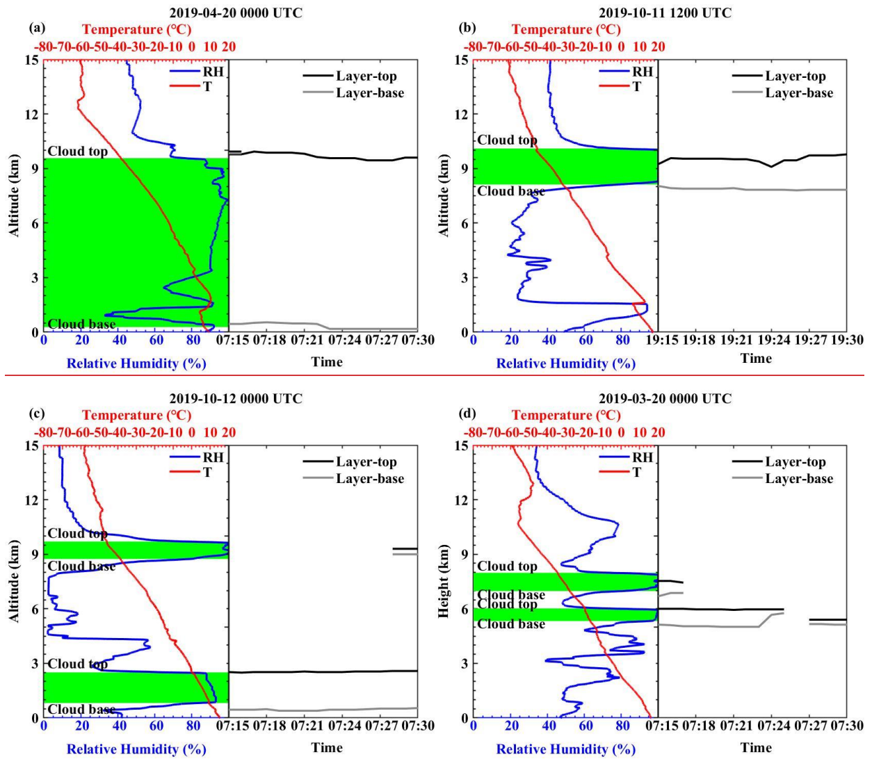
1085 Figure 3. Examples of the detection of CVS by (left) high-resolution radiosonde and (right) Ka-band millimeter wavelength cloud radar (MMCR) at Beijing site for the four selected cases, (a, b) one-layer clouds, and (c, d) two-layer clouds. Green shading represents the cloud layers retrieved from radiosonde. In each subfigure (left), the blue and red solid line represent the RH and T profile, respectively.
