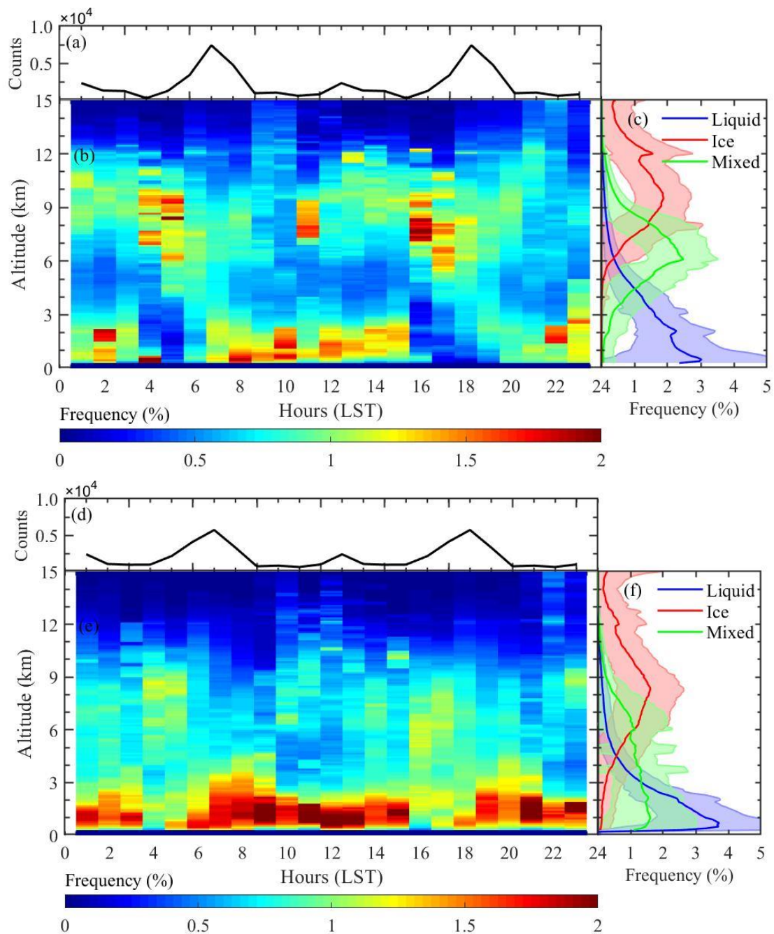
1150 Figure 14. Diurnal variations of all clouds and altitude-resolved clouds as detected by all radiosondes at 0000 and 1200 UTC in boreal summer (JJA, a) and b) and boreal winter (DJF, d) and e) during the period of 2018–2019. Also shown are the vertical probability distributions of liquid (in blue), ice (in red), and liquid-ice mixed (in green) clouds in boreal summer and boreal winter (c, f).
