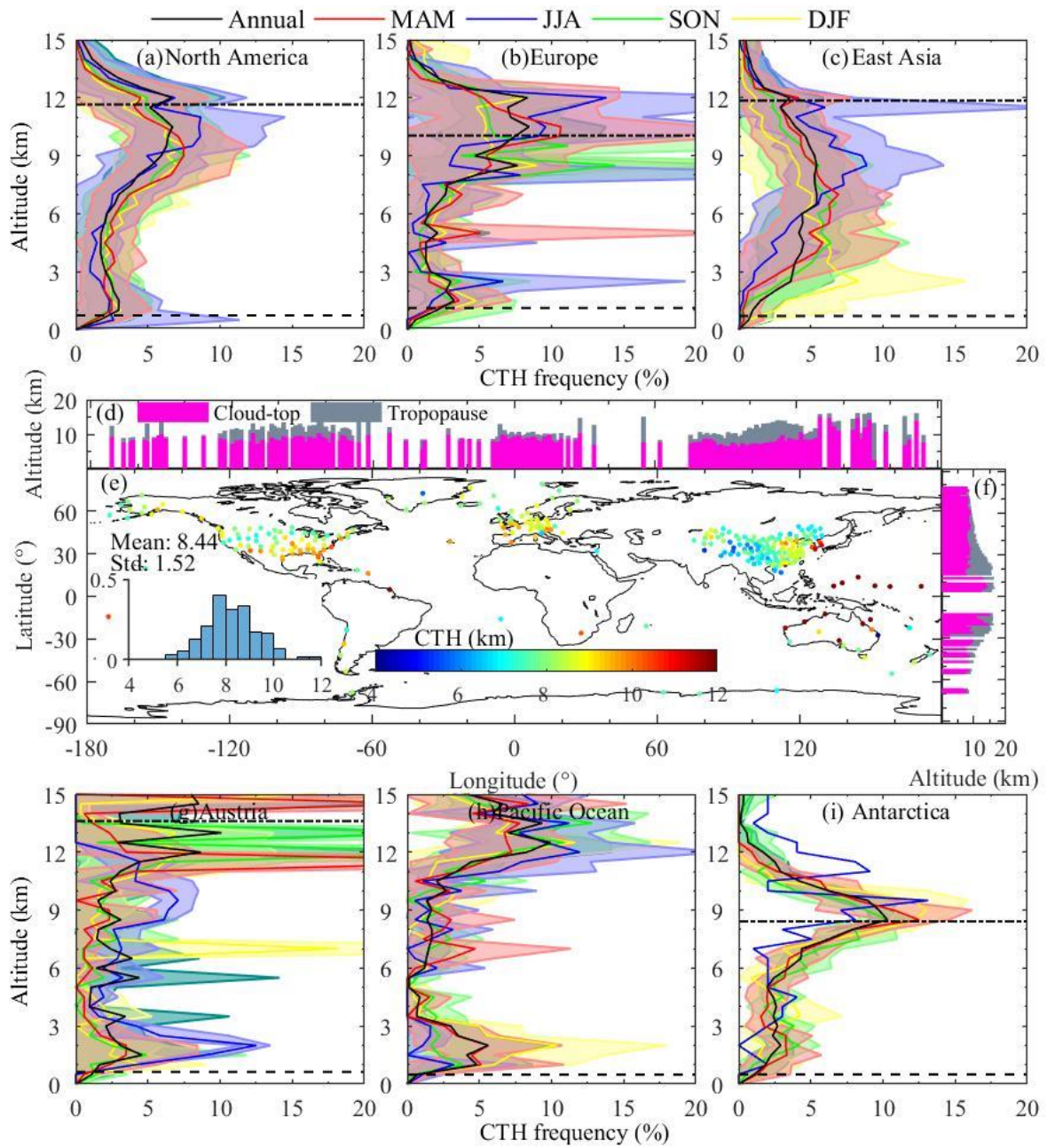
Figure 10. Similar as Figure 9, but for the occurrence frequencies of CTHs at 1200 UTC during the period of 2018–2019.
