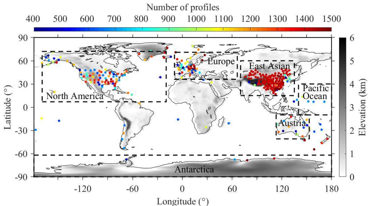
1065 Figure 1. Geographic distribution of the number of profiles (colored full circle) for the near-global high-resolution radiosonde observation stations from 2018 to 2019. Also shown is the elevation of each radiosonde site in grey-scale shading. Black rectangles denote observation coverages at six regions of interest (i.e., Europe, North America, East Asia, Austria, Pacific Ocean, and Antarctica). The numbers of radiosonde stations within Europe, North America, East Asia, Austria, Pacific Ocean, and Antarctica are 44, 150, 120, 13, 5, and 4, respectively. The numbers of radiosonde stations in the Northern Hemisphere (NH) and Southern 1070 Hemisphere (SH) are 338 and 36, respectively.
