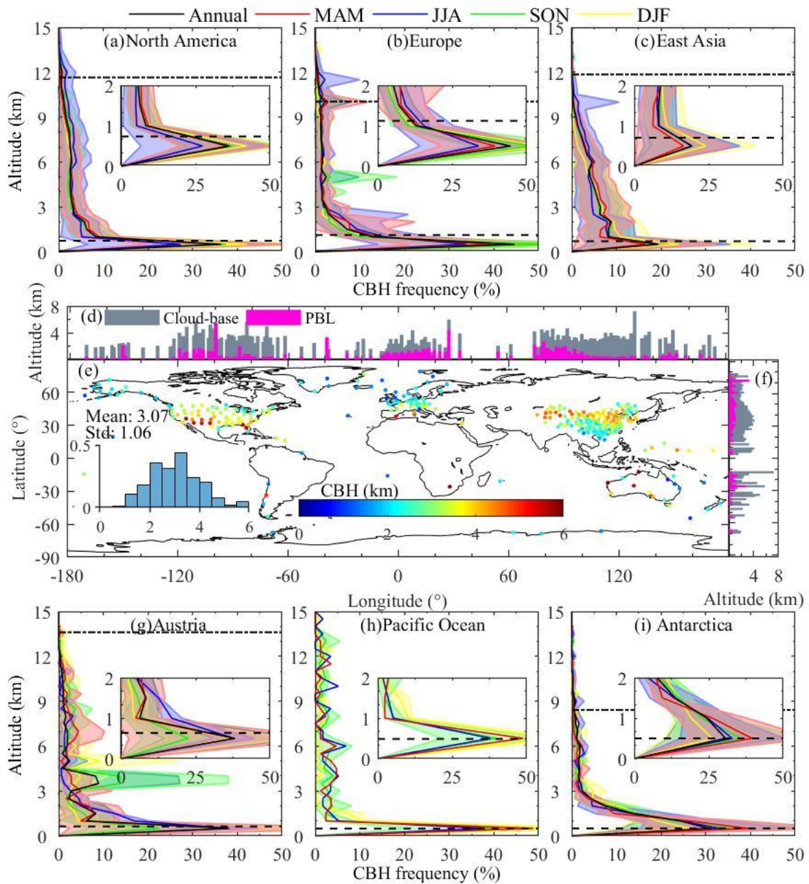
1125 Figure 9. Regional mean vertical distributions of the occurrence frequencies of CBHs at 1200 UTC during the period of 2018–2019. The altitude resolved annual and seasonal averaged occurrence frequencies of CBHs are displayed in (a-c, g-i) over six regions of interest, including North America, Europe, East Asia, Austria, Pacific Ocean, Antarctica. Also shown are the near-global geographic distribution of the annual mean CBH (e), with the histogram of the probability distribution for CBH in the inset and the corresponding meridional (d) and zonal (f) means overlaid with the mean PBLH.
