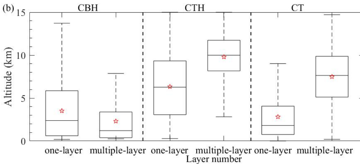
Figure 7. Near-global annual mean (a) vertical locations of one-, two-, three-, four-, and five-layer clouds and (b) boxplot of CVS (CBH, CTH, and CT) for one- and multi-layer clouds at 1200 UTC during the period of 2018–2019. The mean \pm one standard deviation values of CBH, CTH, and total CT for each cloud type are also marked in (a).
