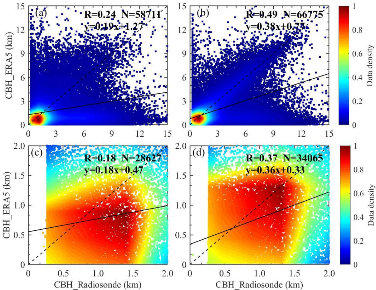
1100 Figure 5. Scatter plots of the comparisons of the radiosonde derived CBHs with those from ERA5 for all the data at (a) 0000 and (b) 1200 UTC, and for the cases that both CBHs are less than 2.0 km at (c) 0000 and (d) 1200 UTC during the period of 2018–2019. Each point represents one measurement at 0000 or 1200 UTC. R represents the correlate coefficient and N represents the sample number. The linear regression equation is also given, and the regression line is marked in black solid line. The dash black line is 1:1 line.
