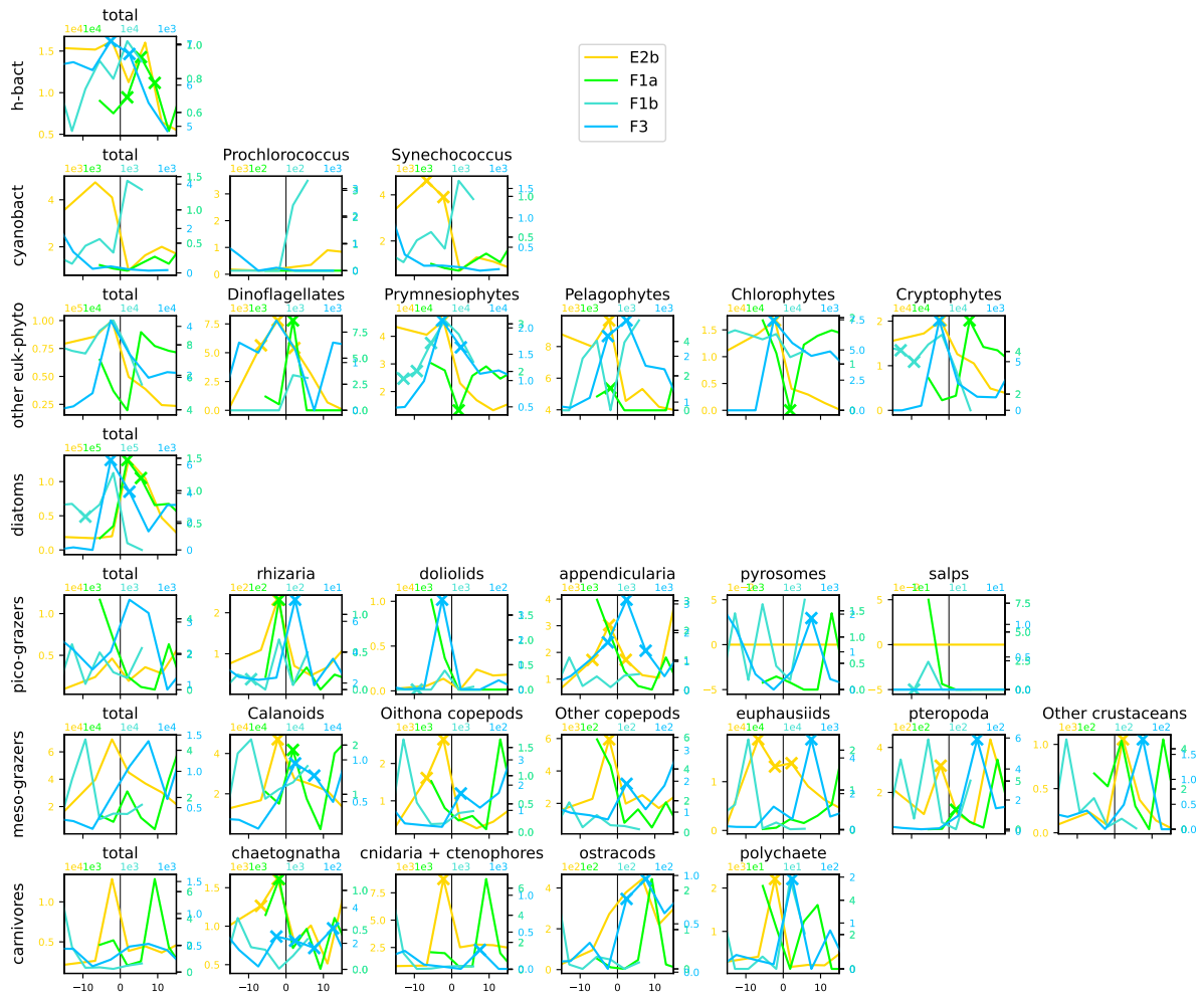
Figure A12. Distribution across fronts E2b, F1a, F1b and F3 of the total biomass ( \mu\text{gCm}^{-3} ) of each trophic group (left column) and biomass of the individual taxa constituting it. The data are centered on the physical density gradient (vertical black lines), the crosses indicate the stations with a biomass peak. The x-axis is in km, with 0 at the center of the front.
