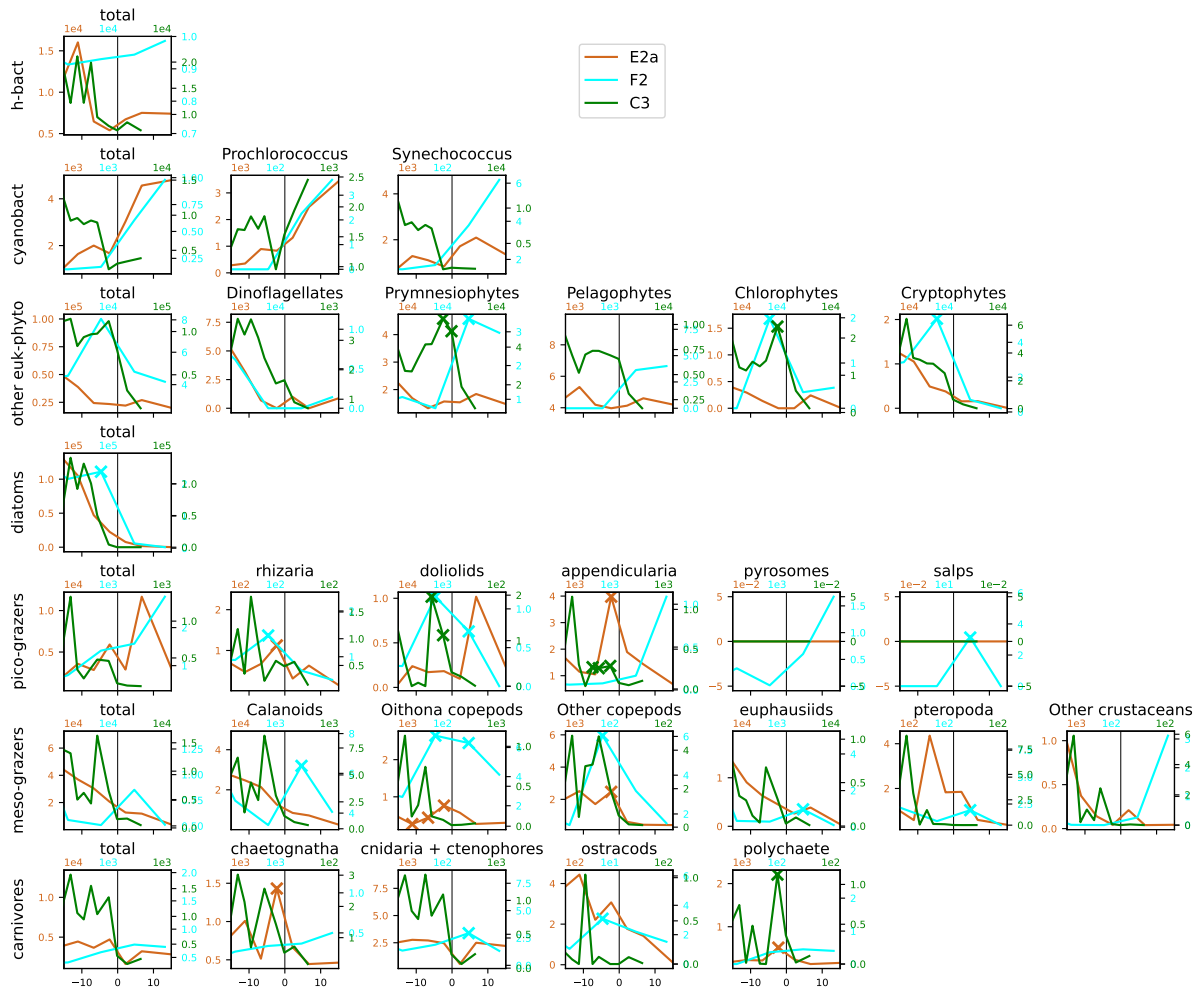
Figure A13. Distribution across fronts E2a, F2 and C3 of the total biomass ( \mu\text{gCm}^{-3} ) of each trophic group (left column) and biomass of the individual taxa constituting it. The data are centered on the physical density gradient (vertical black lines), the crosses indicate the stations with a biomass peak. The x-axis is in km, with 0 at the center of the front.
