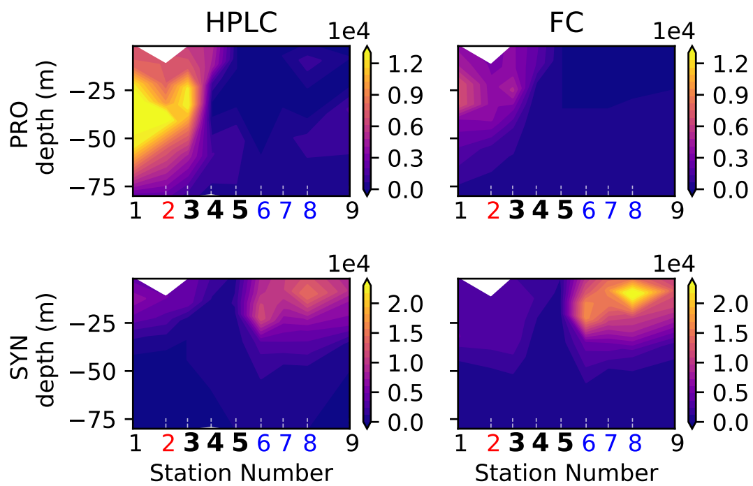
Figure A6. Biomass ( \mu\text{gC m}^{-3} ) of cyanobacteria ( Prochlorococcus on the top row, Synechococcus on the bottom row) in the A-front transect measured by two different instruments : HPLC (left row) and Flow Cytometry (FC, right row). The numbers of the frontal stations are written in bold and the warm and cold sides in red and blue.
