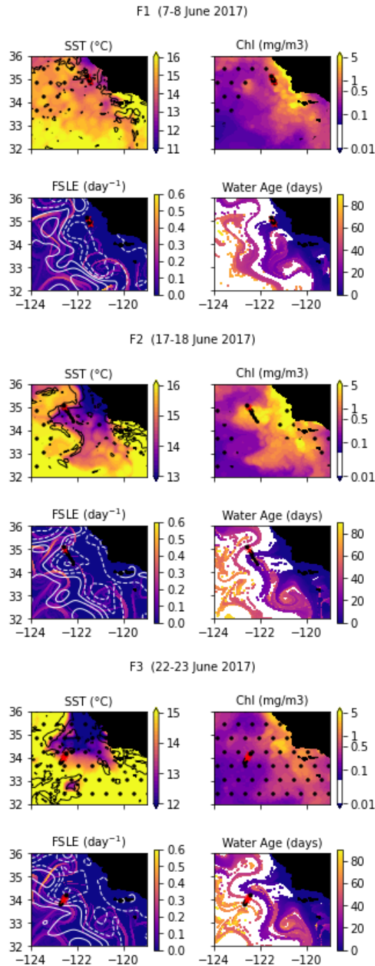
Figure A4. Snapshots of satellite-derived data at the time of transects F1, F2 and F3 : SST (black lines indicate SST fronts ( HI > 10 )), chlorophyll, FSLE ( \text{day}^{-1} , with SSH in white contours at 0,0.05,0.1,0.15,0.2,0.25,0.3 m above geoid; dashed lines indicate cyclonic eddies and solid lines anticyclonic eddies) and water age (in days since the water parcel left the coast). The hatches indicate the presence of clouds, where the fields are smoothed by the interpolation (resulting in weaker gradients). The position of the transect is indicated with red crosses for frontal stations and small black dots for background stations. 27
