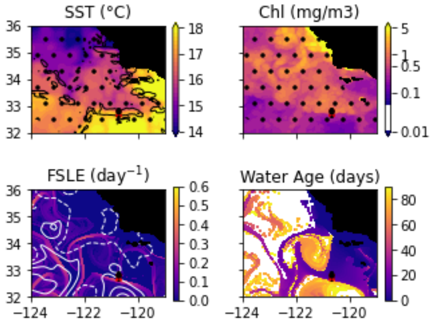
Figure A1. Snapshots of satellite-derived data at the time of transect A : SST (black lines indicate SST fronts ( HI > 10 )), chlorophyll, FSLE ( \text{day}^{-1} , with SSH in white contours at 0,0.05,0.1,0.15,0.2,0.25,0.3 m above geoid; dashed lines indicate cyclonic eddies and solid lines anticyclonic eddies) and water age (in days since the water parcel left the coast). The hatches indicate the presence of clouds, where the fields are smoothed by the interpolation (resulting in weaker gradients). The position of the transect is indicated with red crosses for frontal stations and small black dots for background stations.
