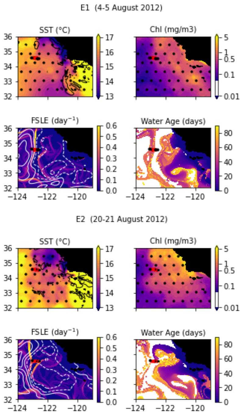
Figure A3. Snapshots of satellite-derived data at the time of transects E1 and E2 : SST (black lines indicate SST fronts ( HI > 10 )), chlorophyll, FSLE ( \text{day}^{-1} , with SSH in white contours at 0,0.05,0.1,0.15,0.2,0.25,0.3 m above geoid; dashed lines indicate cyclonic eddies and solid lines anticyclonic eddies) and water age (in days since the water parcel left the coast). The hatches indicate the presence of clouds, where the fields are smoothed by the interpolation (resulting in weaker gradients). The position of the transect is indicated with red crosses for frontal stations and small black dots for background stations.
