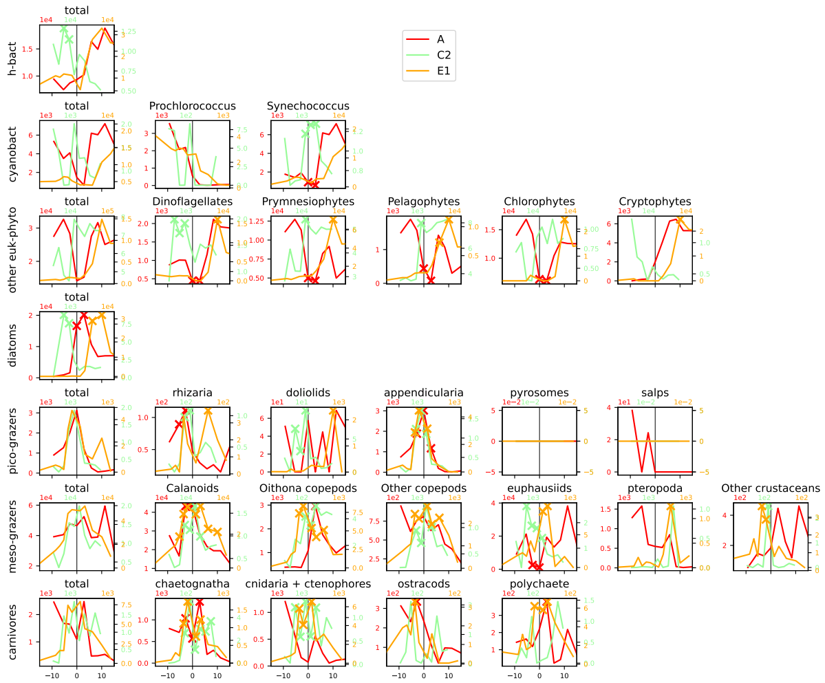
Figure A11. Distribution across fronts A, C2 and E1 of the total biomass ( \mu\text{gC m}^{-3} ) of each trophic group (left column) and biomass of the individual taxa constituting it. The data are centered on the physical density gradient (vertical black lines), the crosses indicate the stations with a biomass peak. The x-axis is in km, with 0 at the center of the front.
