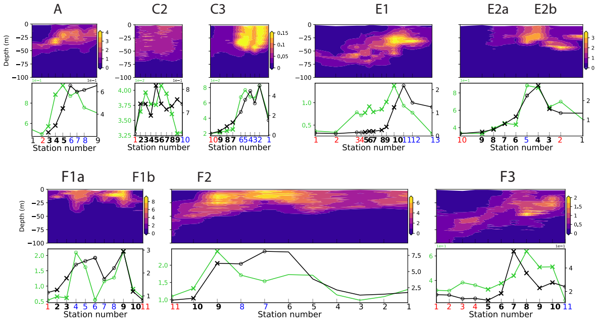
Figure A5. Top row : vertical sections of fluorescence (V). Bottom row : vertically integrated fluorescence (0-100 m) and HPLC-derived surface Chl-a ( \mu\text{gChl} - \text{am}^{-3} ). Front stations are indicated by crosses and the background stations by circles; the numbers of the frontal stations are written in bold and the warm and cold sides in red and blue.
