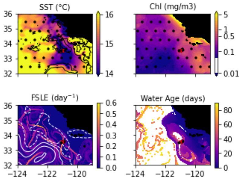
Figure A2. Snapshots of satellite-derived data at the time of transects C2 and C3 : SST (black lines indicate SST fronts ( HI > 10 )), chlorophyll, FSLE ( \text{day}^{-1} , with SSH in white contours at 0,0.05,0.1,0.15,0.2,0.25,0.3 m above geoid; dashed lines indicate cyclonic eddies and solid lines anticyclonic eddies) and water age (in days since the water parcel left the coast). The hatches indicate the presence of clouds, where the fields are smoothed by the interpolation (resulting in weaker gradients). The position of the transect is indicated with red crosses for frontal stations and small black dots for background stations.
