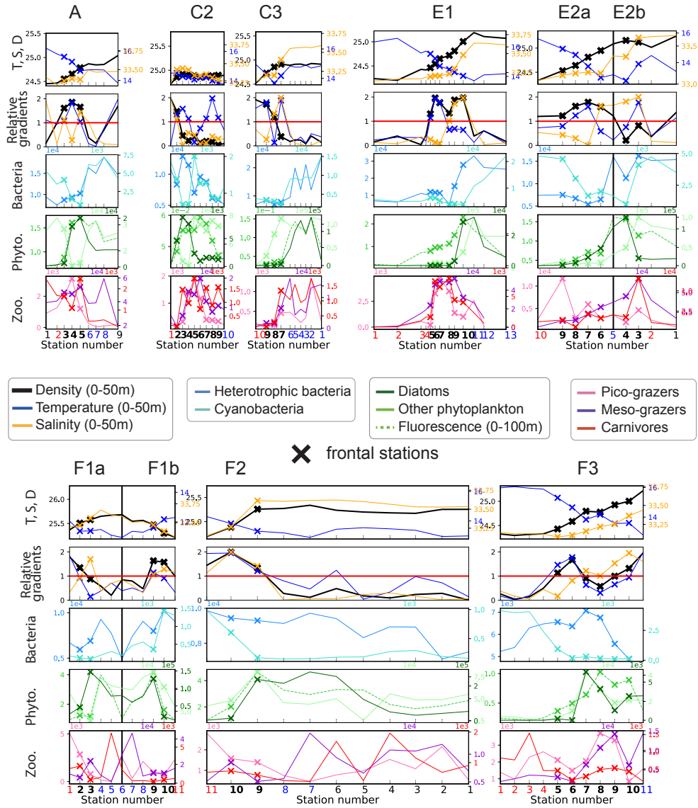
Figure 4. Distribution First row : distribution of density ( \text{kg m}^{-3} ), temperature ( ^{\circ}\text{C} ) and salinity (first row PSU); second row : density, temperature and salinity relative gradients( second row ); third, fourth and the fifth rows : biomass ( \mu\text{gC m}^{-3} ) of the seven plankton groups and fluorescence( third, fourth and fifth rows ), along the 8 transects. Frontal stations are represented with crosses; and the station number is written at the bottom of each panel in bold for frontal stations, red for warm background stations and blue for cold background stations. The center of the filaments in transects E2 and F1 is indicated with a black vertical line. The relative gradient threshold used to define frontal stations is indicated with a red horizontal line. The same scale is used along the x-axis for all transects. The same grid-spacing is used along the y-axis for density, temperature, salinity across all transects; and different scales are used for biomass.
