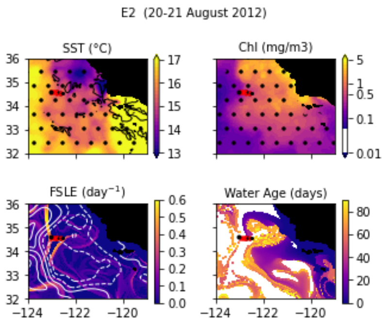
Figure A3. Snapshots of satellite-derived data at the time of transects E1 and E2 : SST (black lines indicate SST fronts ( HI > 10 )), chlorophyll, FSLE ( \text{day}^{-1} , with SSH in white contours at 0,0.05,0.1,0.15,0.2,0.25,0.3 m above geoid; dashed lines indicate cyclonic eddies and solid lines anticyclonic eddies) and water age (in days since the water parcel left the coast). The hatches indicate the presence of clouds, where the fields are smoothed by the interpolation (resulting in weaker gradients). The position of the transect is indicated with red crosses for frontal stations and small black dots for background stations.
