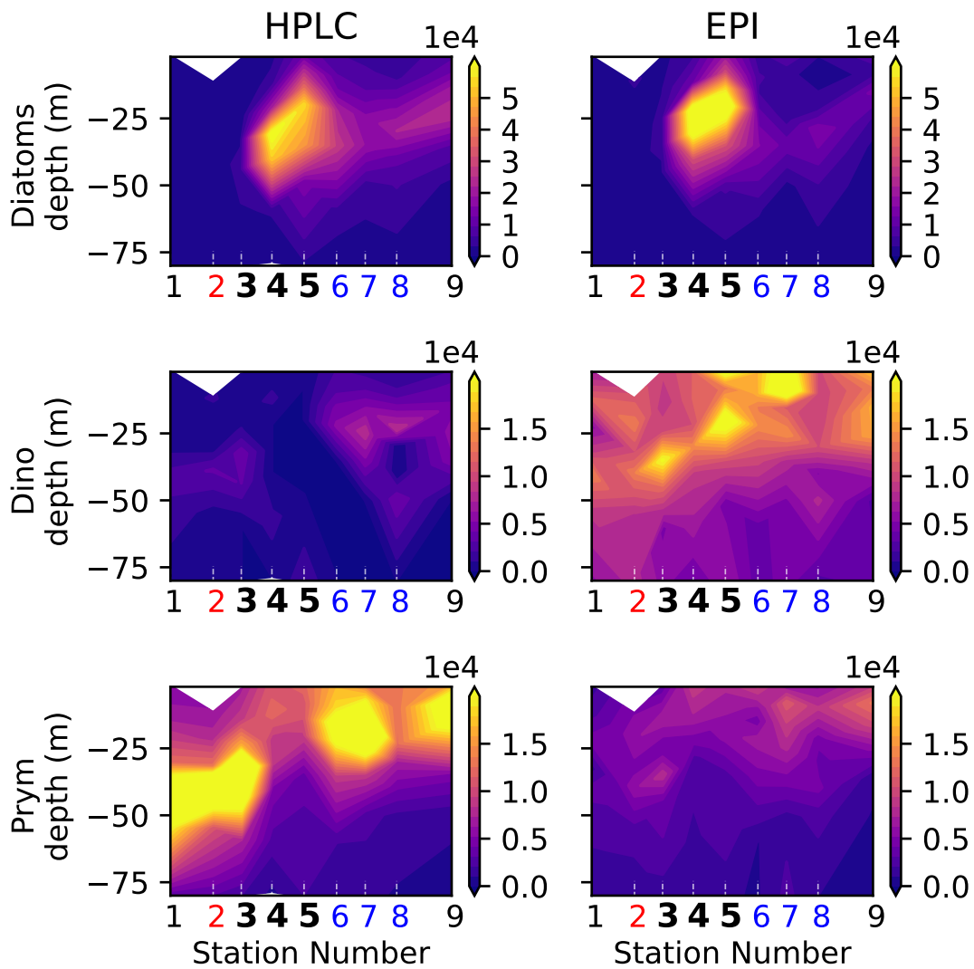
Figure A8. Biomass ( \mu\text{gCm}^{-3} ) of eukaryotic phytoplankton (Diatoms, Dinoflagellates and Prymnesiophytes) determined by HPLC (this study) and Epifluorescence microscopy ( from see Taylor et al. (2012) )
