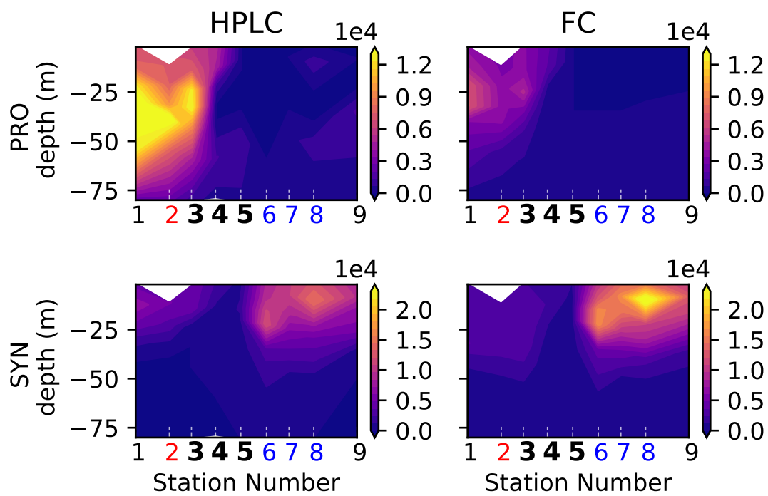
Figure A6. Biomass ( \mu\text{gC m}^{-3} ) of cyanobacteria ( Prochlorococcus on the left-top row , Synechococcus on the right-bottom row ) in the A-front transect measured by two different instruments : HPLC ( top-left row ) and Flow Cytometry ( bottom-FC, right row ). The numbers of the frontal stations are written in bold and the warm and cold sides in red and blue.
