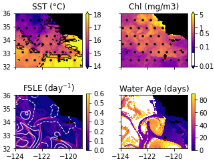
Figure A1. Snapshots of satellite-derived data at the time of transect A : SST (black lines indicate SST fronts ( HI > 10 )), chlorophyll, FSLE ( \text{day}^{-1} , with SSH in white contours at 0, 0.05, 0.1, 0.15, 0.2, 0.25, 0.3 m above geoid; dashed lines indicate cyclonic eddies and solid lines anticyclonic eddies) and water age (in days since the water parcel left the coast). The hatches indicate the presence of clouds, where the fields are smoothed by the interpolation (resulting in weaker gradients). The position of the transect is indicated with red crosses for frontal stations and small black dots for background stations.
