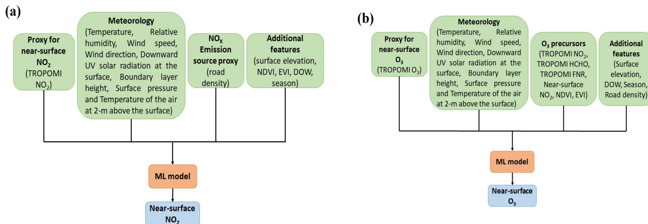
Figure 2. Predictor variables and data flow for the NO 2 (a) and O 3 (b) ML model.
