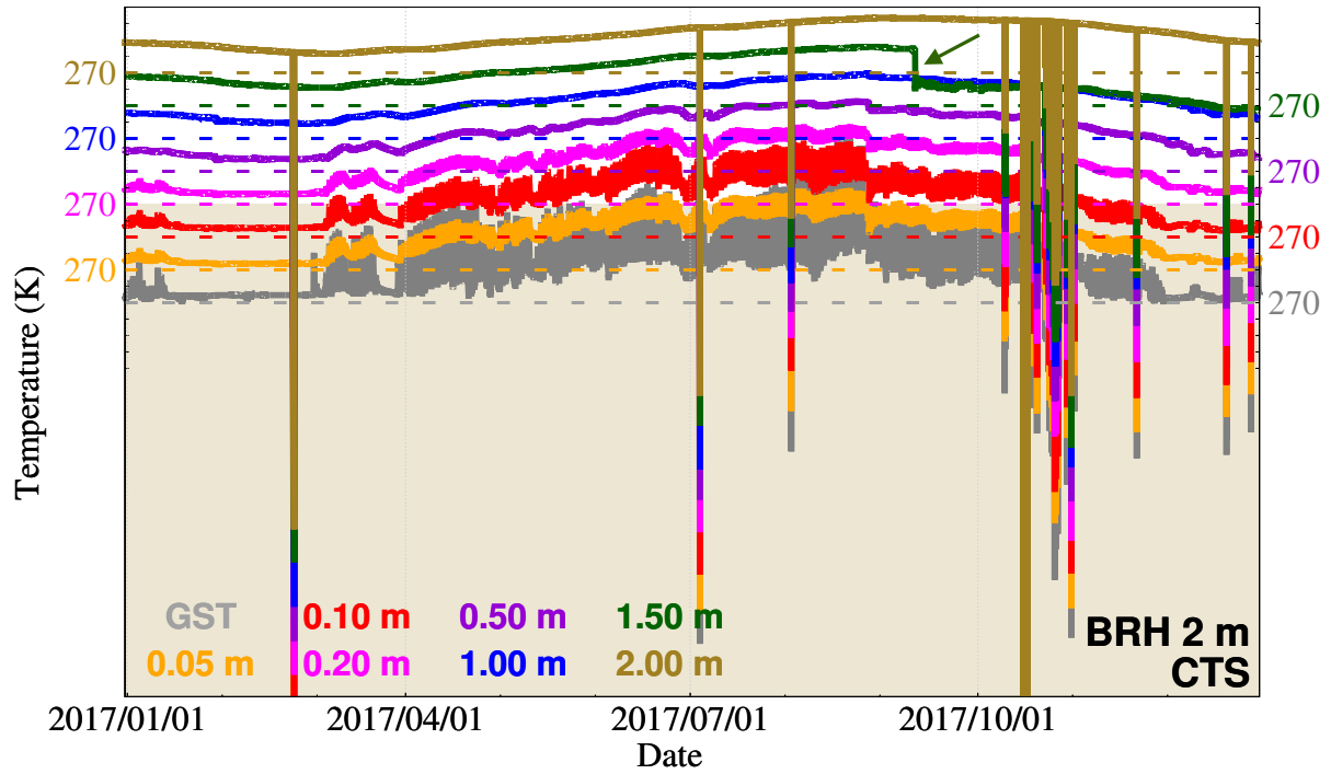
Figure 3. Example of errors in BRH 2 m at CTS in the year 2017. The 10-minute GST observations (grey) and those of temperatures for seven levels below the surface are shown. Time series are shifted an offset equivalent to 10 K and ticks are included every 5 K for clearer visualization. The value of 270 K is shown for all levels as a reference. The olive color band at the bottom represents the level of 230 K for the 2 m depth temperature time series, used to determine nonphysical values. The segment of the level of 1.5 m pointed by the arrow indicates a shift in the mean temperature value. Time values after the shift are subsequently eliminated.
