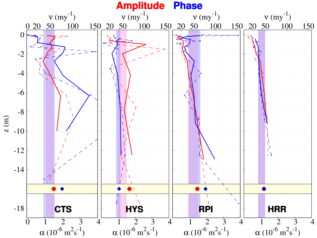
Figure 9. Thermal diffusivity ( \alpha , 10^{-6} \text{ m}^2 \text{ s}^{-1} ) and wave velocity ( \nu , \text{m yr}^{-1} ) profiles with depth (m). The red curves were obtained from normalized amplitude attenuation values \ln(A/A_0) and the blue ones from phase shift values with depth. Dashed (solid) lines represent the raw (3-running layer thickness-weighted average) estimate. Points at the bottom of the profile (shaded yellow) represent the thickness-weighted average of the whole subsurface profile. Shaded areas in red (blue) represent the thermal diffusivity values obtained by linearly fitting amplitude attenuation (phase shift) in Fig. 7.
