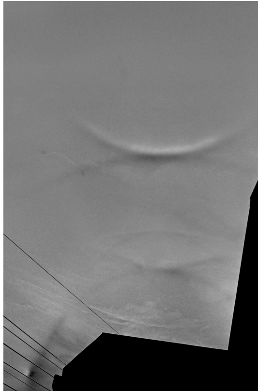
Figure 10. Processed with sky-color regression: In the original image (see Fig. 6), even experienced observers can hardly detect halos except for a parheliion, a circumzenithal arc, and a part of the 22° halo and the upper tangent arc.
