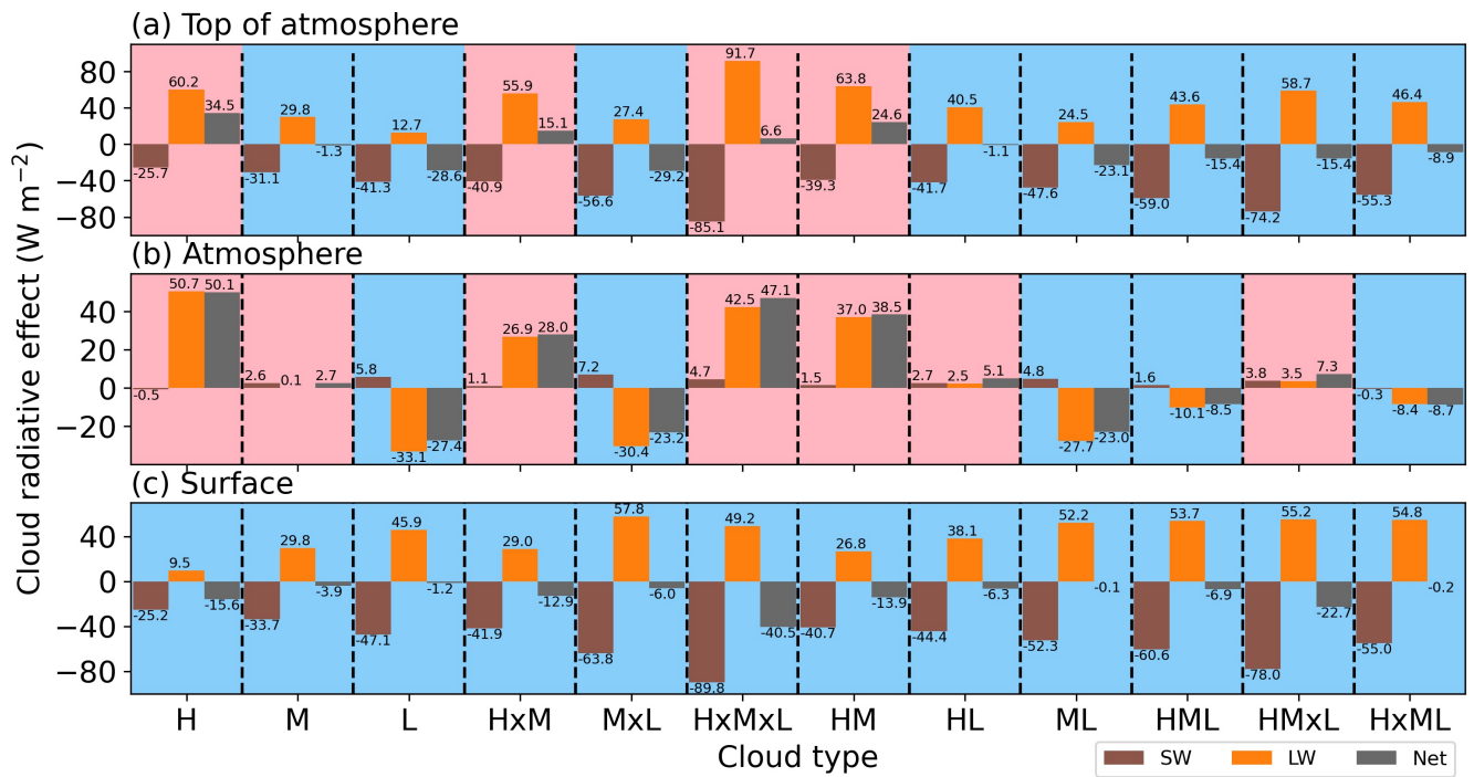
Figure 6: The 4-year (2007–2010) global average SW, LW and net CREs of the 12 CVSs (a) at TOA, (b) within the atmosphere and (c) at the surface. The blue and red backgrounds in each sub-box indicate cooling and warming effects, respectively.
