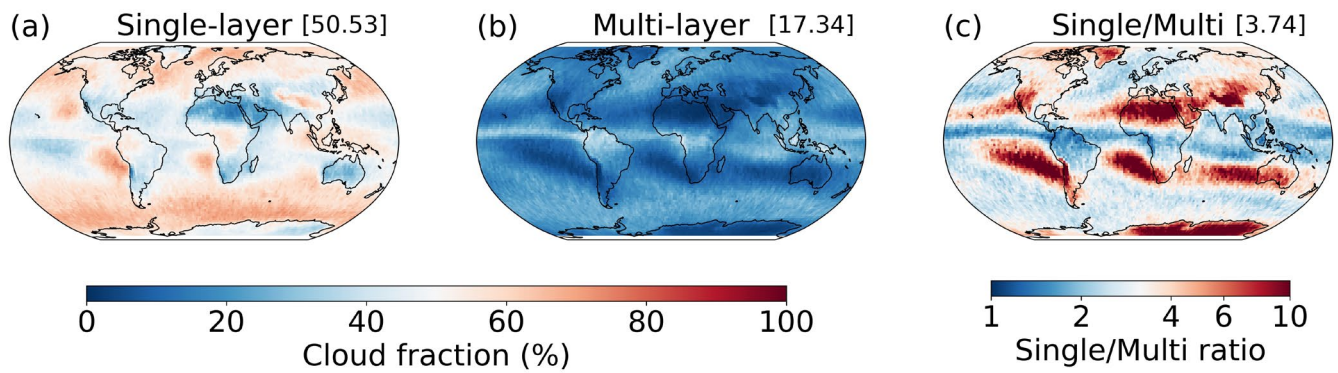
Figure 3: Spatial distributions of the 4-year (2007–2010) average (a) single-layer cloud fraction, (b) multi-layer cloud fraction, and (c) the ratio of time-average single-layer cloud fraction to the multi-layer cloud fraction. The value above each subfigure denotes the area-weighted global, four 4-year average.
