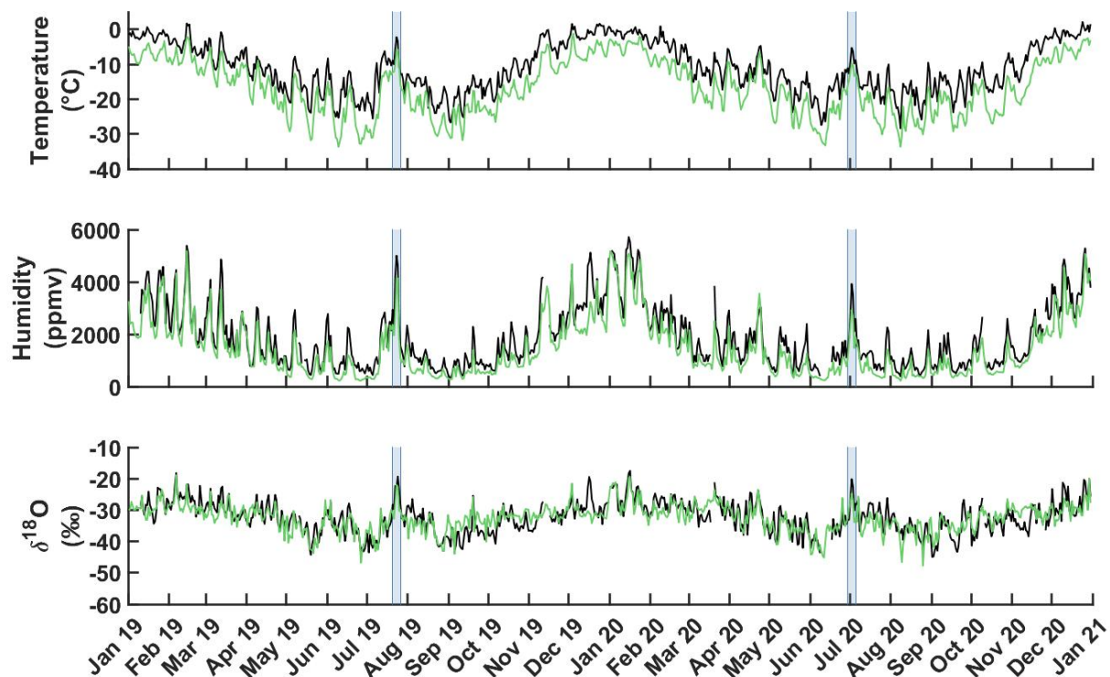
Figure 5. Comparison of temperature, humidity and \delta^{18}\text{O} modeled by ECHAM6-woiso and measured at DDU station over the period 2019-2020. Meteorological and isotopic measurements at DDU at daily resolution are shown in black. Panels from top to bottom: 1) 2m-temperature ( ^{\circ}\text{C} ) from Meteo France weather station, 2) humidity (ppmv) measured by the Picarro laser spectrometer; 3) water vapor \delta^{18}\text{O} ( \text{‰} ). Green lines correspond to the ECHAM6-woiso combination of surface air level outputs (daily resolution) using configuration c (see text). Light blue bars indicate major winter synoptics events of 23 July 2019 and 2 July 2020 (see text).
