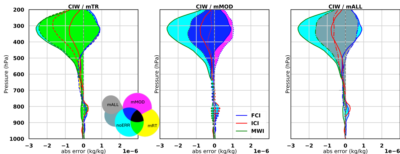
Figure 5. Differences of STD between the combined retrievals and the single instrument retrievals are displayed, blue for FCI, red for ICI and green for MWI. The full lines correspond to the noERR experiments and are the same on the three panels. Then in addition, the mEXP curves are displayed as discontinuous lines: dashed line for mRT (left panel), dotted line for mMOD (middle panel) and dash-dotted line for mALL (right panel). The few large dots represent non-significant differences and can be found in lower layers. The left panel displays together noERR and mRT, the middle panel displays together noERR and mMOD, and the right panel displays together noERR and mALL. Colored areas highlight the differences between full and discontinuous curves. When they are not overlaid, only baseline colors appear (cyan for noERR, yellow for mRT, magenta for mMOD) and this means the perturbation has an impact on the synergy. When they are overlaid, only mixed colors appear (green, blue, dark blue) and this means the perturbation has little impact on the synergy.
