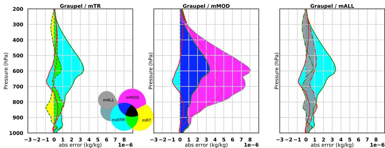
Figure 9. Same as figure 5 for graupel retrievals
