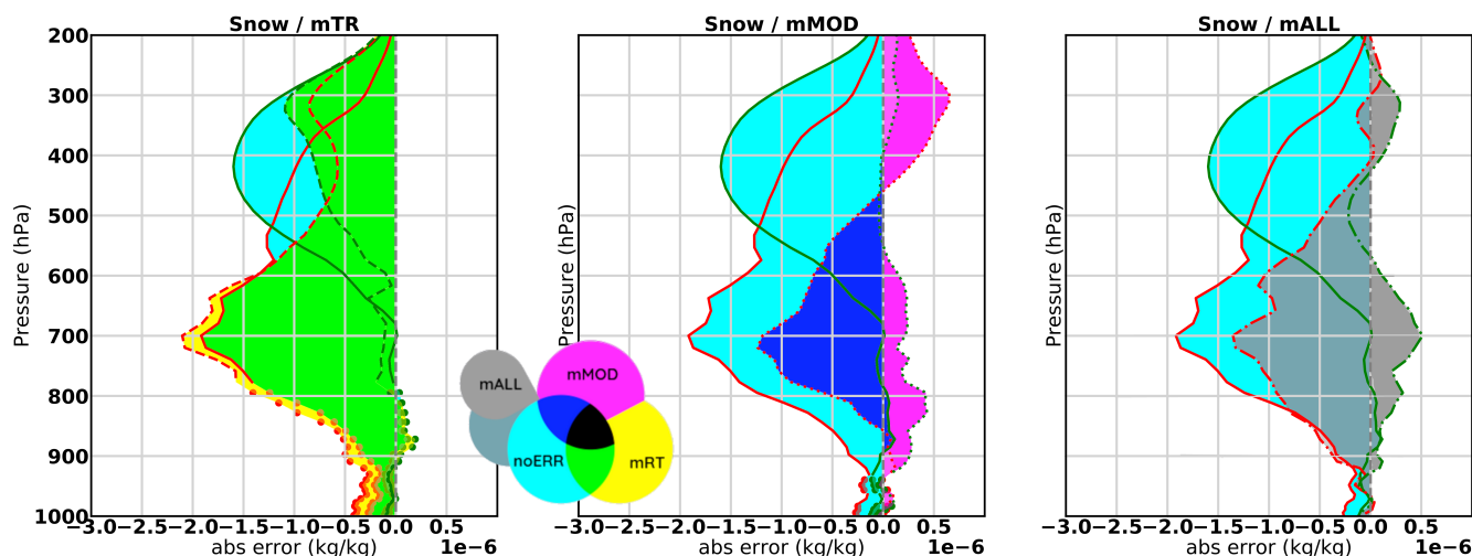
Figure 7. Same as figure 5 for snow retrievals
