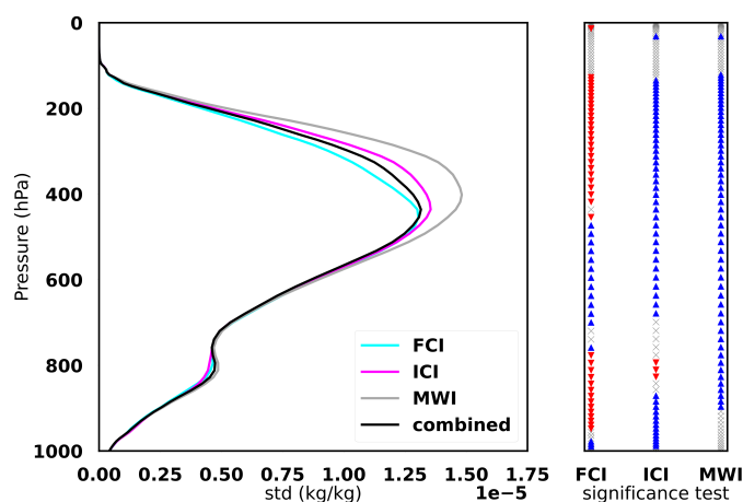
Figure 4. On the left, standard deviation of inversion error for CIW as function of pressure (hPa). On the right, Levene's significance test of differences between std of combined and each single instrument. The cyan curve corresponds to the retrieval with FCI only, the magenta curve with ICI only, the grey curve with MWI only, the black curve is the combined retrieval. Blue (resp. Red) arrows indicate a significant improvement (resp. degradation) due to the combination of the three instruments. Grey crosses indicate a non-significant difference.
