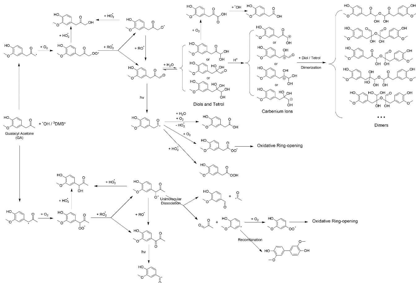
250 Scheme 2. Postulated aqueous-phase reaction pathways triggered by the ketone functional group of GA.
