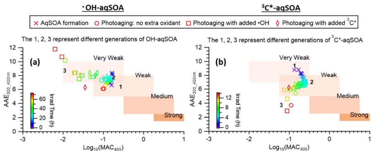
Figure 8. The light absorption properties of (a) •OH-aqSOA and (b) ³C*-aqSOA as shown in the AAE vs. log 10 (MAC 405 ) space. The shaded areas in each plot represent very weakly, weakly, moderately, and strongly absorbing BrC denoted based on the optical-based BrC classification scheme (Saleh, 2020; Zhai et al., 2022). The numbers 1, 2, and 3 represent the different generations of the •OH-aqSOA and the ³C*-aqSOA products obtained from PMF.
