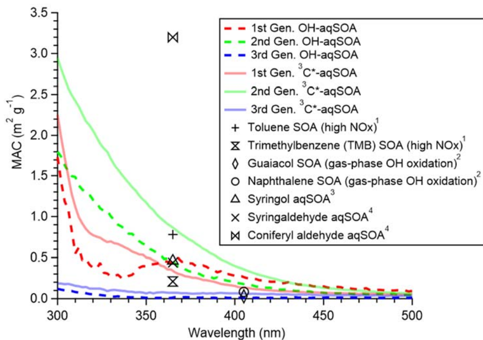
375 Figure 9. Mass absorption coefficient spectra of the PMF resolved three generations of the OH-aqSOA and the ^3\text{C}^* -aqSOA, comparing with previously reported MAC values of SOA produced from aromatic precursors by 1 Liu et al., 2016, 2 Lambe et al., 2013, 3 Yu et al., 2014 and 4 Smith et al., 2016.
