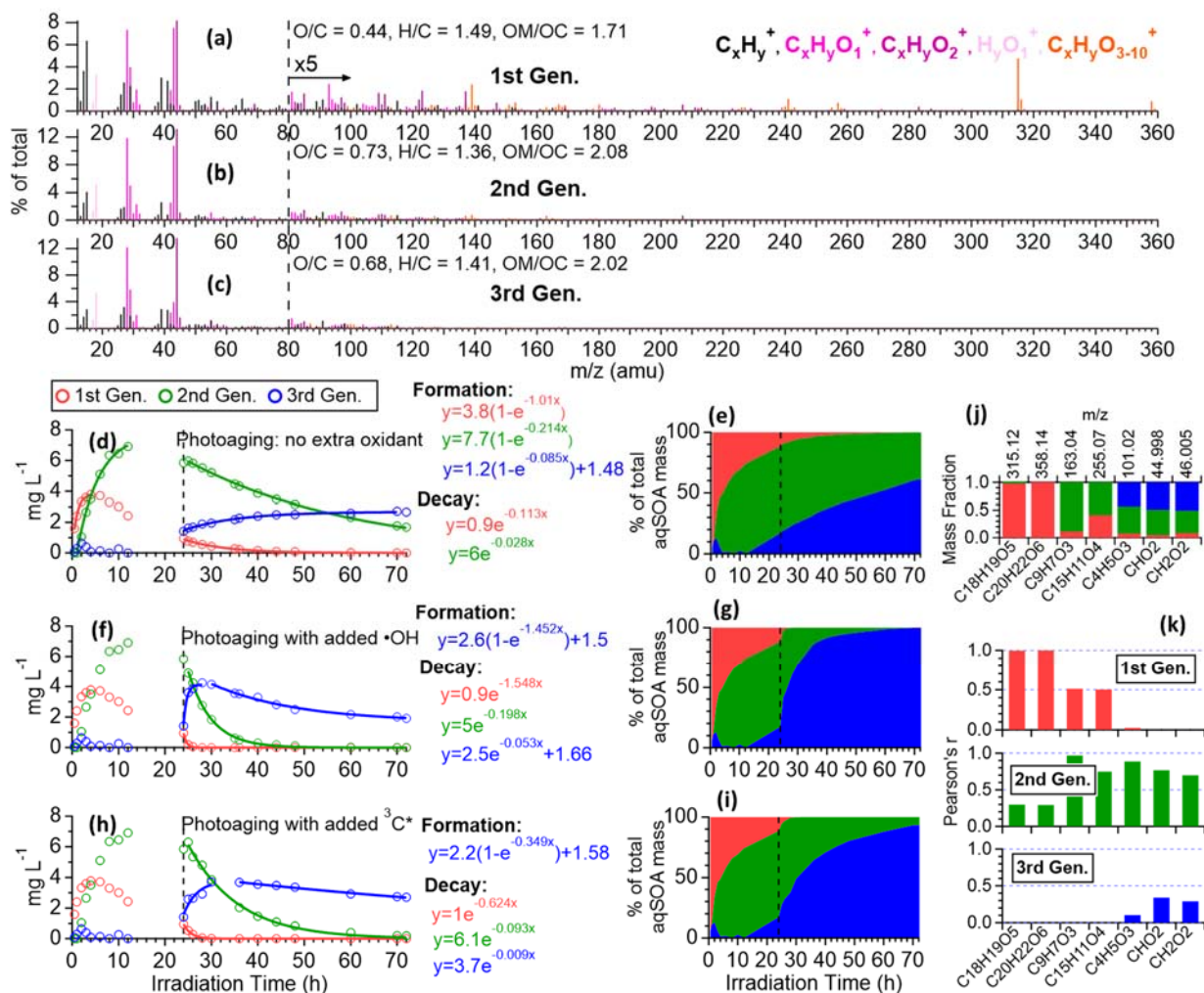
315 Figure 6. Characteristics of the three generations of the \bullet\text{OH} -aqSOA products resolved by PMF: (a-c) MS profiles; (d, f, and h) mass concentration time series; and (e, g, and i) fractional contribution time series of the PMF factors. (j) Mass fraction of selected AMS tracer ions attributed to each PMF factor. (k) Correlation between PMF factors and selected AMS tracer ions.
