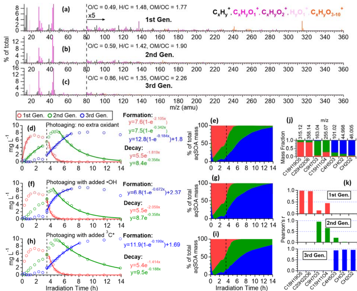
320 Figure 7. Characteristics of the three generations of the ^{13}\text{C}^* -aqSOA products resolved by PMF: (a-c) MS profiles; (d, f, and h) mass concentration time series; and (e, g, and i) fractional contribution time series of the PMF factors. (j) Mass fraction of selected AMS tracer ions attributed to each PMF factor. (k) Correlation between PMF factors and selected AMS tracer ions.
