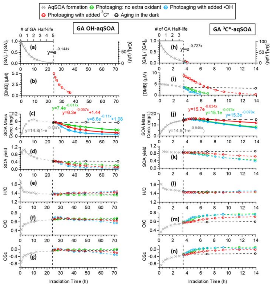
190 Figure 1. Overview of aqSOA formation and aging in •OH- and ^3\text{C}^* -initiated photoreactions of GA. Decay of (a & h) GA and (b & i) 3,4-DMB in the solution. Trends of aqSOA (c & j) mass concentration and (d & k) mass yield and (e & l) H/C, (f & m) O/C and (g & n) OSC determined by HR-ToF-AMS. These measured values are also shown in Tables S1 and S2.
