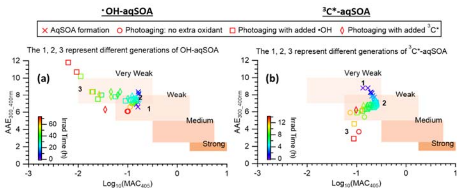
Figure 8. The light absorption properties of (a) •OH-aqSOA and (b) ³C*-aqSOA as shown in the AAE vs. \log_{10}(\text{MAC}_{405}) space. The shaded areas in each plot represent very weakly, weakly, moderately, and strongly absorbing BrC denoted based on the optical-based BrC classification scheme (Saleh, 2020; Zhai et al., 2022). The numbers 1, 2, and 3 represent the different generations of the •OH-aqSOA and the ³C*-aqSOA products obtained from PMF.
