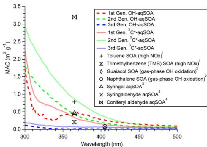
Figure 9. Mass absorption coefficient spectra of the PMF resolved three generations of the OH-aqSOA and the 3 C*-aqSOA, comparing with previously reported MAC values of SOA produced from aromatic precursors by 1 Liu et al., 2016, 2 Lambe et al., 2013, 3 Yu et al., 2014 and 4 Smith et al., 2016.
