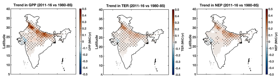
Figure 6: The spatial trend in fluxes from spring wheat. The stippling shows the grid cells where the trend is significant at 95%.
