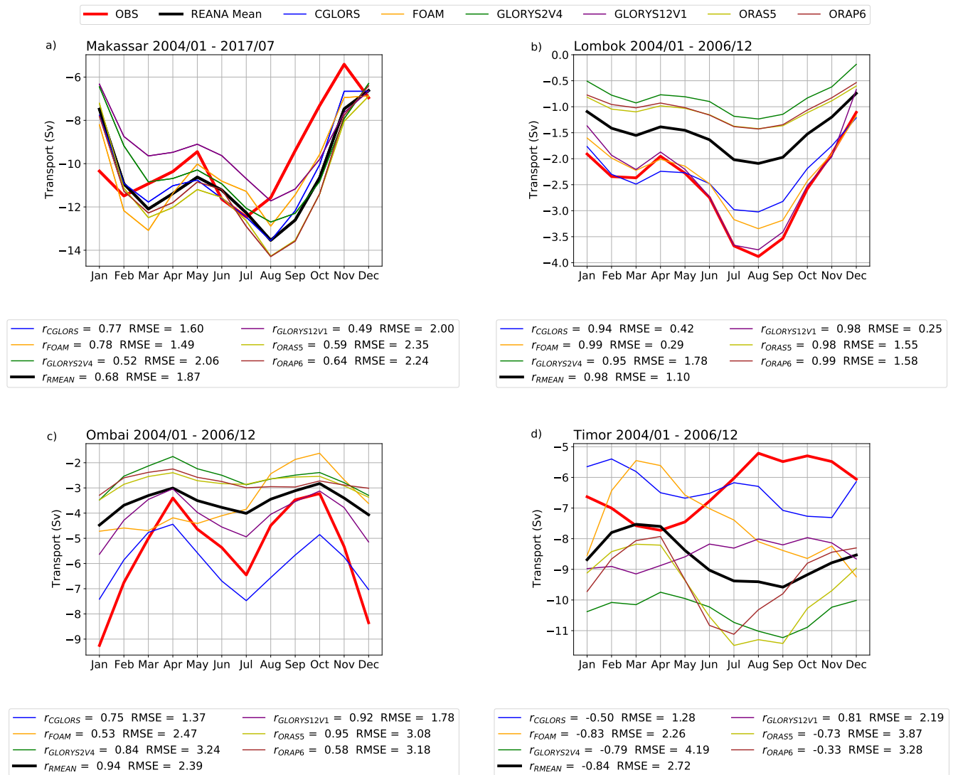
Figure 6. Mean annual cycle of ITF transport in a) Makassar Strait, b) Lombok Strait, c) Ombai Strait, and d) Timor Passage as represented by observations and reanalyses. Subjacent boxes display corresponding Pearson correlation coefficients r and RMSEs between the respective reanalysis and observations. Note that Makassar refers to the extended (2004-2017) observation period. Negative values indicate southward-directed transports (towards the Indian Ocean).
