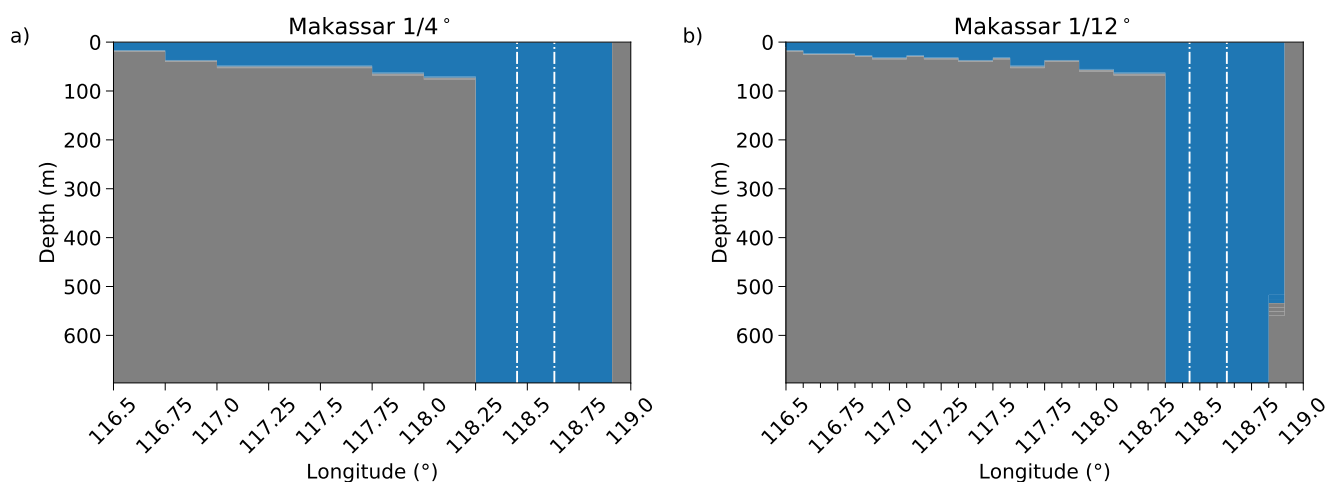
Figure 2. Bathymetries for the cross-passage interpolation of ASVs as given by the a) 1/4^\circ \times 1/4^\circ (75 levels) and b) 1/12^\circ \times 1/12^\circ (50 levels) products in Makassar Strait. White dash-dot lines represent mooring locations.
