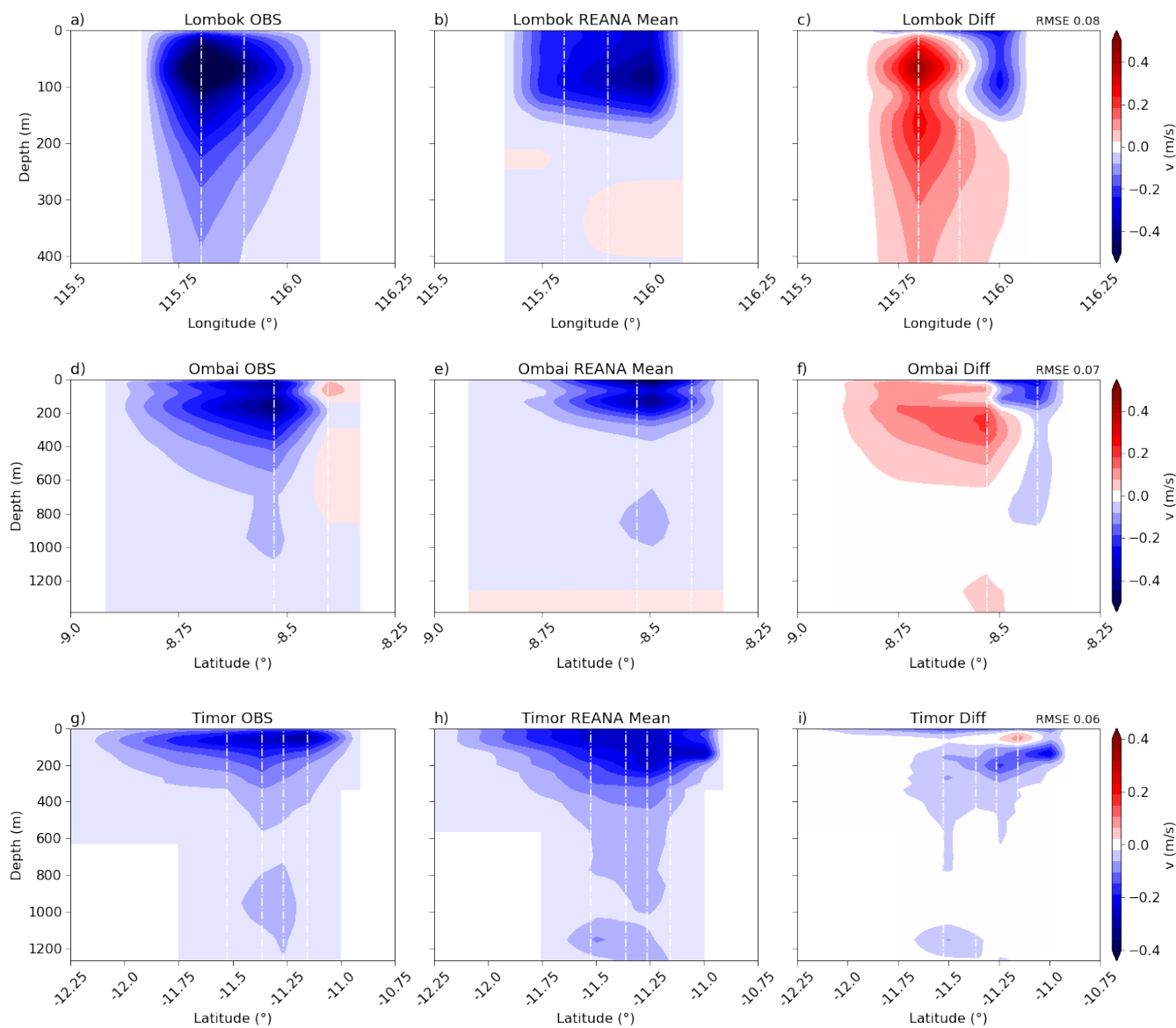
Figure A1. Mean ASV cross sections for a-c) Lombok Strait, d-f) Ombai Strait, and g-i) Timor Passage as given by the observations (left), the GREP mean (middle). The far right column corresponds to the respective differences between observations and GREP mean with the RMSE given in the top right corner. White dash-dot lines represent mooring locations. Negative values indicate southward-directed velocities (towards the Indian Ocean).
