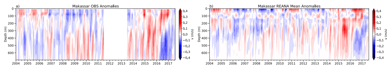
Figure 8. Monthly time series of ASV anomalies in Makassar Strait as represented by a) the observations and b) the GREP mean. Note the missing observational data between July 2011 and August 2013. Negative values indicate southward-directed velocities (towards the Indian Ocean).
