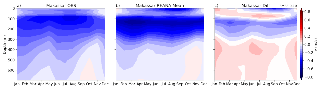
Figure 5. Mean annual cycle of ASVs for Makassar Strait as given by the 1/4^\circ bathymetry for a) observations and b) the GREP mean. c) refers to their respective differences. RMSE between the observations and the GREP mean is given in the top right corner. Negative values indicate southward transport (toward the Indian Ocean).
