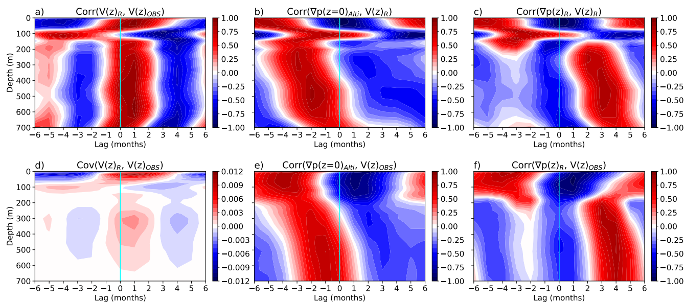
Figure A3. Analogous to Fig. 12 except the observed and reanalysis based monthly time series are replaced by 10-year time series consisting only of the mean annual cycle. Sea level gradients/pressure gradients refer to the ITF’s entrance and exit region. Considered time series cover the period between 2004 and 2017. Red (blue) values indicate positive (negative) correlations.
