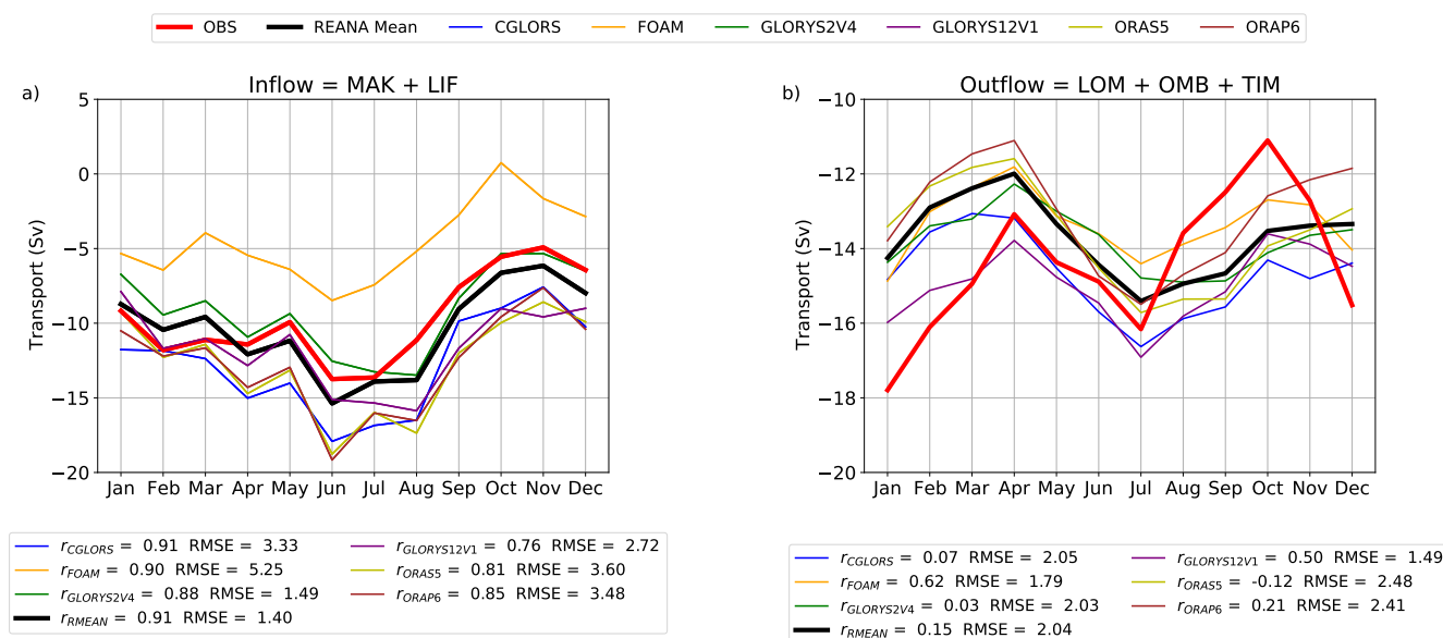
Figure A2. Mean annual cycles of ITF transport through a) the inflow passages (= Makassar Strait + Lifamatola Passage) and b) the outflow passages (= Lombok Strait + Ombai Strait + Timor Passage) as represented by observations and reanalyses. Observations in Lifamatola Passage are only available below 400 m. Subjacent boxes display corresponding Pearson correlation coefficients r and RMSEs. Note that all annual cycles refer to the INSTANT period (January 2004-December 2006). Negative values indicate southward-directed transports (towards the Indian Ocean).
