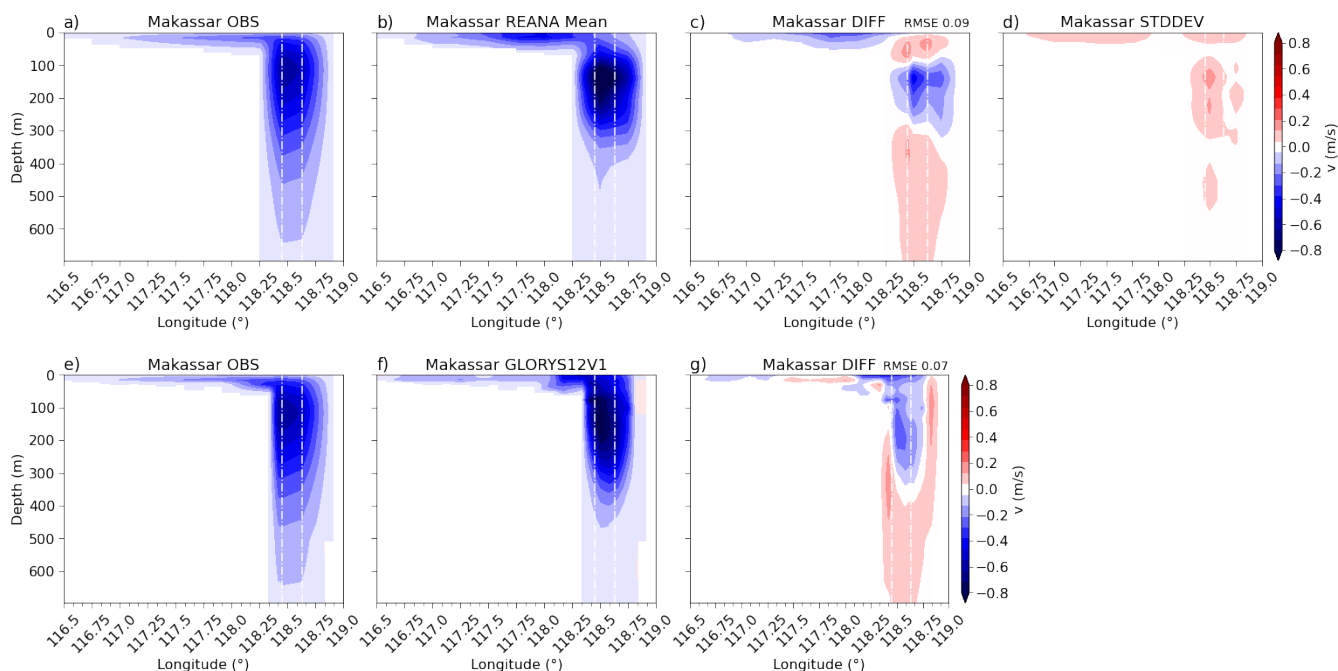
Figure 4. Mean ASV cross sections for Makassar Strait as given by a,e) the observations, b) the GREP mean, and f) GLORYS12V1 for the 1/4^\circ (upper panel) and the 1/12^\circ (lower panel) bathymetry. c,g) correspond to the respective differences between observations and GREP mean with the RMSE given in the top right corner. The standard deviation of the individual products around the GREP mean is shown in d). White dash-dot lines represent mooring locations. Negative values indicate southward-directed velocities (towards the Indian Ocean).
