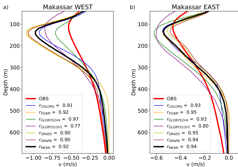
Figure 3. Mean ASV profiles for a) Makassar west and b) Makassar east. Corresponding correlation coefficients between observations and reanalyses are given in the boxes in the lower left. Negative values indicate southward-directed velocities (towards the Indian Ocean).
