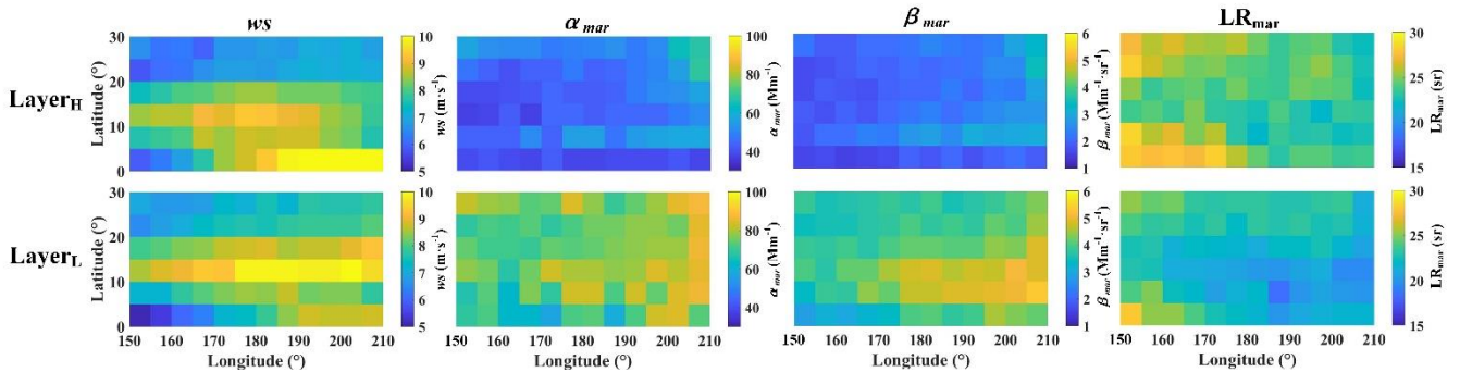
300 Figure 4: Wind speed ( ws ), marine aerosol extinction coefficient ( \alpha_{mar} ), marine aerosol backscatter coefficient ( \beta_{mar} ), and marine aerosol lidar ratio ( LR_{mar} ) spatial distributions above the North Pacific (NP) area at Layer_H and Layer_L .
