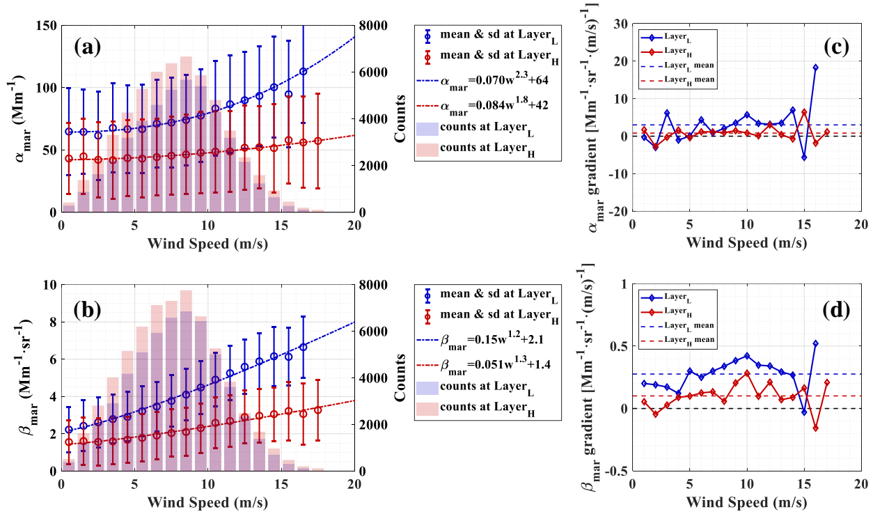
390 Figure 8: Relationship between marine aerosol optical properties ((a) for \alpha_{mar} , (b) for \beta_{mar} ) and wind speed above the NP area. The blue circles and error bars represent the means and standard deviations of the optical properties along wind speed grids at Layer L , while the reds represent the same items at Layer H . The blue and red dotted-dashed lines are the optical property averages regression curves fitted along the wind speed grid at Layer L and Layer H , respectively. The blue and red histograms indicate the data counts of every wind speed grid at Layer L and Layer H , respectively. (c) and (d) represent the gradients of \alpha_{mar} and \beta_{mar} with wind speed at Layer L (blue lines) and Layer H (red lines), respectively, while the blue dashed lines and the red dashed lines show the mean values of the gradients at two layers. 395
