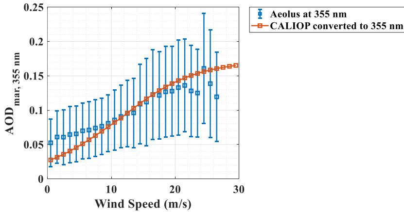
480 Figure 11: AOD_{mar} at 355 nm versus wind speed. The blue squares and the corresponding error bars represent the AOD_{mar} means and standard deviations along the ws grid of all the three study areas in this study; the red squares and line represent the AOD_{mar} at 355 nm along the ws grid converted from the regressive relationship between the AOD_{mar} at 532 nm and the ocean surface wind speed reported by Kiliyanpilakkil and Meskhidze (2011).
