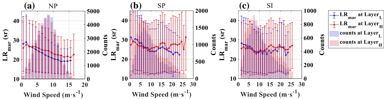
Figure 13: Averaged LR_{\text{mar}} versus wind speed at Layer L and Layer H , in (a) the NP area, (b) the SP area and (c) the SI area, respectively.
