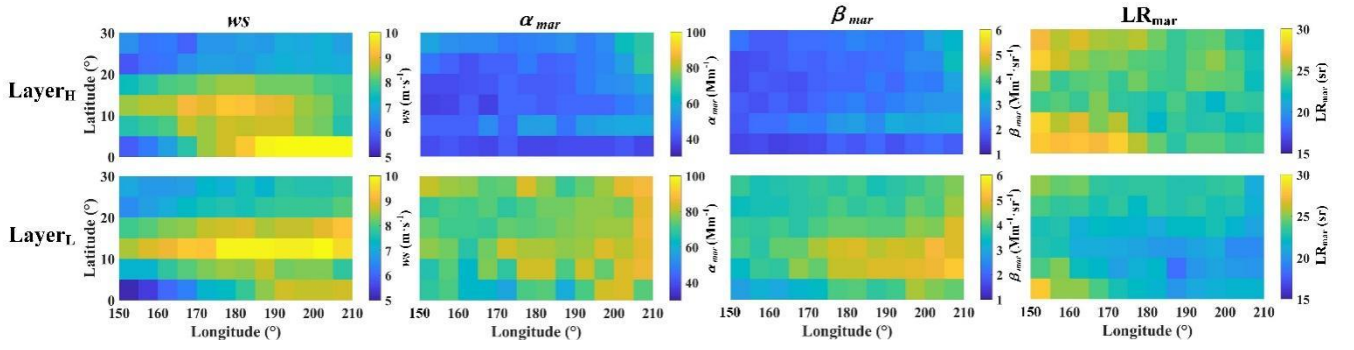
330 Figure 4: Wind speed ( ws ), marine aerosol extinction coefficient ( \alpha_{mar} ), marine aerosol backscatter coefficient ( \beta_{mar} ), and marine aerosol lidar ratio ( LR_{mar} ) spatial distributions above the North Pacific (NP) area at Layer_H and Layer_L .
