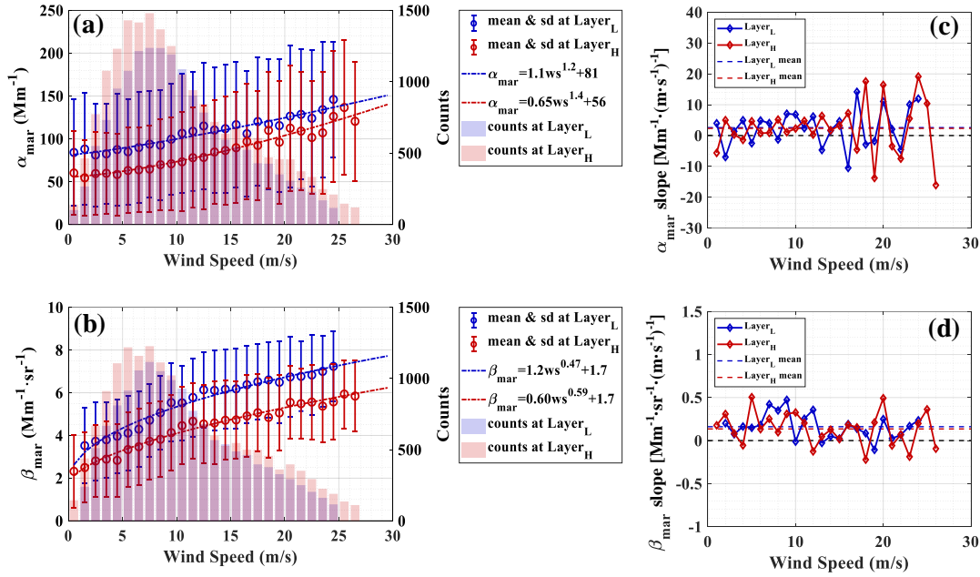
455 Figure 10: Relationship between marine aerosol optical properties and wind speed above the SI area. The items represent the same as those of Fig. 8.
