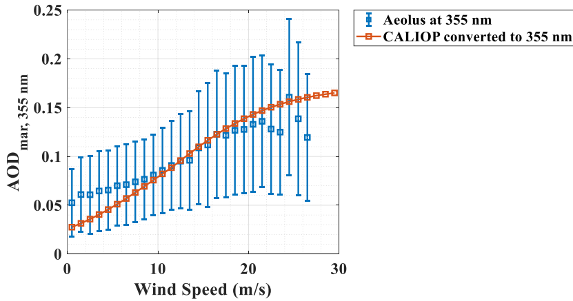
515 Figure 11: AOD_{mar} at 355 nm versus wind speed. The blue squares and the corresponding error bars represent the AOD_{mar} means and standard deviations along the WS grid of all the three study areas in this study; the red squares and line represent the AOD_{mar} at 355 nm along the WS grid converted from the regressive relationship between the AOD_{mar} at 532 nm and the ocean surface wind speed reported by Kiliyanpilakkil and Meskhidze (2011).
