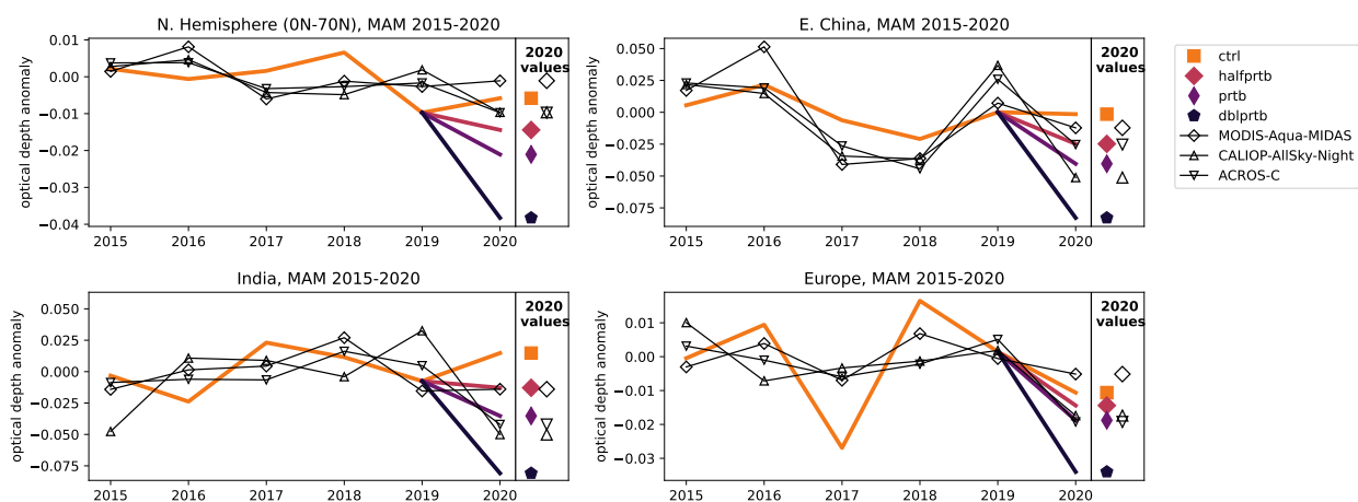
Figure 4. Effects of varying the magnitude of the simulated COVID-19 perturbation in CanAM5.1 . The control simulation, nudged to ERA5 fields, is shown in orange. The remaining symbols show simulations forced with COVID-19 perturbations half, one, and two times the magnitude of the original CovidMIP perturbation. All simulations use the updated baseline inventory introduced in Section 5.2.1.
