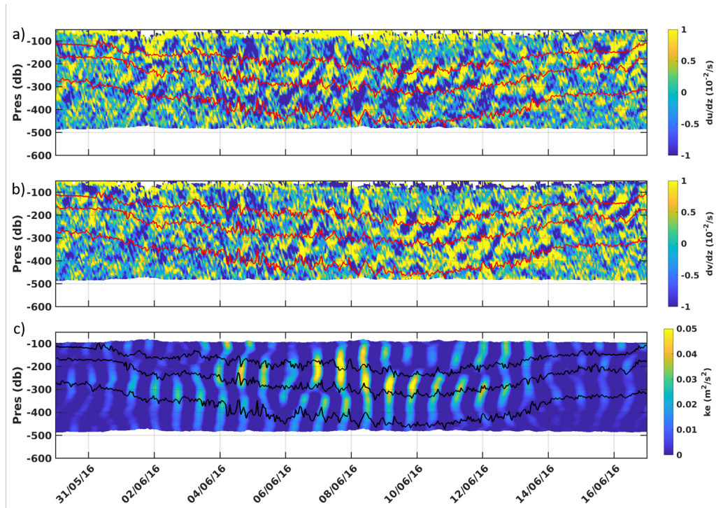
Figure 4: a-b) Vertical shear of velocity components for SUMO during event A1. c) 14-20 h band-pass filtered Ke for SUMO during event A1. Contours correspond to isopycnals 26.65, 26.85 and 27 \text{kg}/\text{m}^3 computed from the vertically interpolated data.
