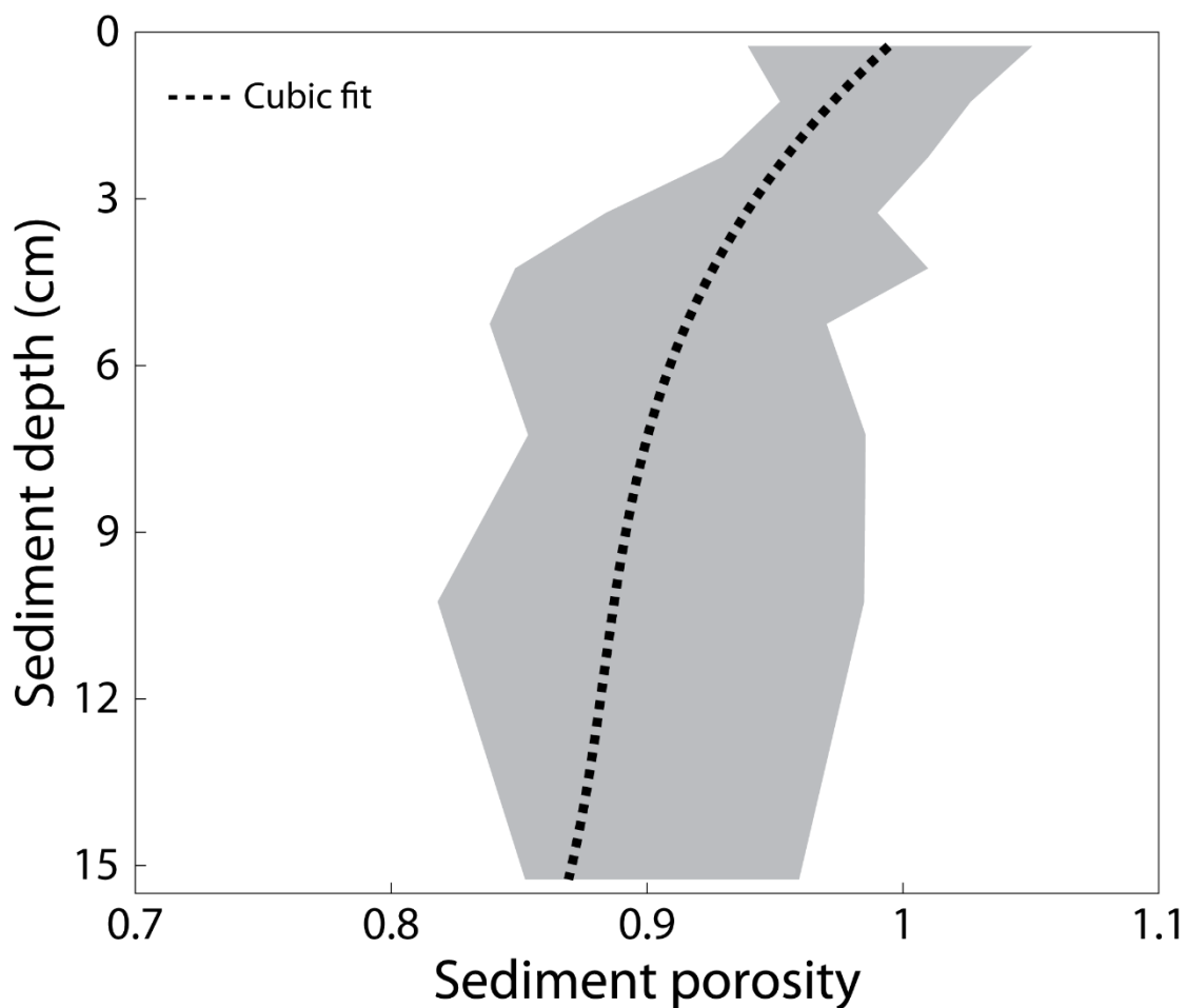
3 4 Supplementary Figure S1. Cubic fit of sediment porosity versus sediment depth (dotted 5 line) of all porosity data from sediment profiles across all sampling campaigns. Shaded 6 areas display the 25 th and 75 th percentile.
