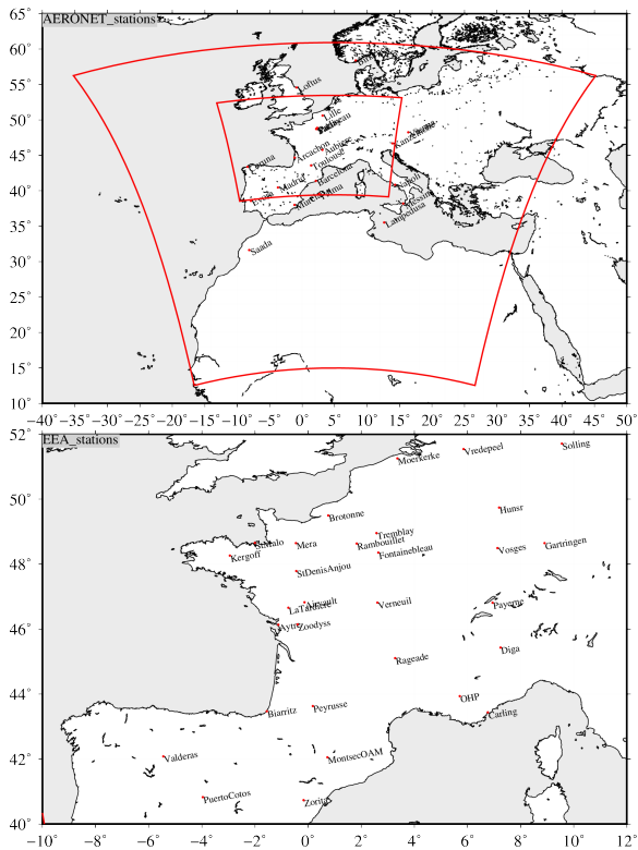
Figure 2. Maps of measurements stations of EEA and AERONET. The two nested model domains are represented as red frames. The largest one has an horizontal resolution of 50 km, when the second one has an horizontal resolution of 15 km.
