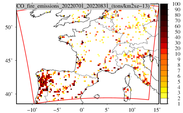
Figure 3. Time-averaged surface flux of CO emitted by fires during the months of July and August 2022 and calculated using the CAMS fires product. The studied Landes fires are those located around the longitude 0^\circ E and the latitude 45^\circ N.
