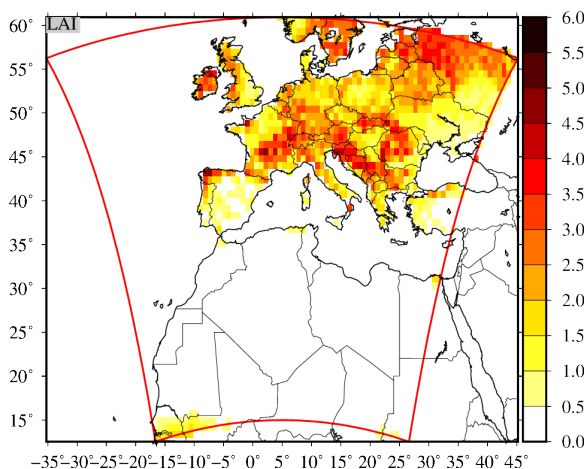
Figure B1. Model domain ( \Delta x=50\text{km} ) with the Leaf Area Index (LAI in \text{m}^2.\text{m}^{-2} ) used by the CHIMERE model and for the month of August.
