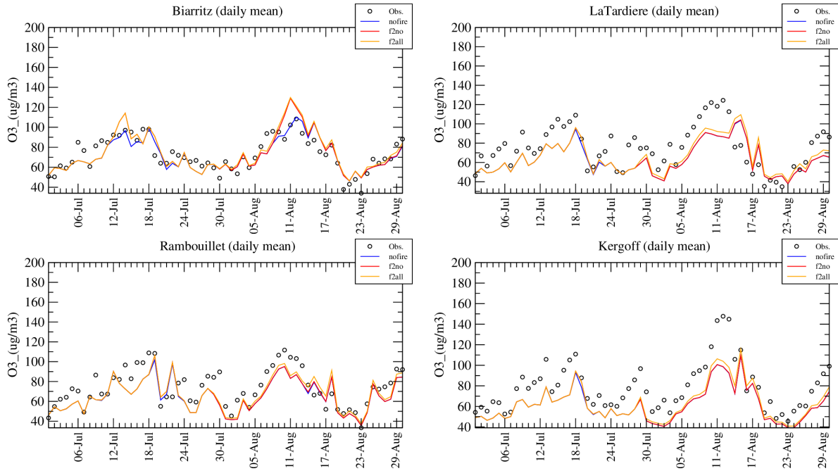
Figure 10. Time-series of daily averaged surface ozone concentrations in Biarritz, LaTardiere, Rambouillet and Kergoff.
