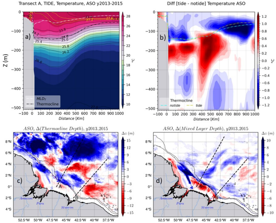
1100 1101 Figure 7. Same as figure 6 but for ASO season.
