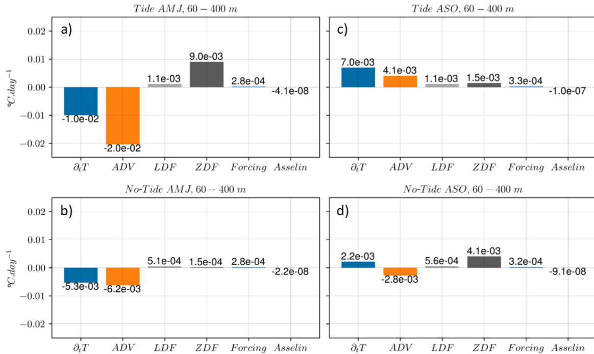
1197 1198 Figure 11. Three-dimensional heat budget equation terms averaged in region around IT 1199 trajectories between 48^\circ W-40^\circ W and 0^\circ N-6^\circ N , and below the MLD between 60-400 m depth. 1200 Upper panels are for the tidal simulations and lower panels for the non-tidal simulations, while 1201 left and right panels are for the AMJ and ASO seasons, respectively. 1202
