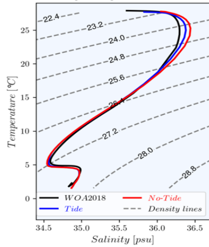
g) T-S diagram depth range : 0 – 5500 m
