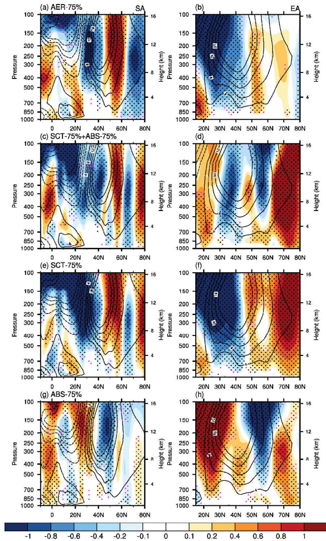
950 Figure 10: Same as Figure 9, but for the zonal-mean zonal wind (shading; unit: \text{m s}^{-1} ; red and blue denote westerly and easterly wind, respectively) responses during monsoon season. Monsoon season is analyzed and based on the definitions from W2009 over South Asia and W2016 over East Asia. Black lines represent the climatological zonal wind from control simulations (unit: \text{m s}^{-1} ; solid and dash lines denote westerly and easterly wind, respectively).
