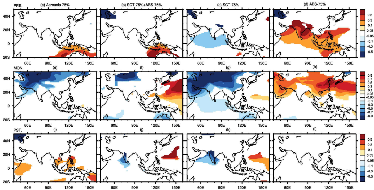
935 Figure 8: Spatial distributions of the sea level pressure (unit: hPa) responses to the reductions in total aerosols (a, e and i), SCT aerosols (c, g and k) and ABS aerosols (d, h and l) over Asia during pre-monsoon (April-May; a-d), monsoon (June-August; e-h) and post-monsoon (September-October; i-l) seasons. The sea level pressure responses are the difference between the aerosol-emission-perturbed and control runs. Panels (b), (f) and (j) are the sum of the impacts of the reductions in the SCT and ABS. Only the sea level pressure changes with a confidence level of 95% or 90% according to the t-test are shown.
