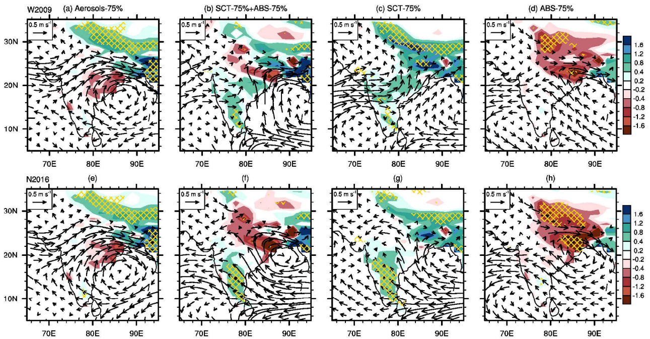
Figure 5: Spatial distributions of the monsoon precipitation (shading; unit: mm day -1 ) and 850-hPa wind fields (vector; unit: m s -1 ) responses to the reductions in total aerosols (a and e), scattering aerosols (SCT; c and g) and absorbing aerosols (ABS; d and h) over South Asia. Panels (b) and (f) are the linear addition of the impacts of the reductions in the SCT and ABS. Hatched regions denote where the precipitation change is statistically significant at the 95% confidence level according to a Wilcoxon rank sum test. Panels (a)-(d) are derived based on the definition from W2009. Panels (e)-(h) are derived based on the definition from N2016. The SASM adjustments forced by emission reductions in different aerosol types are the difference between the aerosol-emission-perturbed and control runs.
