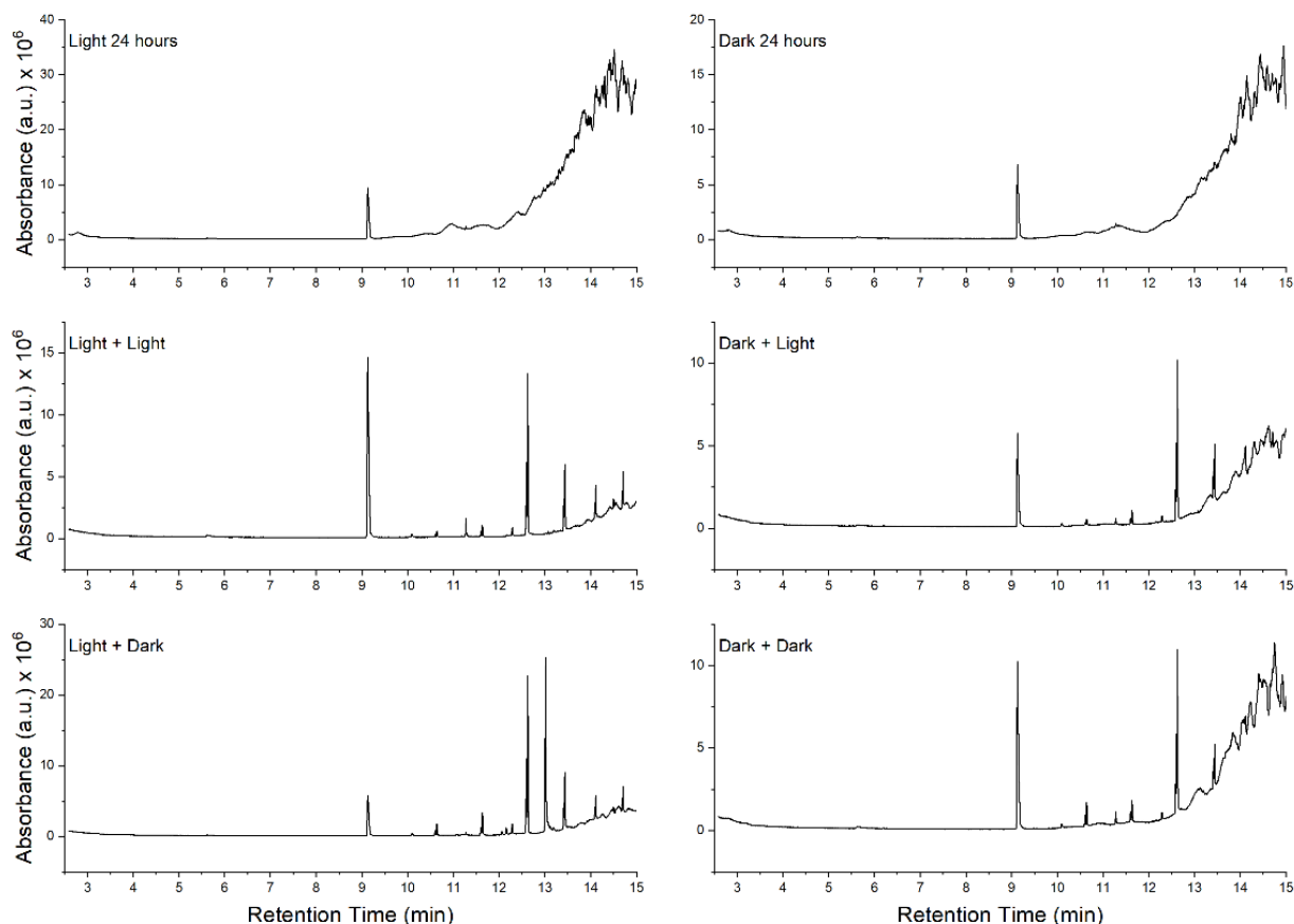
210 Figure 6 Gas chromatograms of soot at each step of the aging process. The left column contains chromatograms of soot extracts taken from the photo-aged pathway (samples B → E & D), and the right column contains extracts of soot that followed the dark-aged pathway (samples C → G & F). The first row is extracts from the soot after initial 24 hours of aging. The second row is soot that was photo-aged in water for 16 hours, and the bottom row is soot that was dark aged in water for 16 hours.
