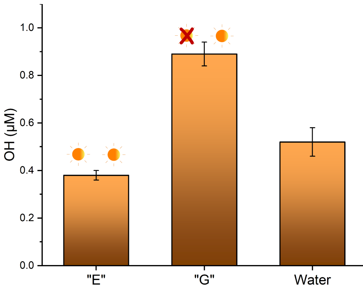
Figure 5 Concentrations of OH measured from lighted reactions of soot that had been previously aged for 24 hours in the light (E), aged for 24 hours in the dark (G) and an ultrapure water control.
