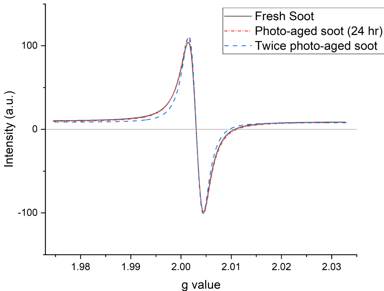
260 Figure A1 Representative EPR spectra of three soot samples at different stages of photo-aging, Fresh (black, solid line), soot aged for 24 hours under simulated sunlight (red dash-dot), and soot photo-aged twice, once dry, and once wet (blue, dash-dash). Signals have been baseline corrected and intensity normalized.
