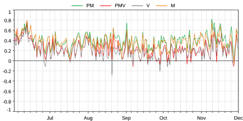
Figure 10: Temporal evolution of MNMB of the mean daily analysis of AOD for the PM, PMV, V and M experiments, evaluated against level-2 AERONET AOD measurements at 500nm from 18 desert sites (a) and 11 oceanic sites (b).
