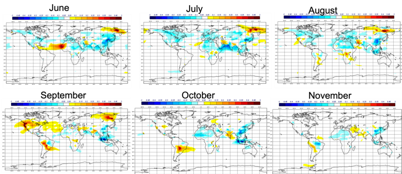
240 Figure 1: CAMS monthly AOD reanalysis anomalies in 2020 (computed as the difference between monthly average 2020-monthly average over the period 2003-2020)
