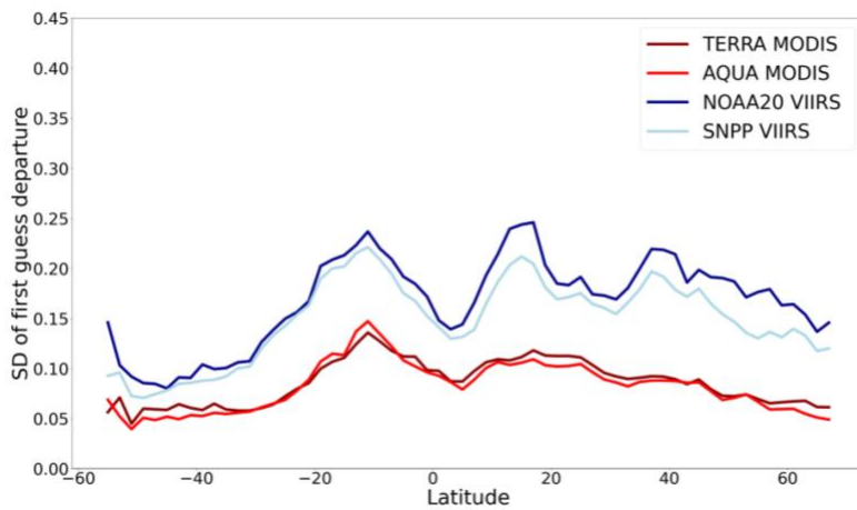
Figure 5: Latitude cross-section of FGD SD, for the JJA (a) and SON (b) periods over land
