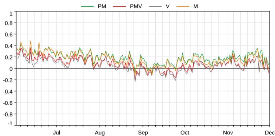
450 Figure 11: Temporal evolution of MNMB of the mean daily analysis of AOD for the PM, PMV, V and M experiments, evaluated against level-2 AERONET AOD measurements at 500nm from 106 European sites (a), 130 North America sites (b), 80 South-East Asia sites (c) and 53 Africa sites (d).
