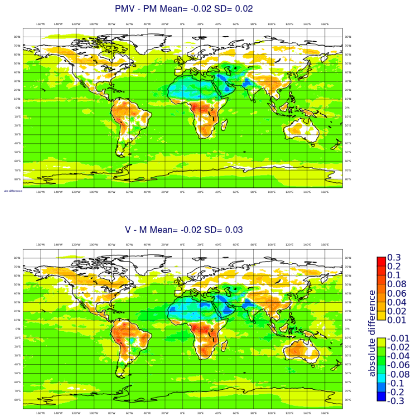
370 Figure 6: Difference in mean JJA (a) and SON (b) AOD daily analysis between i) PMV and PM and ii) M and V experiments.
