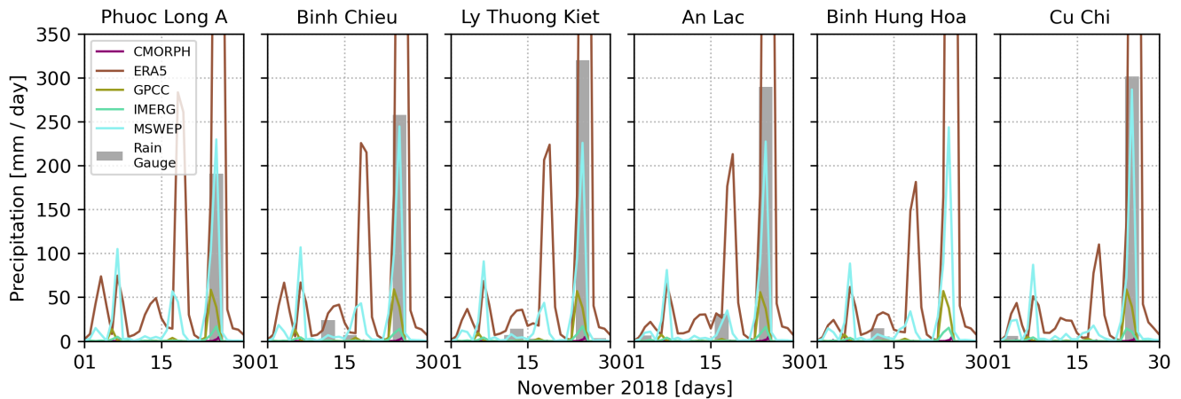
Figure 5. The 5 precipitation products compared to the 6 rain gauges with available observations for the month of November 2018. The peak of precipitation during TY Usagi is best captured by MSWEP (light blue) whereas the other datasets either underestimate or overestimate it. The ERA5 (brown) presents estimations above 500 mm. The high spatial variability over the city makes it hard to obtain accurate results at all stations simultaneously.
