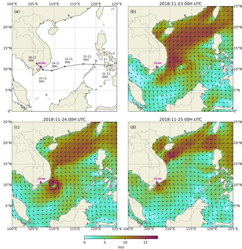
Figure 2. (a) The track of TY Usagi and Ho Chi Minh City (pink); (b–d) ERA5 10-m wind fields from November 23rd, 2018 00H UTC to November 25th, 2018 00H UTC.
