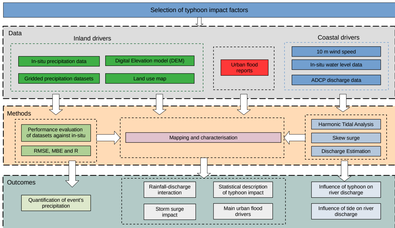
Figure 3. Framework to characterize and study the compound flood drivers brought by TY Usagi on the estuarine system. All typhoon-related phenomena that influences coastal dynamics (such as storm surge and wind) is referred to as “coastal” effects. Typhoon-related phenomena influencing the hydrology (precipitation, surface run-off, river discharge, flooding) is referred as “inland’ effects.
