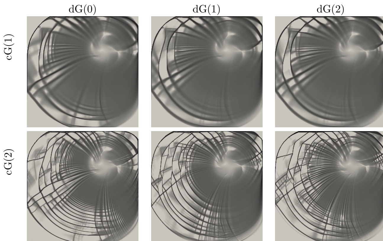
Figure 9. Shear deformation ( \log_{10} ) for the benchmark at time T = 2 days. We compare different combinations of cG velocity discretizations (linear and quadratic) with dG advection discretization (constant, linear and quadratic). All computations are run on meshes with the grid spacing h = 2 km.
