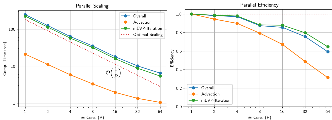
Figure 14. Scaling (left) and parallel efficiency (right) of the OpenMP parallelization for the benchmark test case on the 2 km mesh. The mesh has 65 536 elements, a total of 60 advection steps with 10 momentum substeps within the mEVP iteration are covered by the total time.
