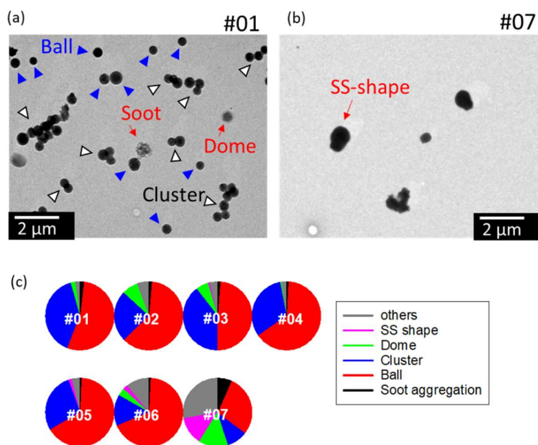
290 Figure 3: Electron micrographs for samples #01 (a) and #07 (b), and Pie chart showing the number fractions of morphological types (c). Blue arrowed particles are ball-like shaped particles. White arrowed particles are clusters of balls. Red arrows indicate soot, dome-shaped, and sea-salt (SS)-shaped particles.
