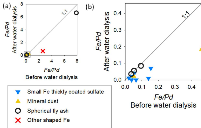
500 Figure 10: Scatter plot of Fe weight normalized Pd weight before and after water dialysis for Fe-containing particles on sample #03. (b) is an enlarged graph of the light-gray square area of (a). Pd is a coating material in alloy for shadowing to samples.
