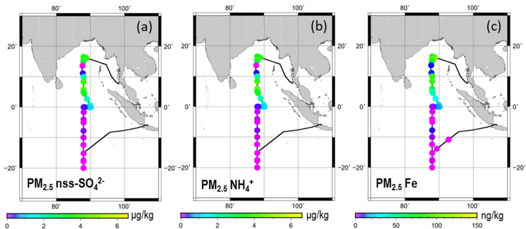
Figure 2: Horizontal variation of mass concentrations of (a) nss- \text{SO}_4^{2-} , (b) \text{NH}_4^+ , and (c) Fe in PM_{2.5} . Each sample was collected continuously 12 h or 24 h under controlling by wind sector. Data are as shown at averaged locations for latitude and longitude during the sampling period.
