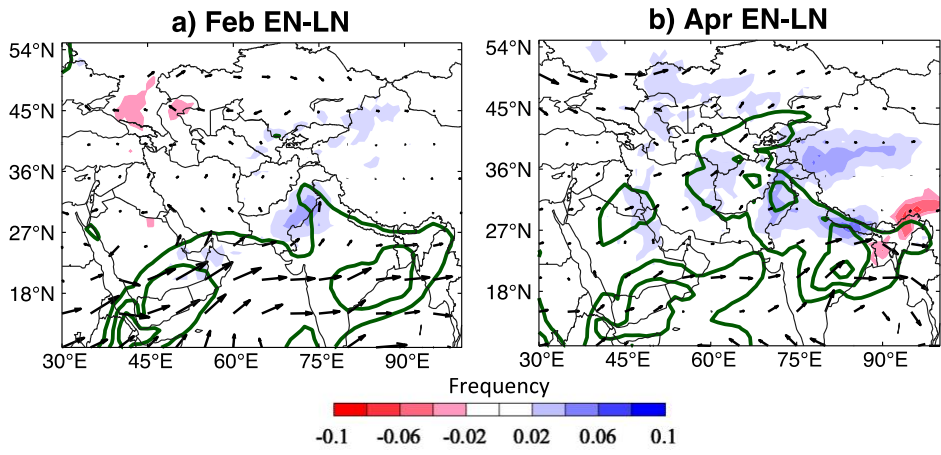
Figure S4: Panel a) is as in Fig. 10c but for February EN – LN months, and panel b) is as in Fig. 10c but for April EN – LN months. Plotting conventions are as in Fig. 10c,f.
