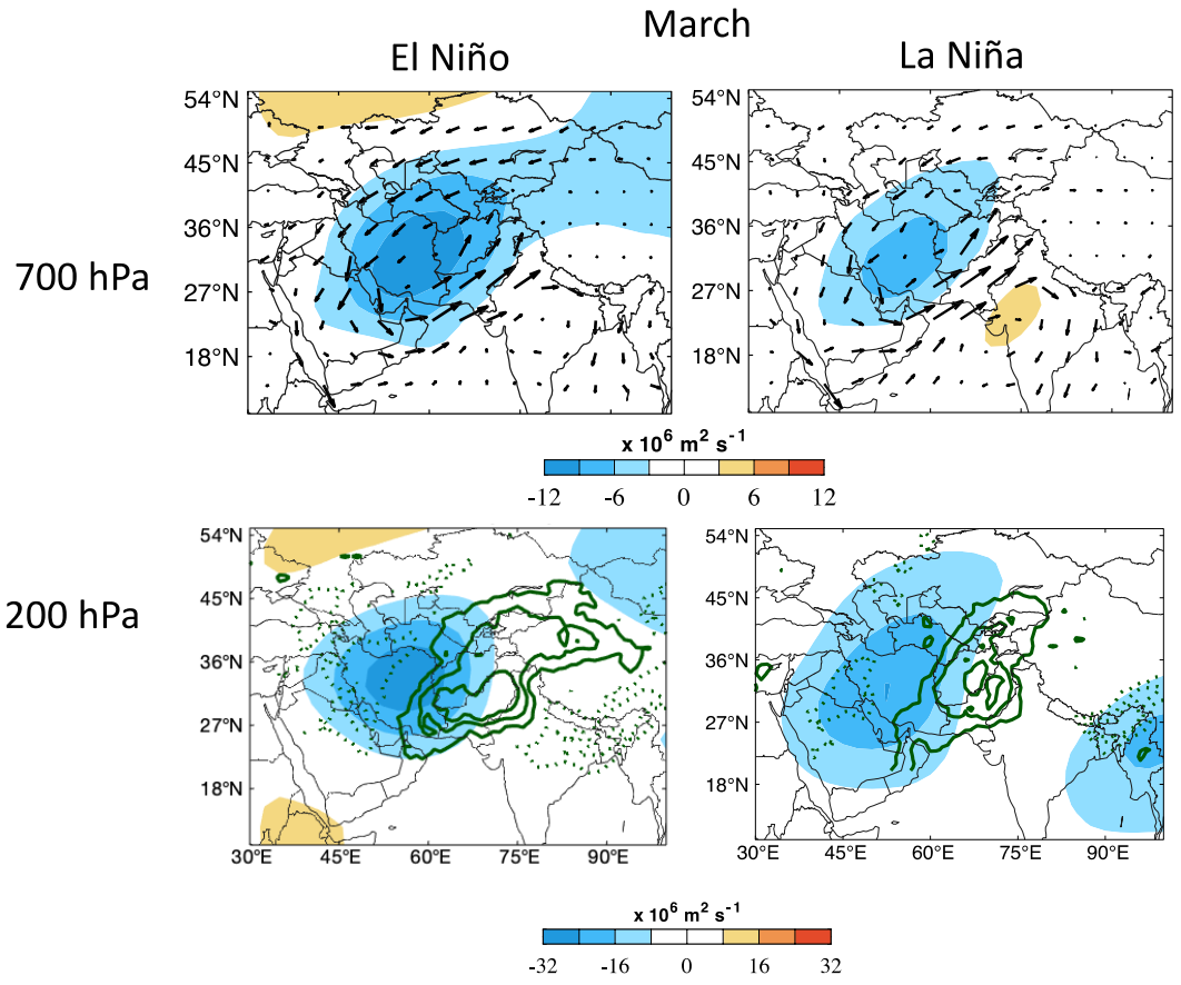
Figure S3: Composite difference between ‘wet’ days – meaning >4 mm accumulation days - subtracted from ‘dry’ days, when precipitation < 0.05 mm during El Niño (left) and La Niña (right) months. 700-hPa streamfunction and IVT (top) and 200-hPa streamfunction and WCB’s (bottom) on days when accumulation > 4 mm during El Niño conditions (left) and La Niña conditions (right). Plotting conventions are as in Figure 7.
