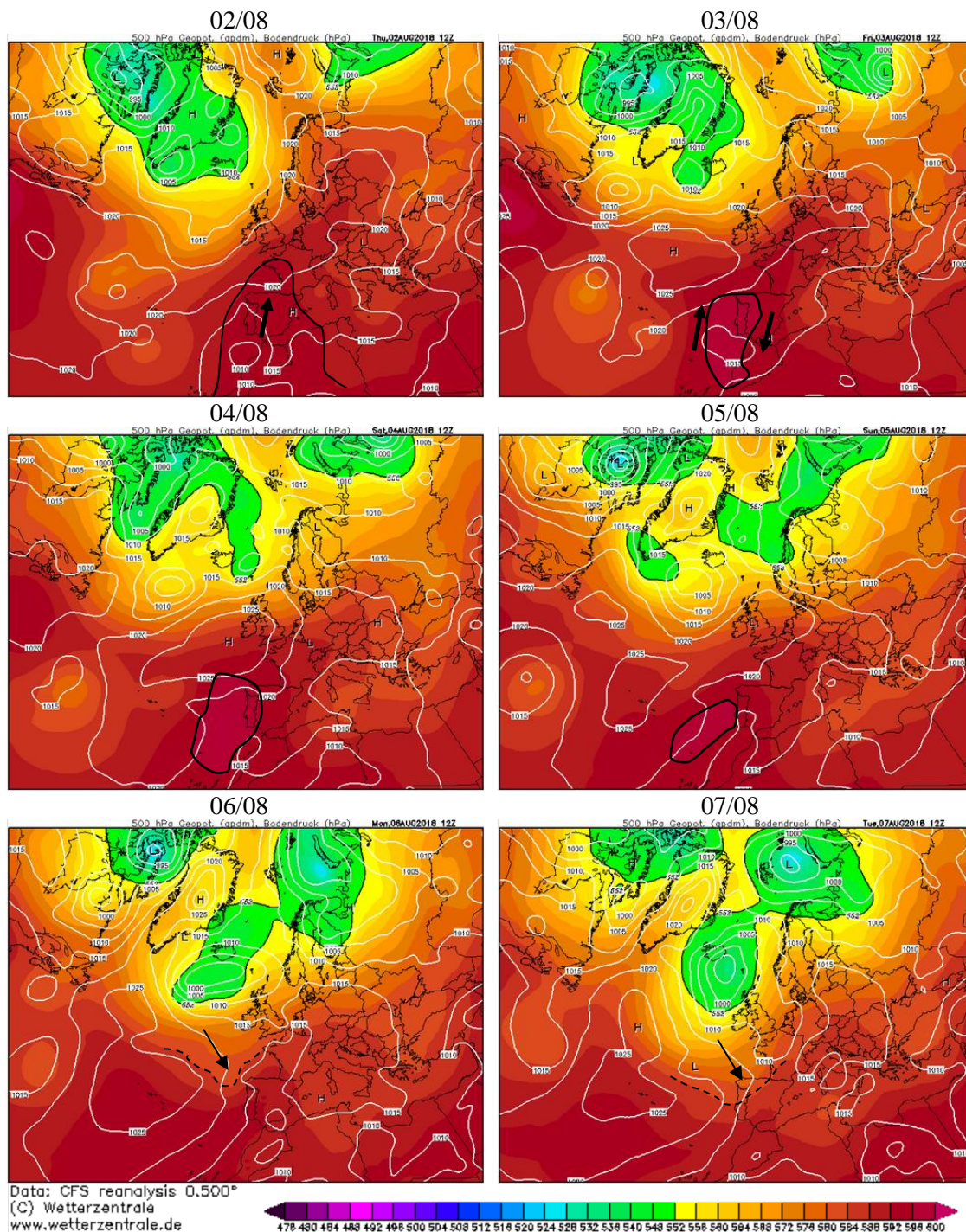
Figure 3. Synoptic conditions during the O 3 episode with geopotential height at 500 hPa (geopotential dm, shaded) and surface pressure (hPa, contours) during the period of the high ozone episode (August 2-7). L and H mean “low pressure centre” and “high pressure centre” respectively. Continuous black lines represent the warmer air mass over the IP and dashed black lines represent the Atlantic advection. Source: NCEP CFS reanalysis from www.wetterzentrale.de .
