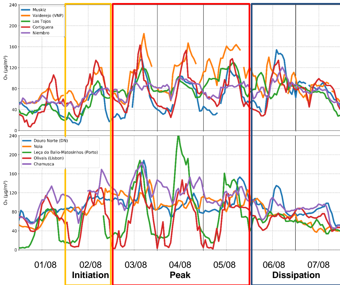
Figure 8. Ozone hourly concentrations time sequences for 1-7 August 2018 at a selection of stations along Northern Atlantic Iberia (top) and Western Atlantic Iberia (bottom).
