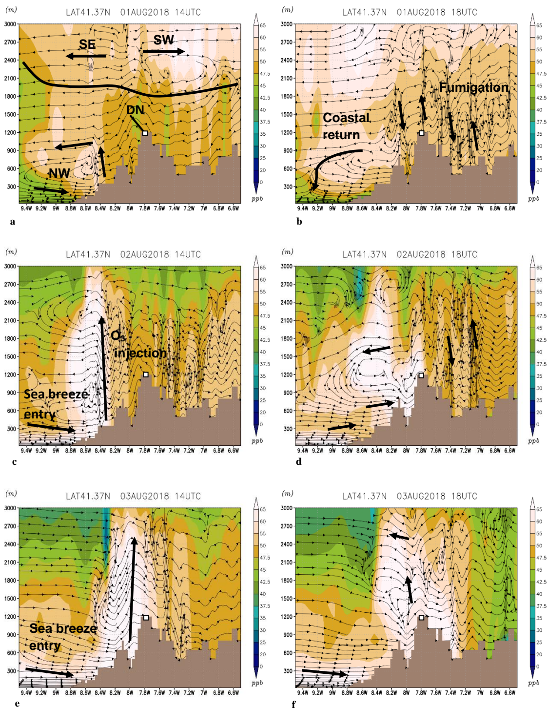
620 Figure 11. Simulated vertical O_3 concentrations (color scale) and projected wind fields (stream composed by projected v with w(*10) ) by WRF-CAMx in d03 at 14 UTC and 18 UTC on August 1, 2 and 3, 2018 for the DN vertical cross-section. Concentrations are depicted in ppb as they are altitude independent ( 1 \text{ ppb} \approx 2 \mu\text{g}\cdot\text{m}^{-3} at sea level).
