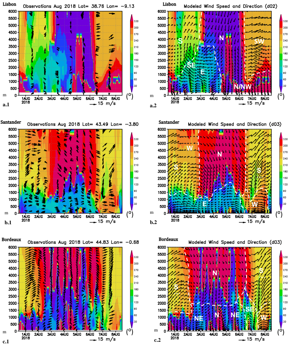
395 Figure 4. Wind vectors measured in radiosonde (left) and WRF simulations (right) for the period 01-08 August 2018. The range of colors in all graphics represents the simulated wind direction. The size of the vectors represents wind speed.
