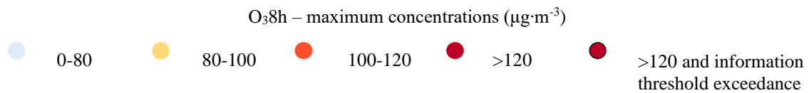
Figure 7. Daily evolution of the spatial distribution of maximum 8-hour O 3 concentrations, from 31 July to 8 August in 2018 .
