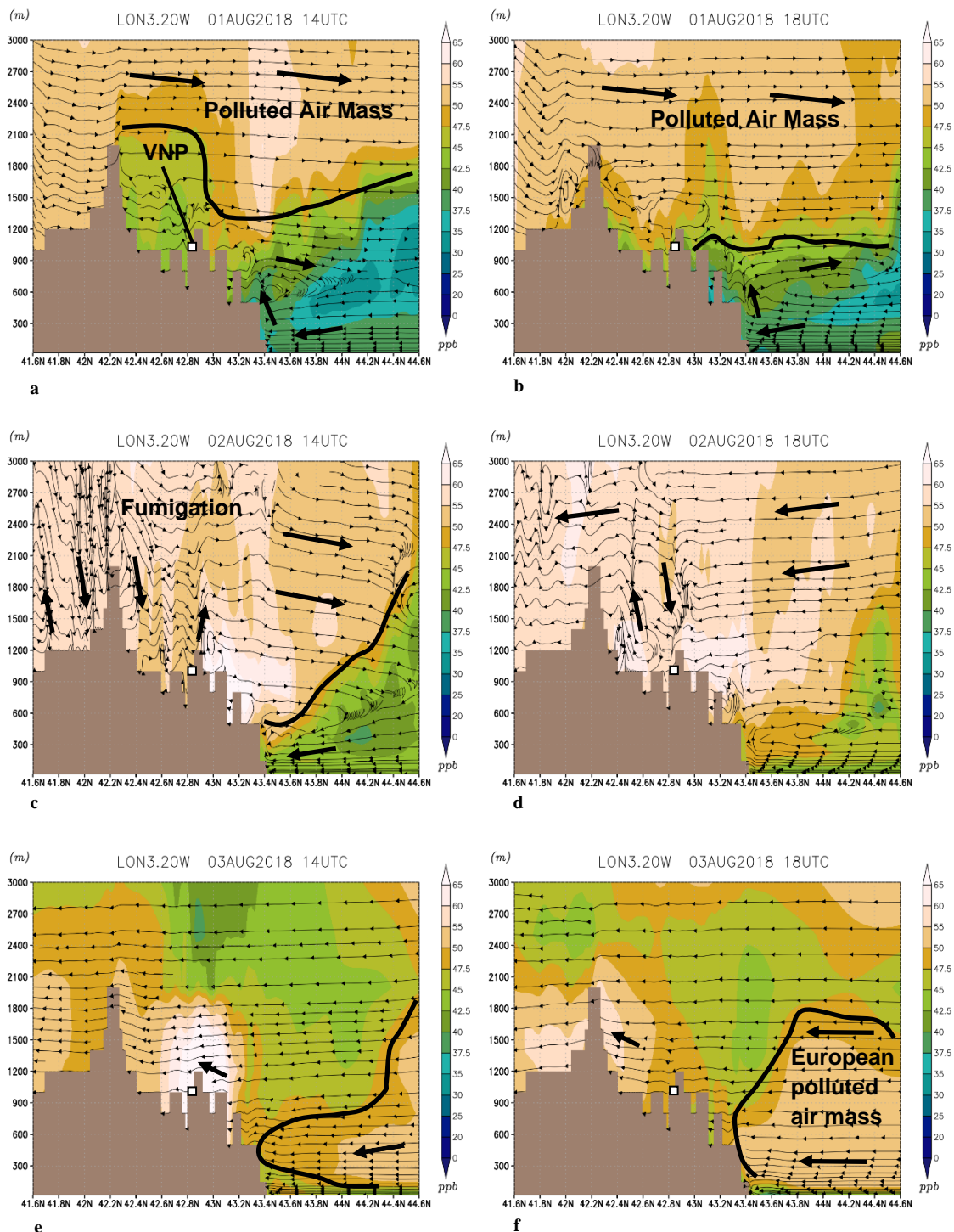
Figure 10. Simulated vertical O 3 concentrations (color scale) and projected wind fields (stream composed by projected u with w(*10)) by WRF-CAMx in d03 at 14 UTC and 18 UTC on August 1, 2 and 3, 2018, for the VNP vertical cross-section. Concentrations are depicted in ppb as they are altitude independent (1 ppb ≈ 2 μg·m -3 at sea level).
