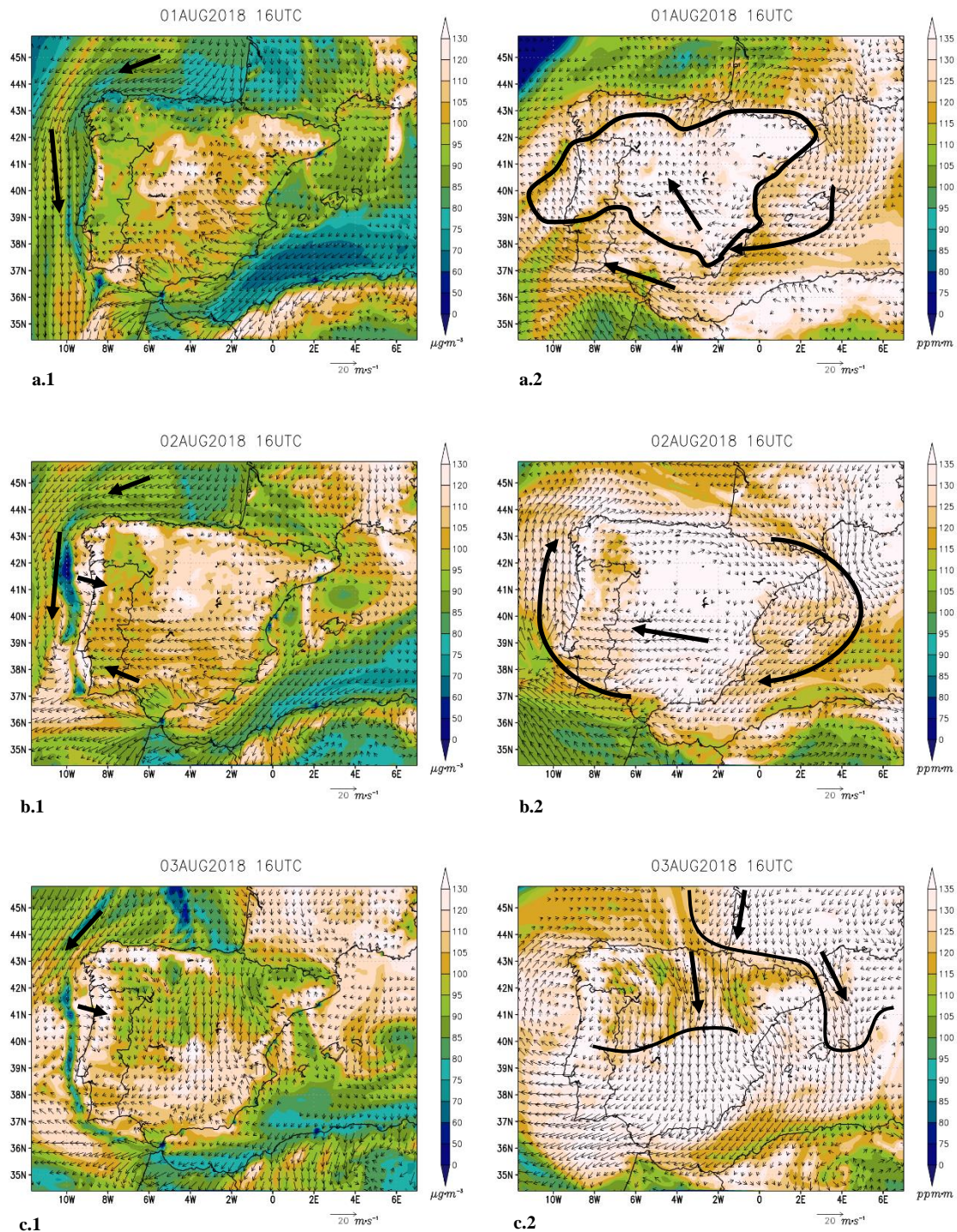
555 Figure 9. Simulated O 3 concentrations (color scale) and wind fields (vectors) by WRF-CAMx in d02 at 16 UTC on August 1, 2 and 3, 2018. Left panels show the ozone and wind concentration in surface and right panels the integrated ozone concentration up to 2,500 m AGL and wind at 1,250 m AGL. Winds lower than 2 m s -1 have been omitted.
