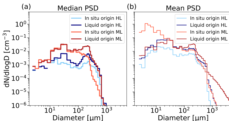
Figure 8. (a) Median and (b) mean particle size distributions (PSD) of the groups: in situ origin HL cirrus (light blue), liquid origin HL cirrus (navy), in situ origin ML cirrus (light red) and liquid origin ML cirrus (dark red). Median PSDs are indicated with thick lines and means with thinner lines.
