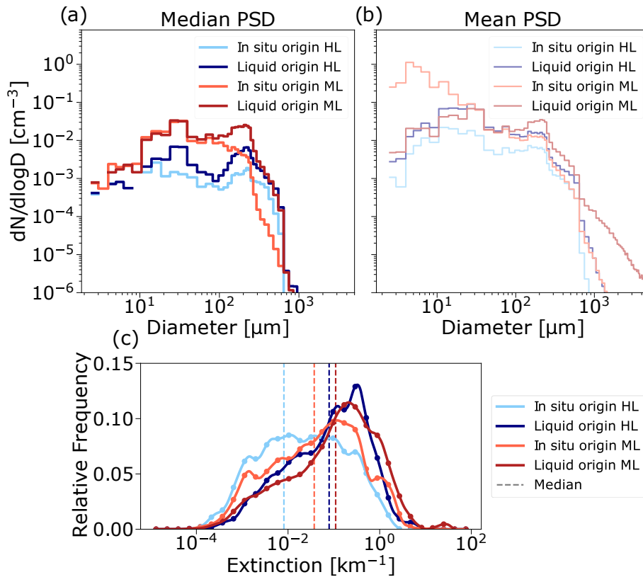
Figure 8. (a) Median and (b) mean particle size distributions (PSD), and (c) extinction coefficient ( \beta_{ext} ) of the groups: in situ origin HL cirrus (light blue), liquid origin HL cirrus (navy), in situ origin ML cirrus (light red) and liquid origin ML cirrus (dark red). Median PSDs are indicated with thick lines and means with thinner lines. The frequency of occurrence of \beta_{ext} was calculated in logarithmic bins and fitted with B-Splines.
