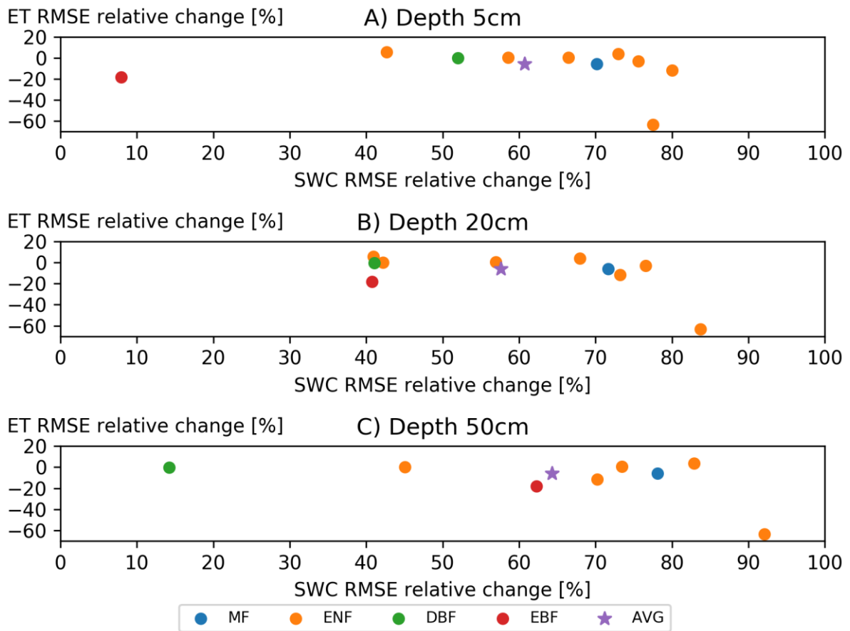
745 Figure 13: Comparing the SWC and ET characterization for the OL and DASP simulations using CLM5-SP. Each point represents the overall average RMSE change for one site. The color of the points indicate the forest type (MF: mixed forest, ENF: evergreen needle leaf forest, DBF: deciduous broad leaf forest, EBF: evergreen broad leaf forest, AVG: average over all forest types).
