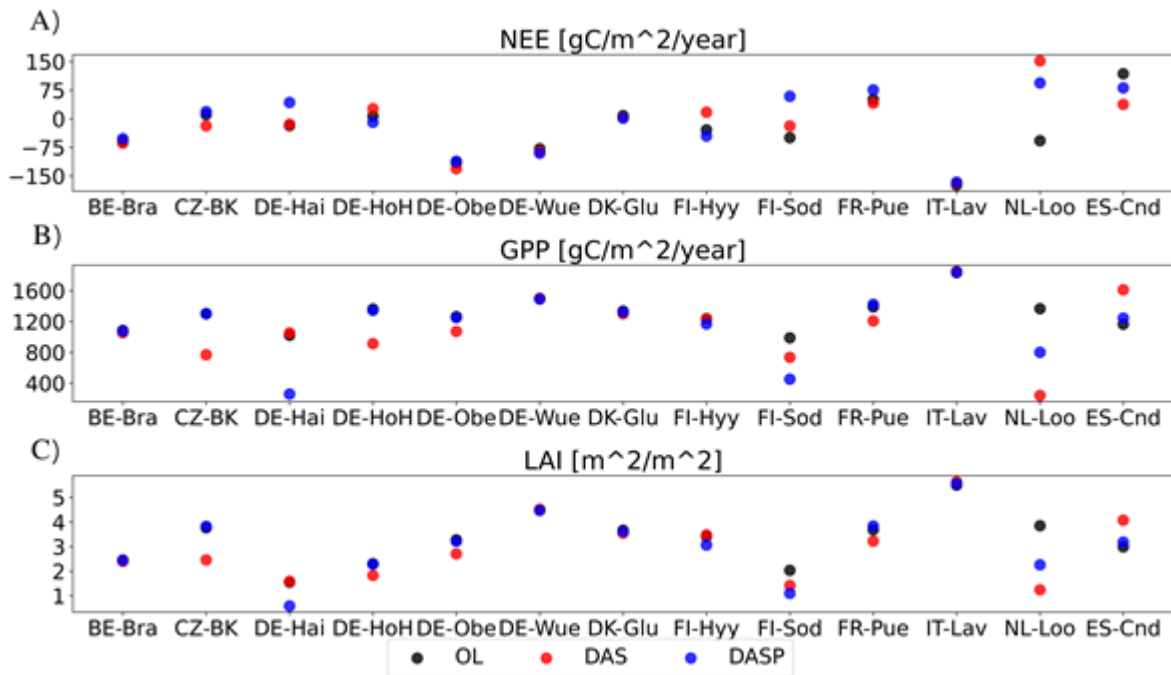
Figure 16: Open loop (OL) and assimilation scenario (DAS and DASP) yearly averages of A) net ecosystem exchange (NEE), B) gross primary production (GPP), and C) leaf area index (LAI) for all selected sites.
