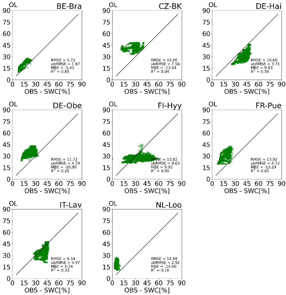
790 Figure A6: Scatter plots of observed soil water content at eight study sites versus OL simulation results at 50 cm depth. The points represent daily averages for the days on which observation data are available.
