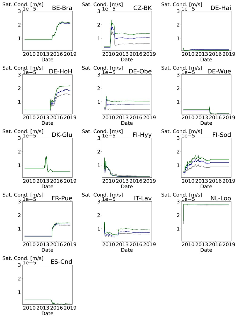
Figure 6: Time series of the saturated soil hydraulic conductivity for each site in the DASP simulation. The grey line is the value at 5 cm depth, the blue line at 20 cm depth, and the green line at 50 cm depth.
