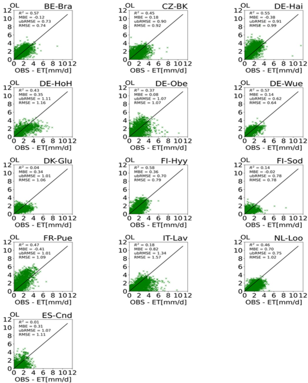
Figure 10: Scatter plots of observed evapotranspiration at thirteen study sites versus OL simulation results. The points represent daily averages for the days on which observation data are available.
