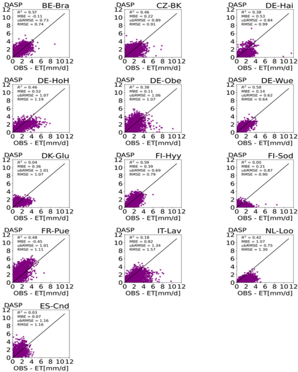
735 Figure 11: Scatter plots of observed evapotranspiration at thirteen study sites versus DASP simulation results. The points represent daily averages for the days on which observation data are available.
