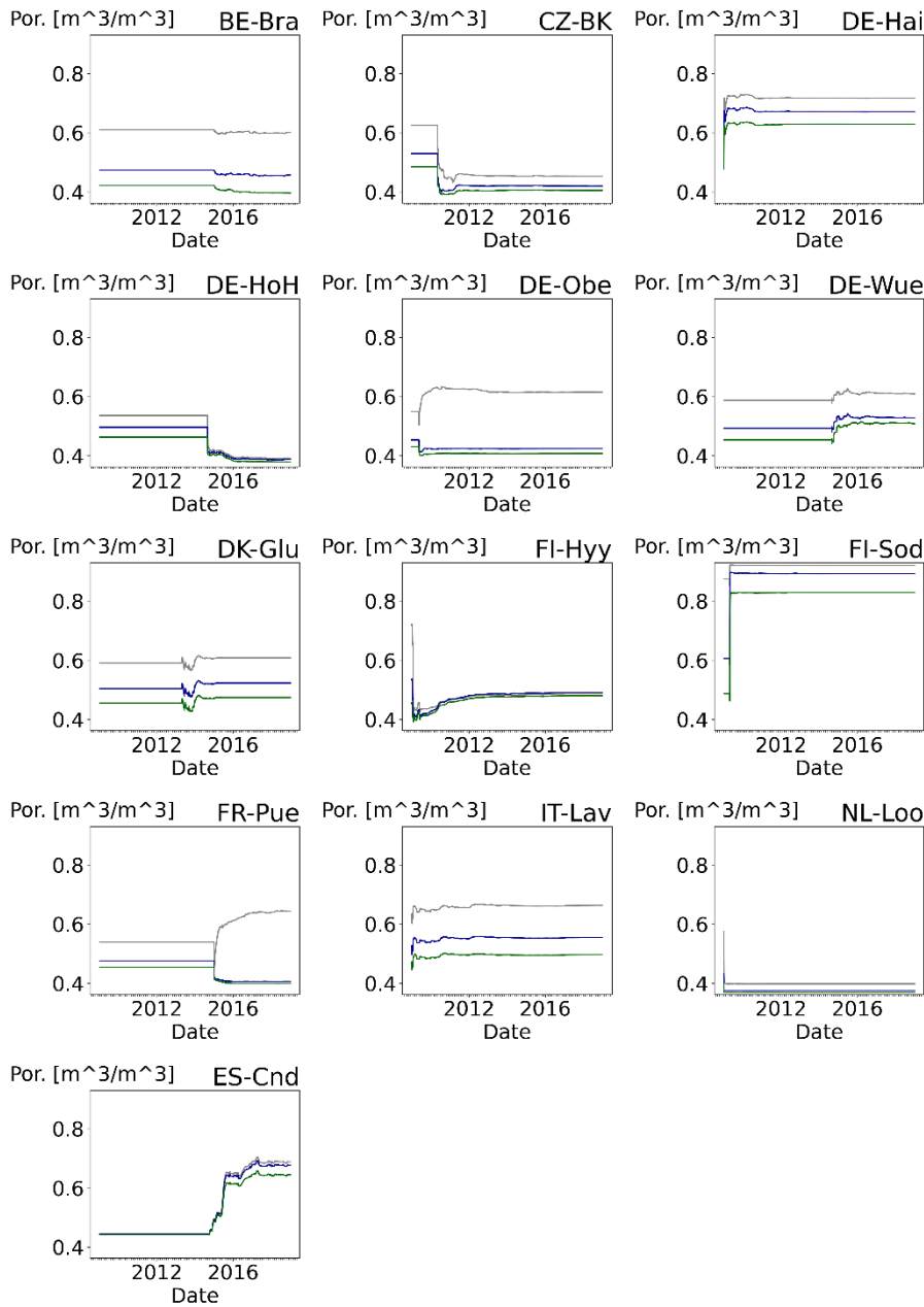
805 Figure A10: Time series .for the porosity for each site in the DASP simulation. The grey line is the value at 5 cm depth, the blue line at 20cm depth, and the green line at 50cm depth.
