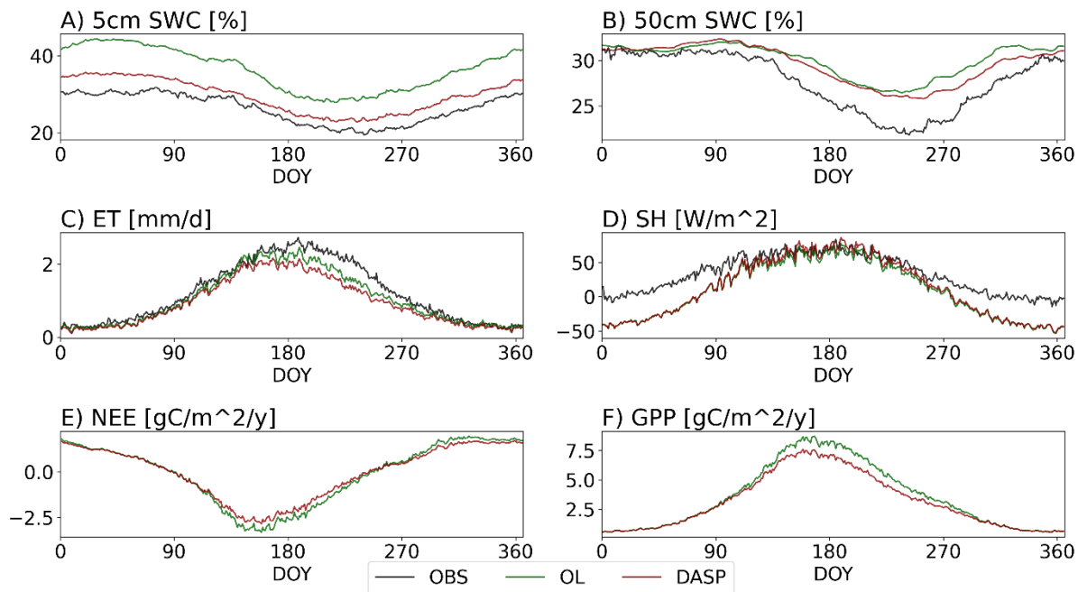
Figure 17: Seasonality of observed (OBS) and simulated (OL and DASP) states and fluxes based on daily averages from all years (2009 to 2018) and all sites: A) soil water content (SWC) at 5 cm depth, B) SWC at 50 cm depth, C) evapotranspiration (ET), D) sensible heat flux (SH), E) net ecosystem exchange (NEE), and F) gross primary production (GPP).
