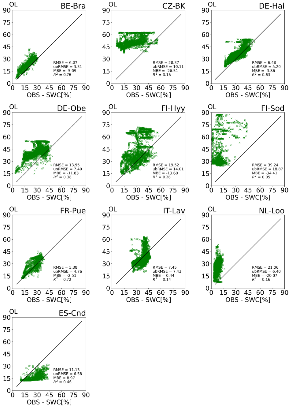
775 Figure A1 : Scatter plots of observed soil water content at ten study sites versus OL simulation results at
