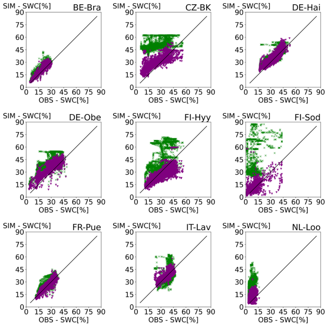
690 Figure 3: Scatter plots of observed soil water content at 20 cm depth at nine study sites versus OL and DASP simulated soil water content results at 20 cm depth. The points represent daily averages for the days observation data are available. Green points are OL and purple points are DASP results.
