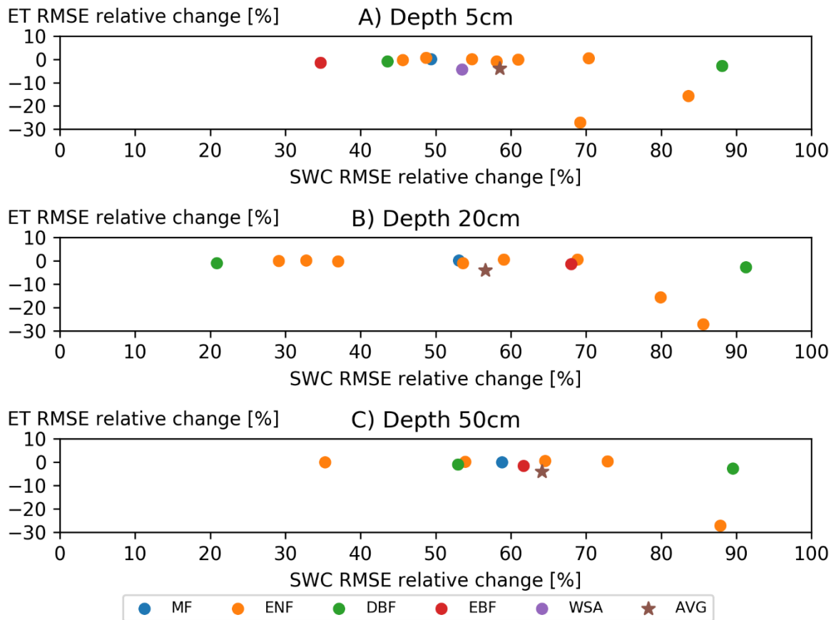
Figure 8: Comparing the SWC and ET characterization for the OL and DASP simulations. Each point represents the overall average RMSE change for one site. The color of the points indicates the classification code for the different forest types (MF: mixed forest, ENF: evergreen needle leaf forest, DBF: deciduous broad leaf forest, EBF: evergreen broad leaf forest, AVG: average over all forest types).
