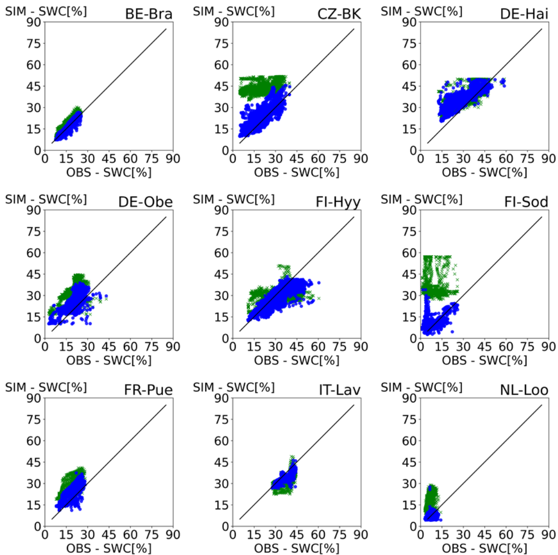
685 Figure 2: Scatter plots of observed soil water content at 20 cm depth at nine study sites versus OL and DAS simulated soil water content. The points represent daily averages for the days observation data are available. Green points are OL and blue points are DAS results.
