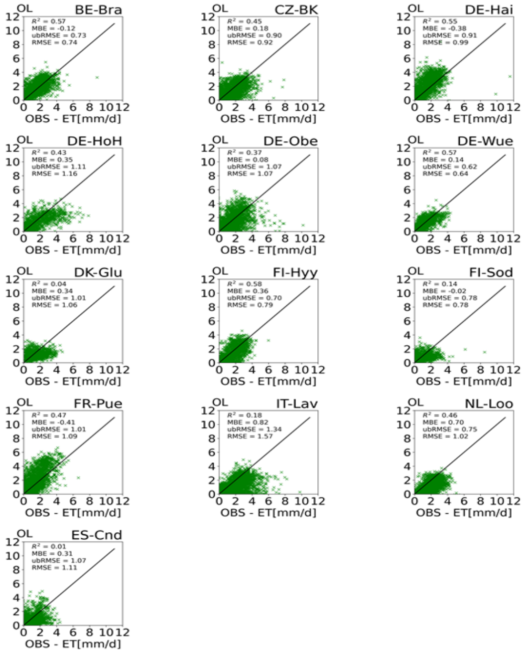
Figure 6: Scatter plots of observed evapotranspiration at thirteen study sites versus OL simulation results. The points represent daily averages for the days on which observation data are available.
