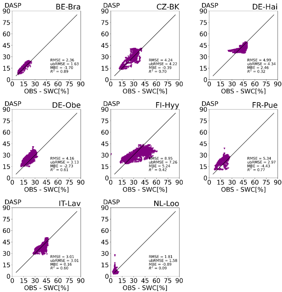
765 Figure A7: Scatter plots of observed soil water content at eight study sites versus DASP simulation results at 50 cm depth. The points represent daily averages for the days on which observation data are available.
