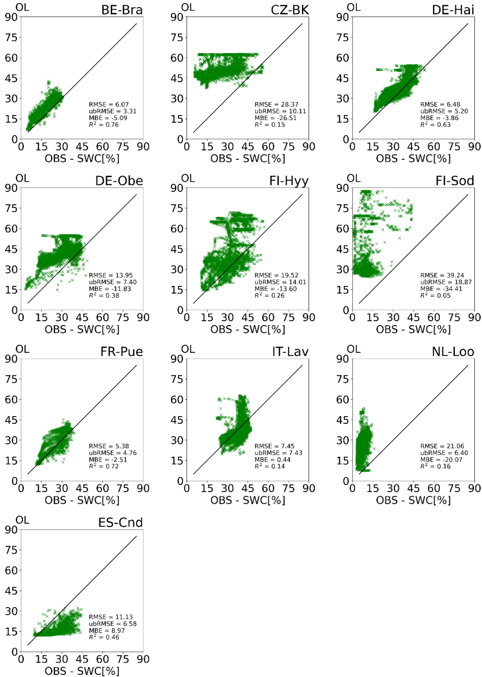
Figure A1 : Scatter plots of observed soil water content at ten study sites versus OL simulation results at
