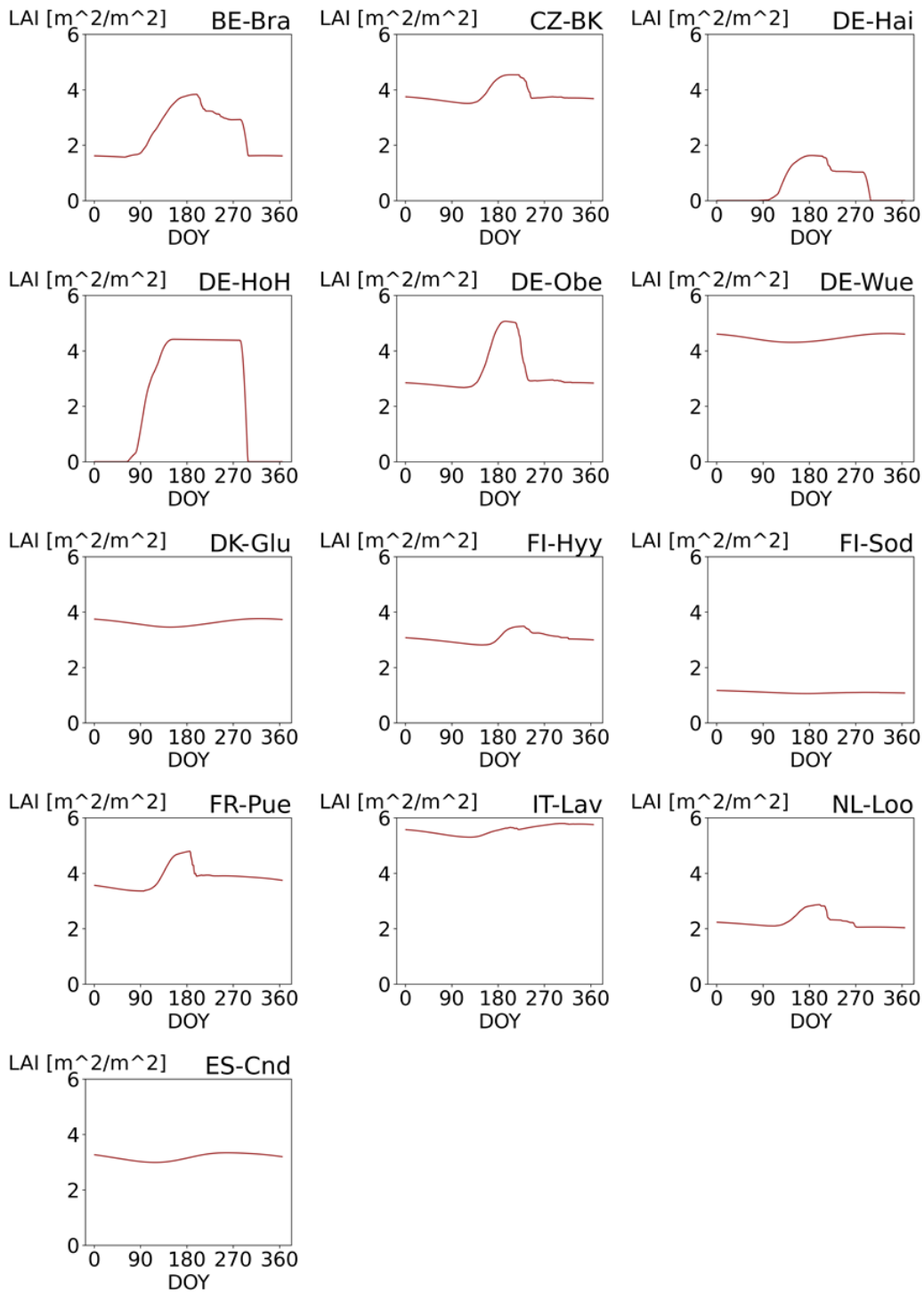
Figure 14: Seasonality of simulated (DASP) Leaf Area Index for each of the sites.
