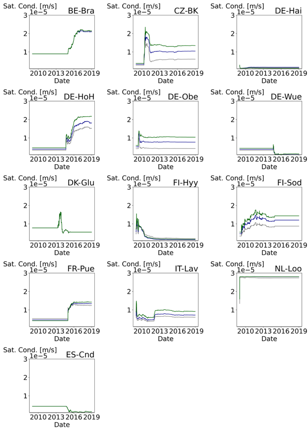
700 Figure 5: Time series of the saturated soil hydraulic conductivity for each site in the DASP simulation. The grey line is the value at 5 cm depth, the blue line at 20 cm depth, and the green line at 50 cm depth.
