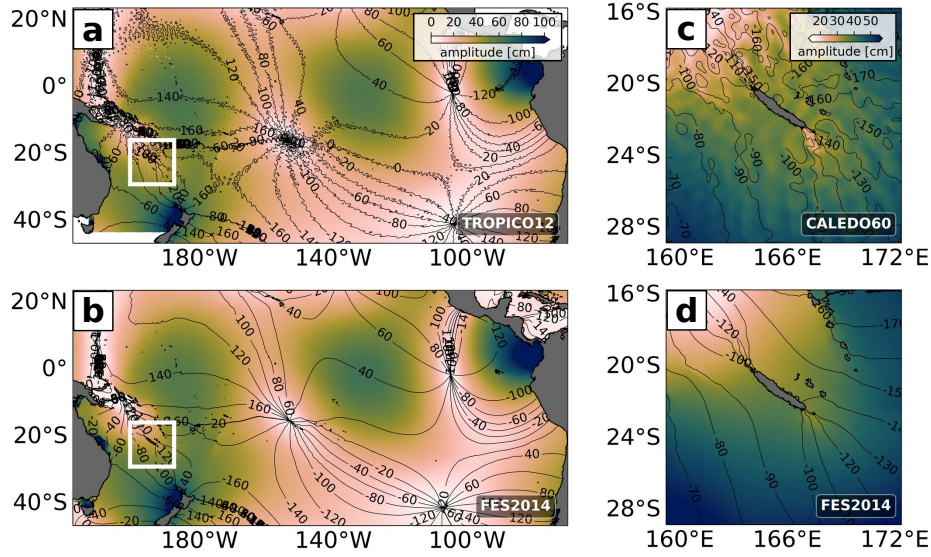
Figure 5. Barotropic M2 SSH amplitude (shading) and phase (contour) for (a) TROPICO12 and (c) CALEDO60 based on a 1-year (2014) harmonic analysis (assuming that the model SSH is dominated by the barotropic tide) and in comparison to the global tide atlas FES2014 for (b) TROPICO12 and (d) CALEDO60. The insets in (a) and (b) indicate the location of the CALEDO60 domain.
