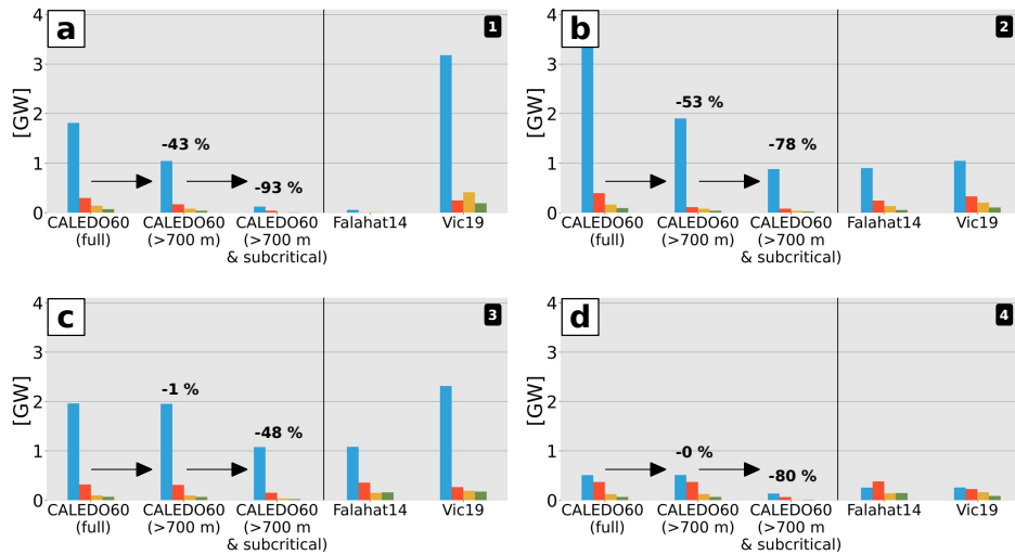
Figure 10. M2 barotropic-to-baroclinic energy conversion in GW for the four lowest modes integrated over (a) North , (b) South , (c), Norfolk Ridge , and (d) Loyalty Ridge for the full model, corrected for the upper 700 m, and corrected for both the upper 700 m and critical to supercritical slopes. The associated percentage decrease for the given correction is also shown. Energy conversion is compared to the semi-analytical estimates from Falahat et al. (2014) (Falahat14) and Vic et al. (2019) (Vic19) corrected for the upper 700 m.
