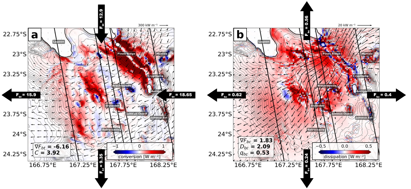
Figure 12. Regional M2 energy budget for the South (2) domain showing (a) the barotropic-to-baroclinic conversion (shading) overlaid by the barotropic energy flux (vectors) and (b) the depth-integrated baroclinic energy dissipation overlaid by the depth-integrated baroclinic energy flux (vectors). The area-integrated values for the barotropic energy flux divergence ( \nabla F_{bt} ) and barotropic-to-baroclinic conversion C in (a) and the baroclinic energy flux divergence ( \nabla F_{bc} ), the baroclinic energy dissipation D_{bc} , as well as the ratio of locally dissipated baroclinic energy q_{bc} in (b) are also given. The incoming/outgoing (a) barotropic and (b) baroclinic energy flux with integrated values along the boundary are illustrated at the lateral boundaries of the domain indicating the net direction of energy propagation. All integrated quantities are given in GW. The Pines Ridge, the lagoon and the most prominent seamounts are labeled. The depth contour interval is 100 m. The SWOT swaths and nadir track (solid black lines) during the fast-sampling phase (1-day repeat orbit) are also shown.
