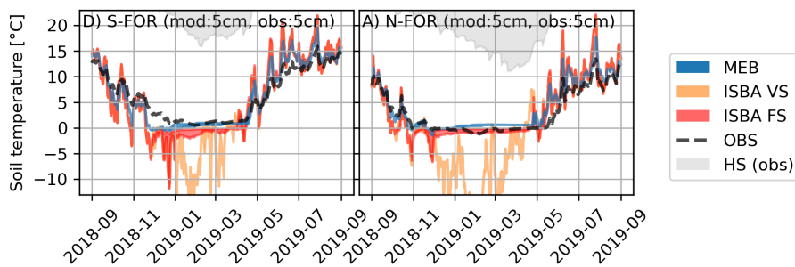
Figure 10. Effect of alternative configurations of ISBA and MEB on soil temperatures. The envelopes visualize the corresponding ensemble spreads. The observed evolution of the snow depth (HS) is not in scale. The observed soil temperatures are compared to the closest model layer; the depths of measurements and simulations are presented in each panel.
