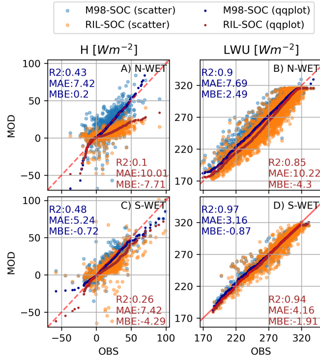
Figure 6. Scatterplots and quantile-quantile plots of sensible heat flux (H) and upward longwave radiation (LWU) during snow cover for the evaluation period with the RIL-SOC and M98-SOC turbulence parameterizations.
