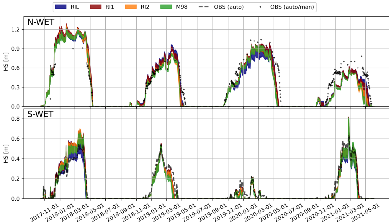
Figure 5. Time series of snow depths (HS) simulated by ISBA-FS ESCROC- E_2 . The 35 ensemble members are grouped by their turbulent flux parameterization, and the spread of each group is presented in colored ranges. Observed snow depths are presented in black dots and dashed lines.
