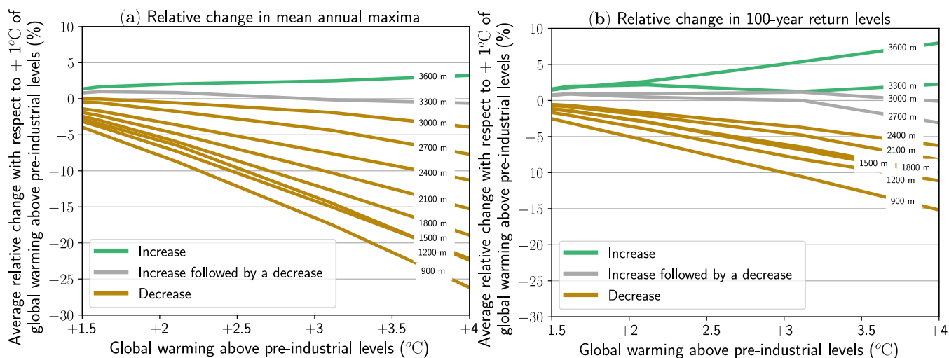
Figure 4. Average relative changes in (a) mean annual maxima (b) 100-year return levels of daily snowfall, every 300 m of elevation from 900 m to 3600 m, between +1.5 and +4°C global warming levels. Relative changes are computed with respect to the current climate (corresponding here to +1°C of global warming), and are averaged over all available massifs of the French Alps.
