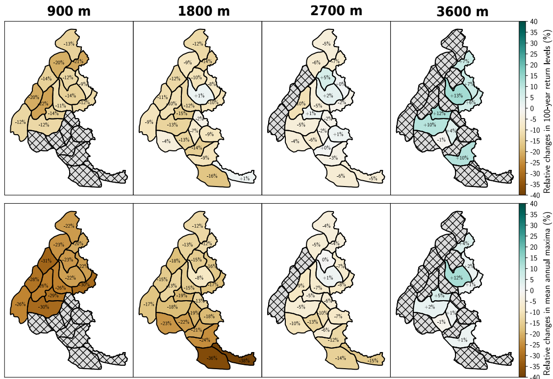
Figure 2. Relative changes in mean annual maxima and 100-year return levels of daily snowfall between the current climate (corresponding here to +1^\circ\text{C} of global warming) and +4^\circ\text{C} of global warming at elevations 900 m, 1800 m, 2700 m, and 3600 m. Hatched grey massifs denote massifs that are not available (Sect. 3, second step of our analysis).
