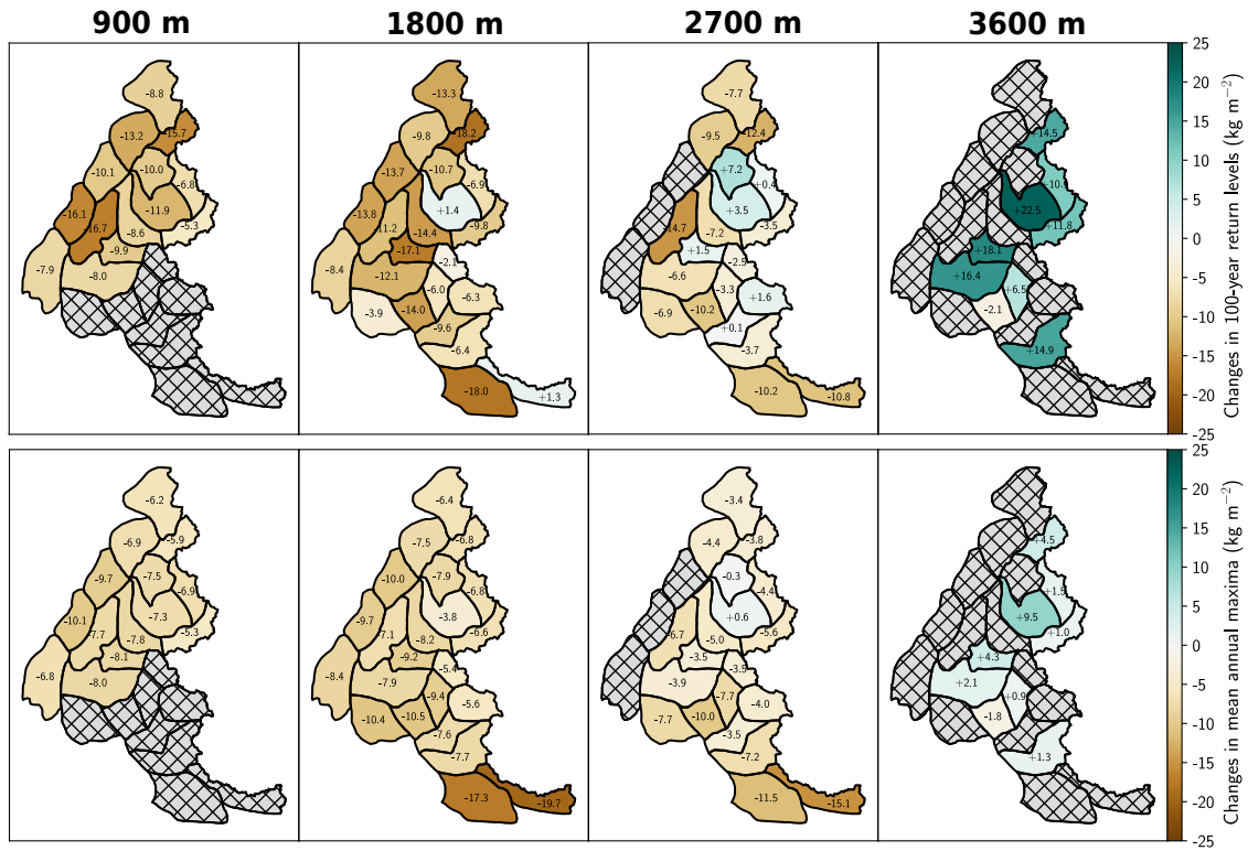
Figure 3. Absolute changes in mean annual maxima and 100-year return levels of daily snowfall between the current climate (corresponding here to +1°C of global warming) and +4°C of global warming at elevations 900 m, 1800 m, 2700 m, and 3600 m. Hatched grey massifs denote massifs that are not available (Sect. 3, second step of our analysis).
