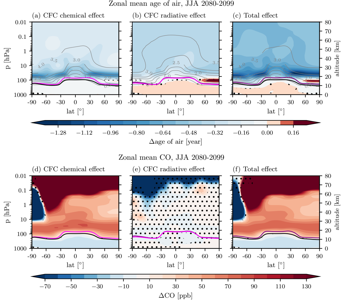
Figure B1. Top: age of air for JJA (other seasons look very similar) 2080-2099, bottom: CO. The left column shows the CFC chemical effect, the center column the CFC radiative effect and the right column the total effect of CFC chemical and radiative effect combined. Stippling indicates not significant at a 90 % confidence level. The tropopause height is indicated in purple for the noMPA, in magenta for noMPA_CFCRadOff and in black for the reference experiment.
