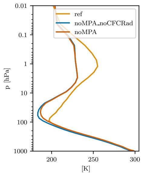
Figure D1. Tropical (30° N-S) zonal mean temperature profiles of noMPA, noMPA_CFCRadOff and ref in JJA 2080-2099.
