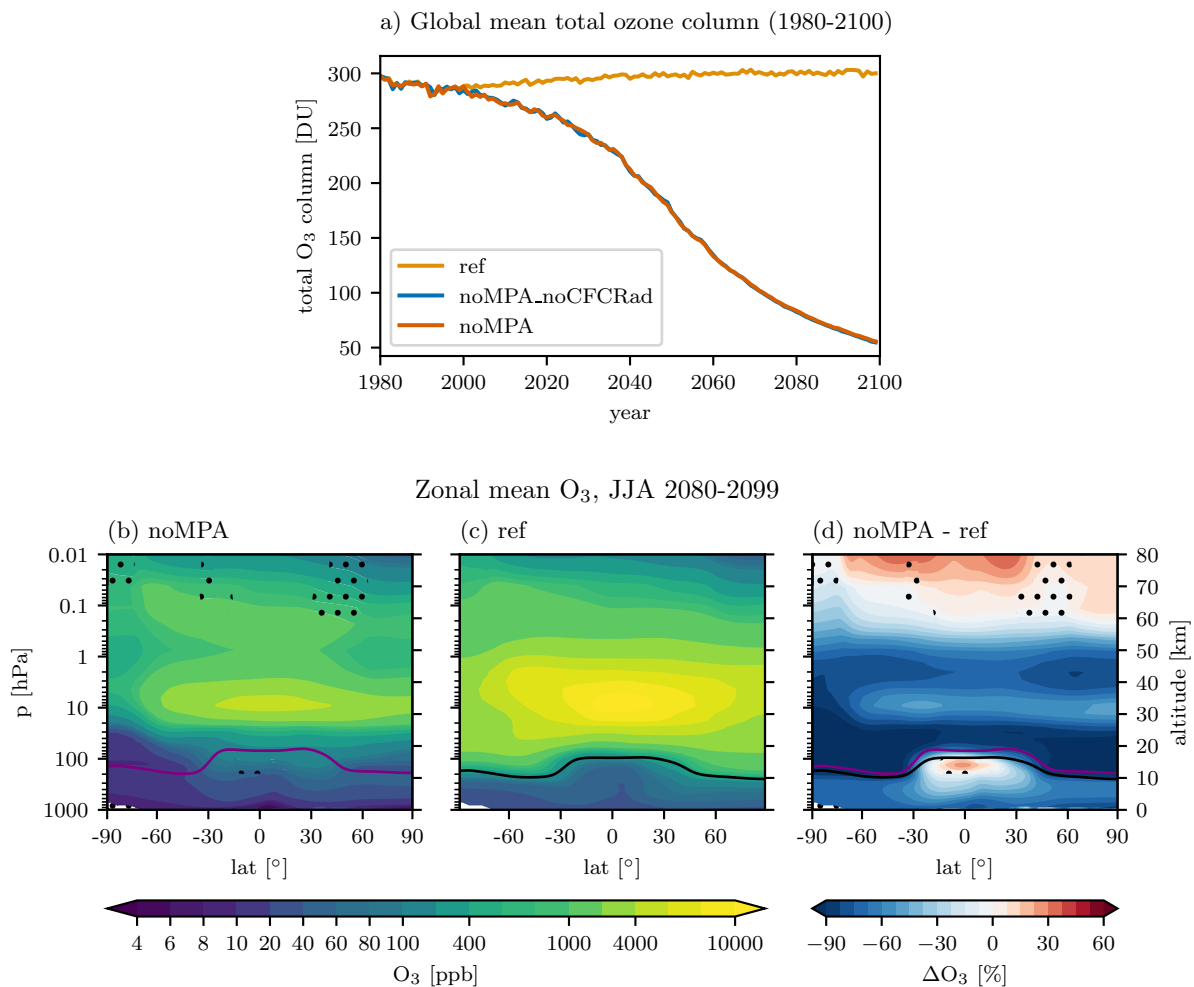
Figure 1. Top: Global mean total ozone column evolution from 1980-2099 for the reference, noMPA and noMPA_noCFCRad scenarios. Bottom: Zonal mean ozone noMPA (b), ref (c) and differences in % of noMPA–ref (d) for JJA 2080–2099. The tropopause height is indicated in purple for the noMPA and in black for the MPA reference experiment. Stippling indicates not significant at a 90 % confidence level. Colorbar levels for b and c are evenly numbered in log spacing.
