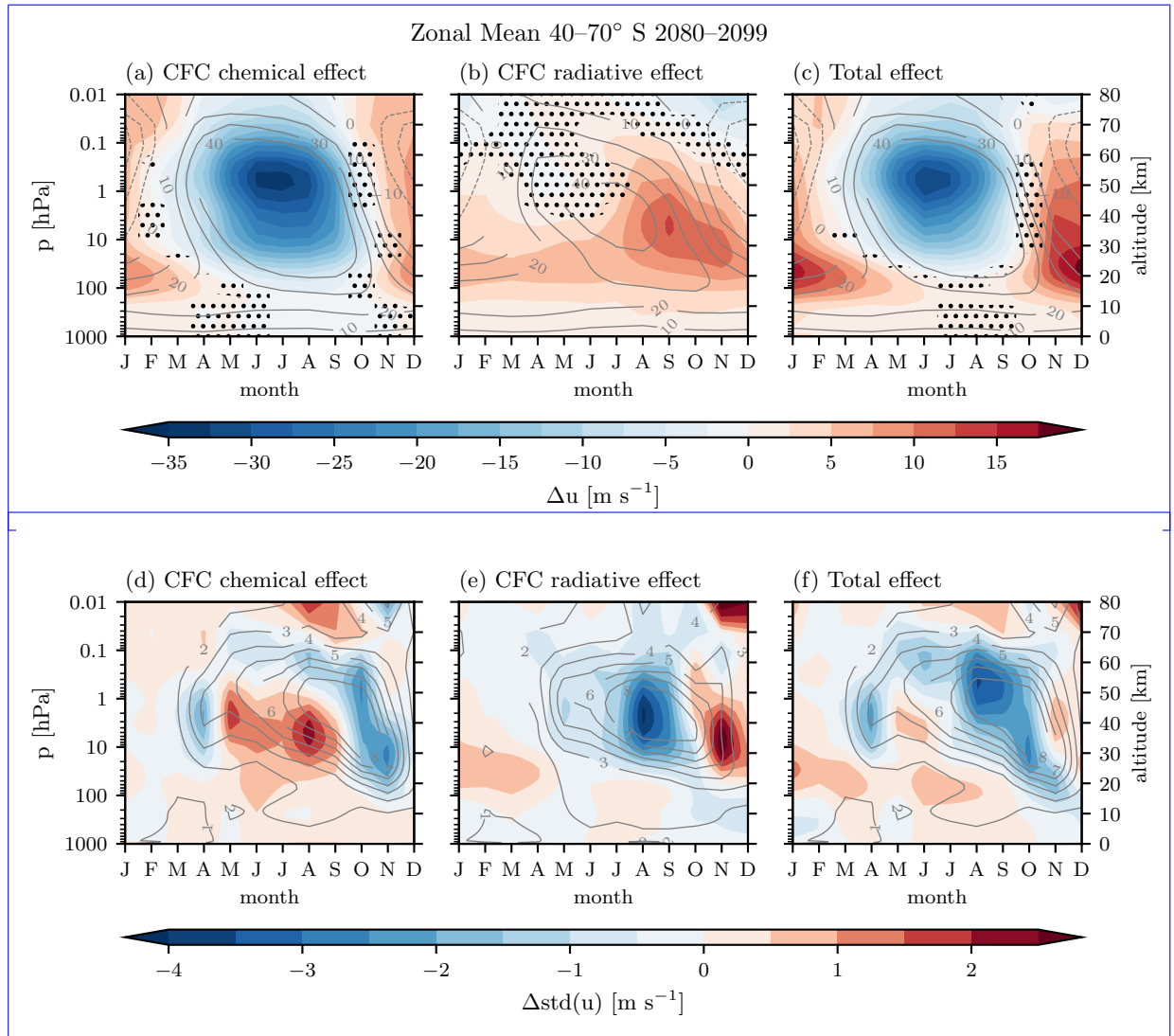
Figure 5. 40–70° S zonal mean wind differences (upper row) and zonal mean standard deviation differences for zonal wind (bottom row) for each month of 2080–2099. The left column shows CFC chemical effect (noMPA_CFCRadOFF–ref), the center column the CFC radiative effect (noMPA–noMPA_CFCRadOFF) and the right column the total effect of CFC chemical and CFC radiative effect combined (noMPA–ref). Stippling indicates not significant at a 90 % confidence level. The contour lines indicate the ref zonal wind profile in the top row and the ref standard deviation in the bottom row. Note that the color saturation is different for negative and positive values.
