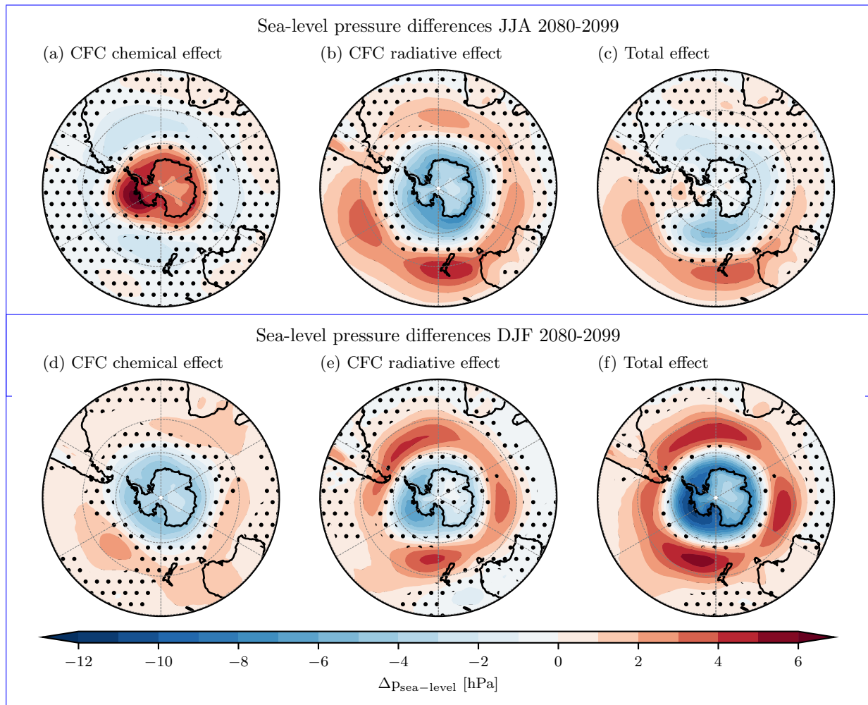
Figure 6. 2080-2099 Antarctic winter (upper row) and summer (lower row) sea-level pressure differences. CFC chemical effect (a, d), CFC radiative effect (b, e) and total effect (c, f). Stippling indicates not significant at a 90 % confidence level.
