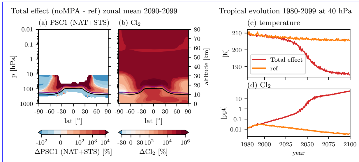
Figure 2. Left: 2090-2099 annual mean zonal mean of PSC Type 1 (nitric acid trihydrate (NAT) and supercooled ternary solution (STS)) (a) and Cl 2 (b) differences in % for the total effect (noMPA–ref). The tropopause height is indicated in purple for the noMPA and in black for the MPA reference experiment. Colorbar levels for (a) and (b) are linear around 0 and log spacing < -10 % and > 10 % for (a) and > 30 % for (b). Right: Evolution of tropical mean (23° N – 23° S) temperature (c) and Cl 2 (d) anomalies at 40 hPa from 1980 to 2099 for the total effect (noMPA-ref). Note that (d) has a log y-axis.
