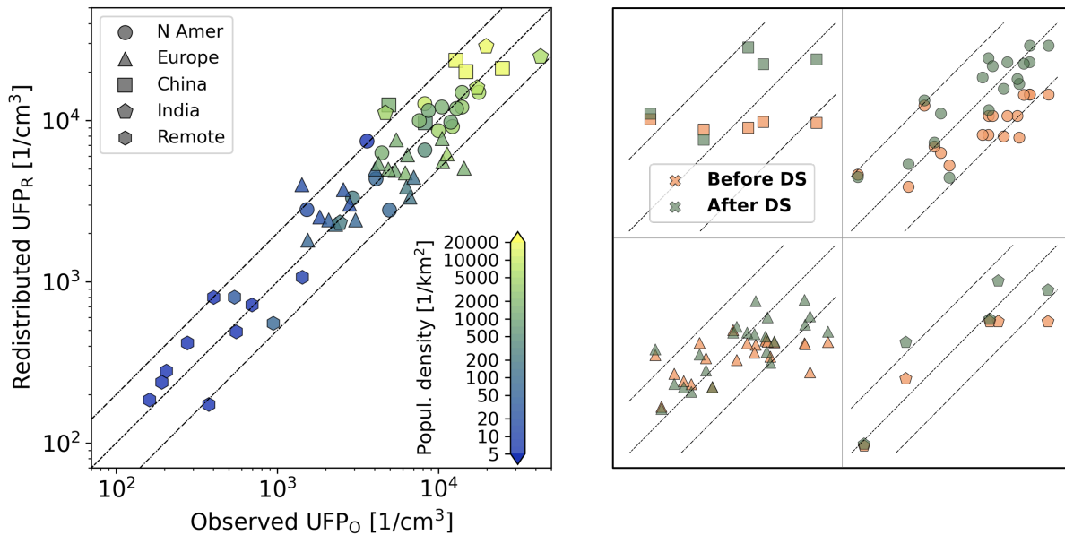
Figure 11. Left: Same as Fig. 7, but after the redistribution of UFP M concentrations (downscaling) based on the relative anthropogenic emissions per grid box (more details in the text). Right: Evaluation results before and after the downscaling (DS) for China, North America Europe and India (from top left to bottom right). Note that the value range differs in all subpanels.
