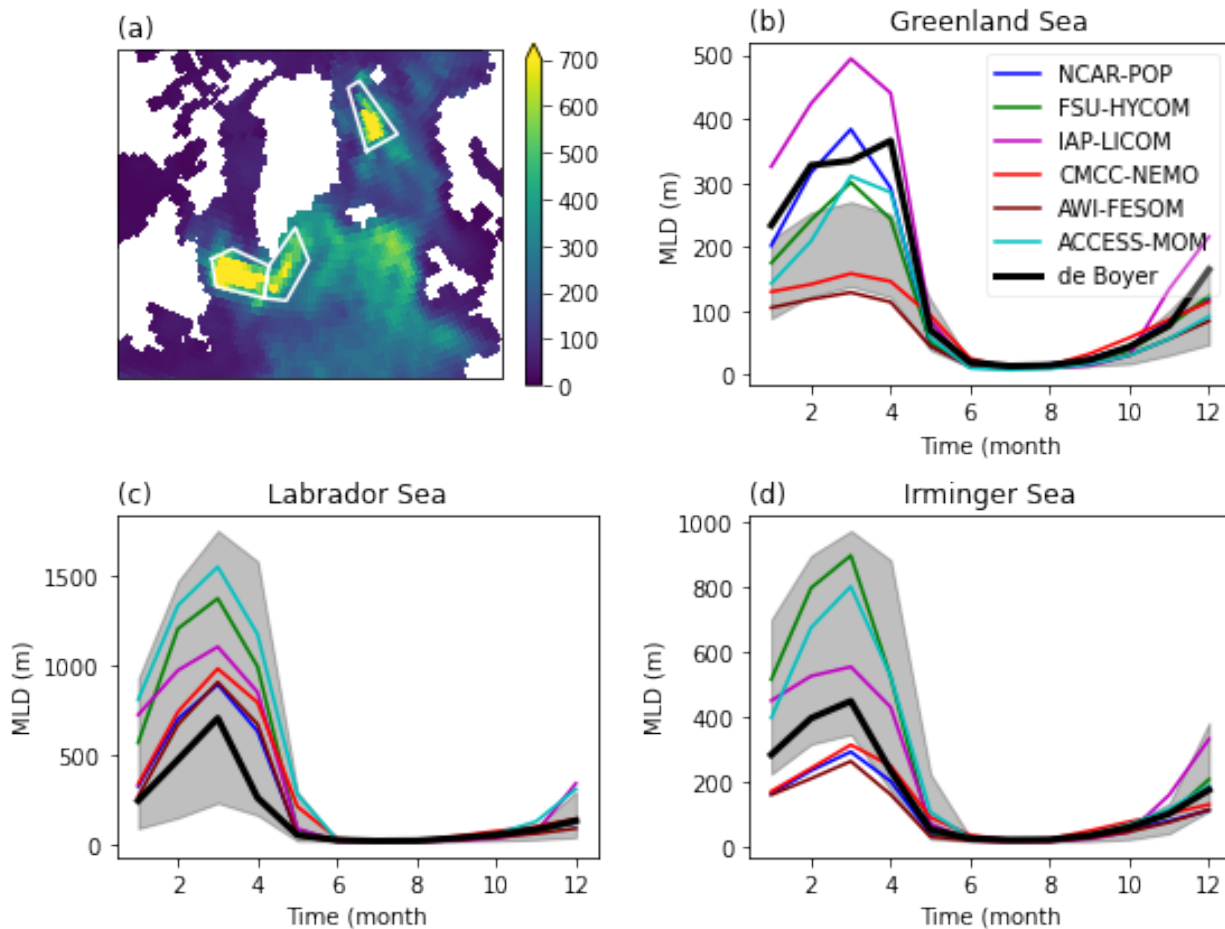
540 Figure 10 : Seasonal cycle of MLD in three regions. (a) map of the maximum MLD (de Boyer Montégut, 2022) indicating the three regions of deep water formation (Labrador Sea, Irminger Sea, and Greenland Sea). In panels (b-d), the seasonal cycle of the observed MLD (m) averaged over each region is plotted in black and the high resolution models in color. The time axis is in months. The grey area is the range of the low resolution model MLDs.
