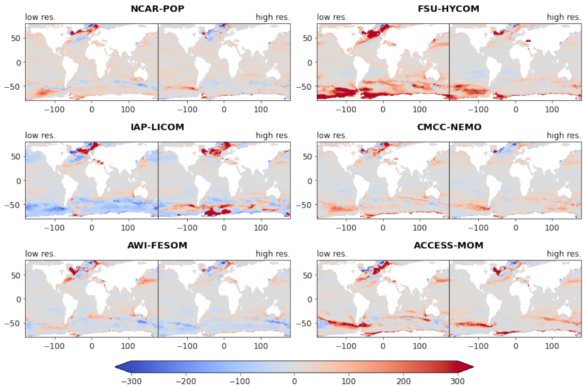
Figure 7 : MLD biases (m) of models in winter, relative to de Boyer Montégut (2022). For each model, biases are shown for both the low resolution version (left panel) and the high resolution version (right panel). The MLD has been recomputed from monthly archives, with the same potential density threshold and 10 m reference depth as the observations, except for CMCC-NEMO at high resolution where the MLD has been computed online using a reference level of 0.5 m (see text for details). The winter MLD is the average over the months of January to March in the Northern Hemisphere, and July to September in the Southern Hemisphere.
