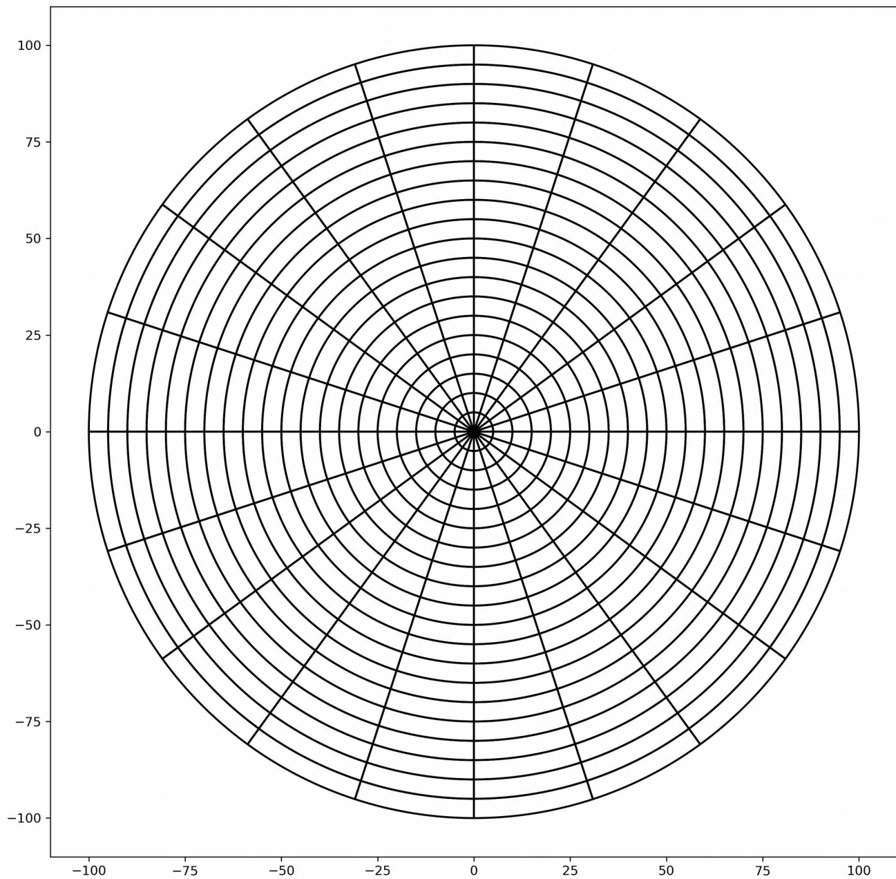
Figure S1: Radial grid or circular grid, created by drawing 20 concentric circles within the radius of 100km, and each circle is further divided into 20 arcs, thereby providing a radial grid with 400 spatial cells. The radial grid provides a simplest form of a multi-resolution grid with the area of each cell increasing away from center.
