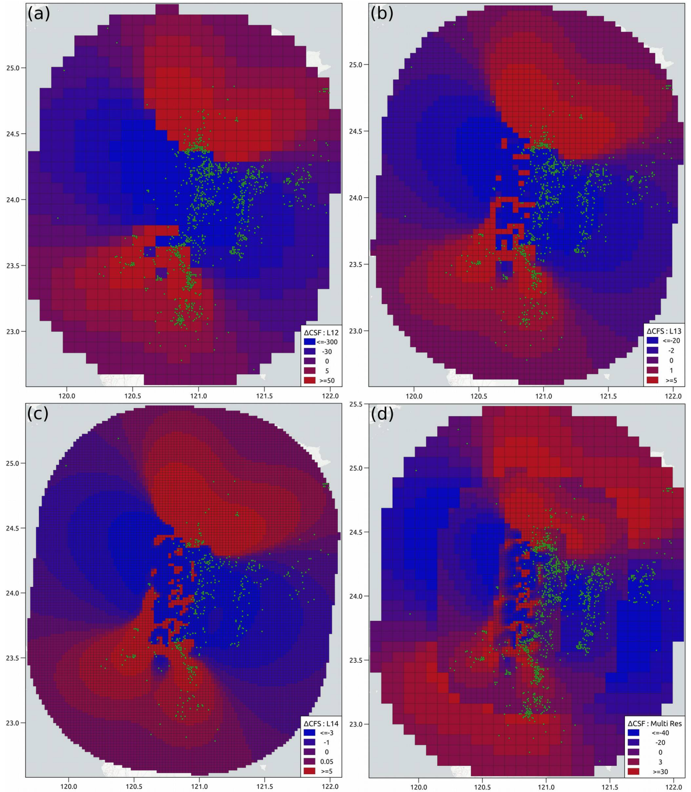
Figure S2: CFS aftershocks forecast model for 1999 Chi-Chi earthquake aggregated on the Quadtree grids of different resolutions. The forecast shown here is from 3D cells around depth 7.5km aggregated on: (a): single-resolution grid L12, (b): single-resolution grid L13, (c): single-resolution grid L14, (d): multi-resolution grid.
