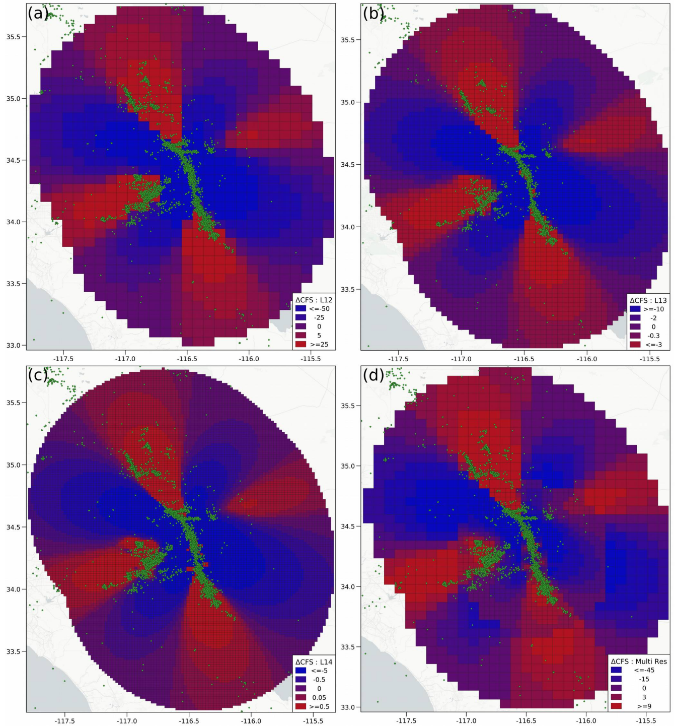
Figure S3: Coulomb aftershocks forecast model for Landers 1992 earthquake aggregated on the Quadtree grids of different resolutions. The forecast shown here is from 3D cells around depth 7.5km aggregated on: (a): single-resolution grid L12, (b): single-resolution grid L13, (c): single-resolution grid L14, (d): multi-resolution grid.
