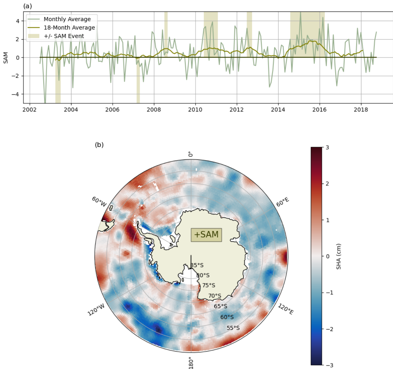
Figure 7: a) Timeseries of Southern Annular Mode (SAM) index smoothed over 18 months. Months with a SAM index greater than 2 standard deviations and less than 0 are highlighted in pale green. B) Composite plot of SHA within months in which the SAM index is greater than 2 standard deviations. SHA has also been smoothed over 18 months. Data quality may vary regionally; please refer to Section 3.1 for validation results.
