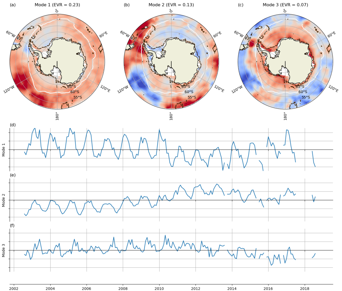
230 Figure 5: Spatial signatures of Modes 1 (a), 2 (b) and 3 (c) resulting from EOF analysis of SHA. The colour scale is arbitrary but consistent across (a), (b) and (c) and centred at zero. The Explained Variance Ratio (EVR) is shown in the title. The sea ice maximum is demarcated in white (solid), and the -1000m isobath in black (dashed). Temporal signatures of Modes 1 (d), 2 (e) and 3 (f). The scale on the y-axis is arbitrary but consistent across (d), (e) and (f) and centred at zero. Data quality may vary regionally; please refer to Section 3.1 for validation results.
