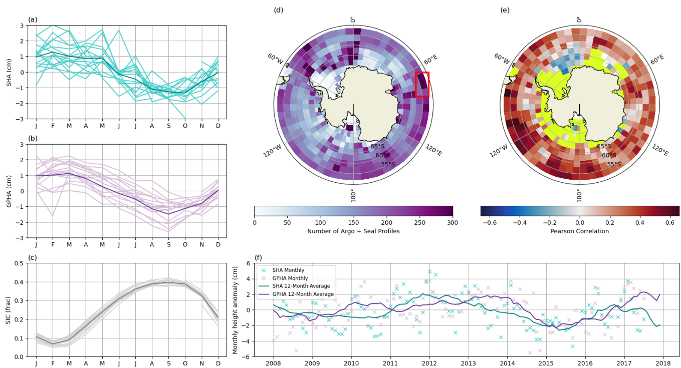
205 Figure 3: Validation of SHA against GPHA from Argo and seals profiles. (a) The monthly average SHA (darker line) across the entire domain. (b) The monthly average GPHA across the entire domain. (c) The monthly average Sea Ice Concentration (SIC) across the entire domain. Individual years' data are shown as lighter lines in (a), (b) and (c). (d) The total number of profiles recorded within each grid square. The red box outlines the region from which the data in (f) have been taken. (e) The Pearson correlation coefficient between the SHA and GPHA for each grid square. Pixels with fewer than 36 months of data are masked in yellow. (f) Comparison between the SHA and GPHA timeseries for the location shown in (d). Monthly measurements are shown with an 'x' and the 12-month rolling mean a solid line.
