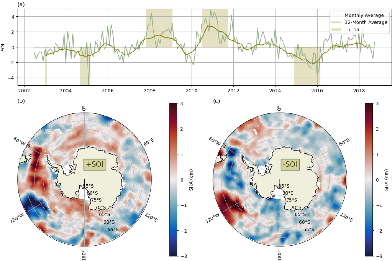
270 Figure 6: a) Timeseries of Southern Oscillation Index (SOI) smoothed over 12 months. Months showing a SOI greater than 1 standard deviation and less than -1 standard deviation highlighted in pale green. b) Composite plot of SHA within months where the SOI is greater than 1 standard deviation. c) As b), but where the SOI is less than -1 standard deviation. SHA has also been smoothed over 12 months. Data quality may vary regionally; please refer to Section 3.1 for validation results.
