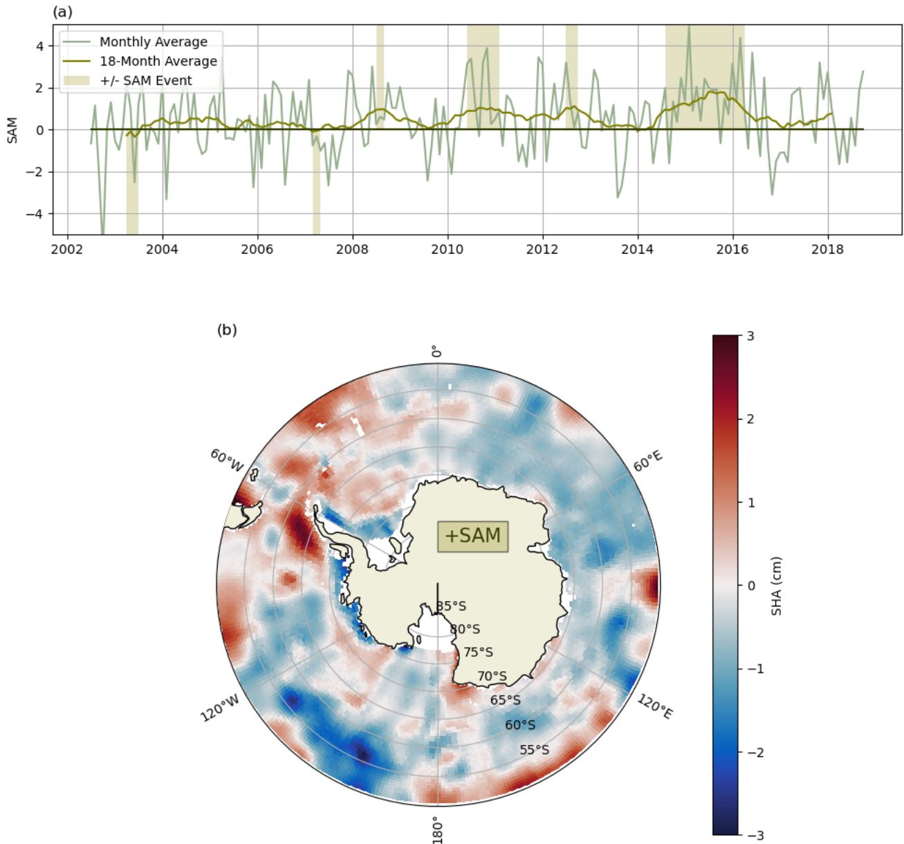
Figure 7: a) Timeseries of Southern Annular Mode (SAM) index smoothed over 18 months. Months showing with a SAM index greater than 2 standard deviations and less than 0 are highlighted in pale green. B) Composite plot of SHA within months in which the SAM index is greater than 2 standard deviations. C) As b), but where the SAM index is less than 0. SHA has also been smoothed over 18 months. Data quality may vary regionally; please refer to Section 3.1 for validation results.
