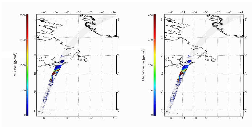
Figure 4. M-CWP of the HALIFAX scene (left) and the error of M-CWP (right)
