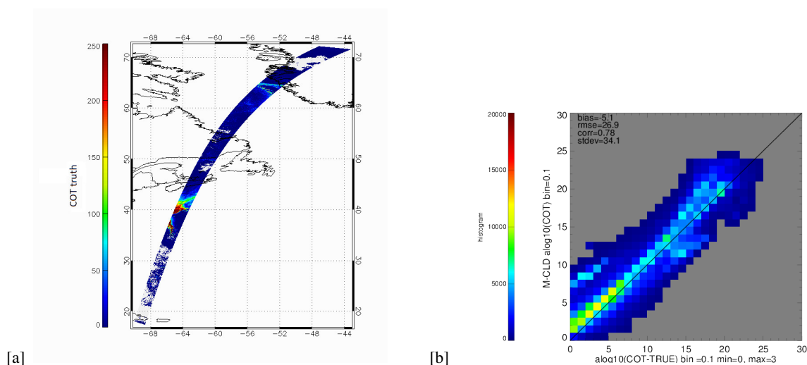
Figure 5. Cloud optical thickness for the Halifax scene a) true cloud optical thickness at 680nm and b) Histogram of the true COT and M-COT
