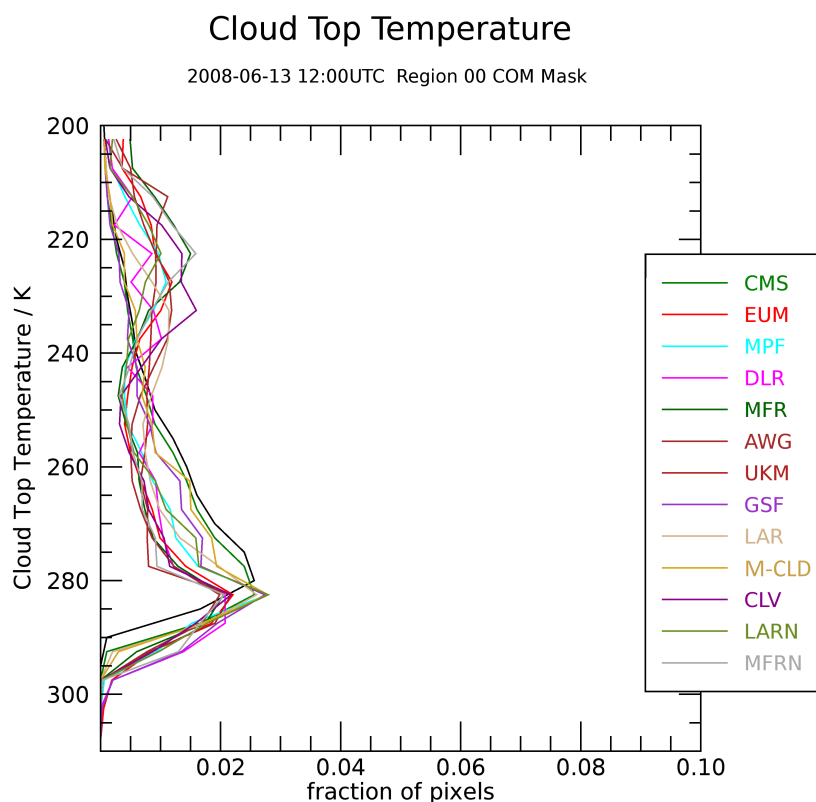
Figure 8. Histograms of the cloud top temperature of the thirteen ICWG algorithms for 13-06-2008 at 12:00 UTC based on a common cloud mask.
