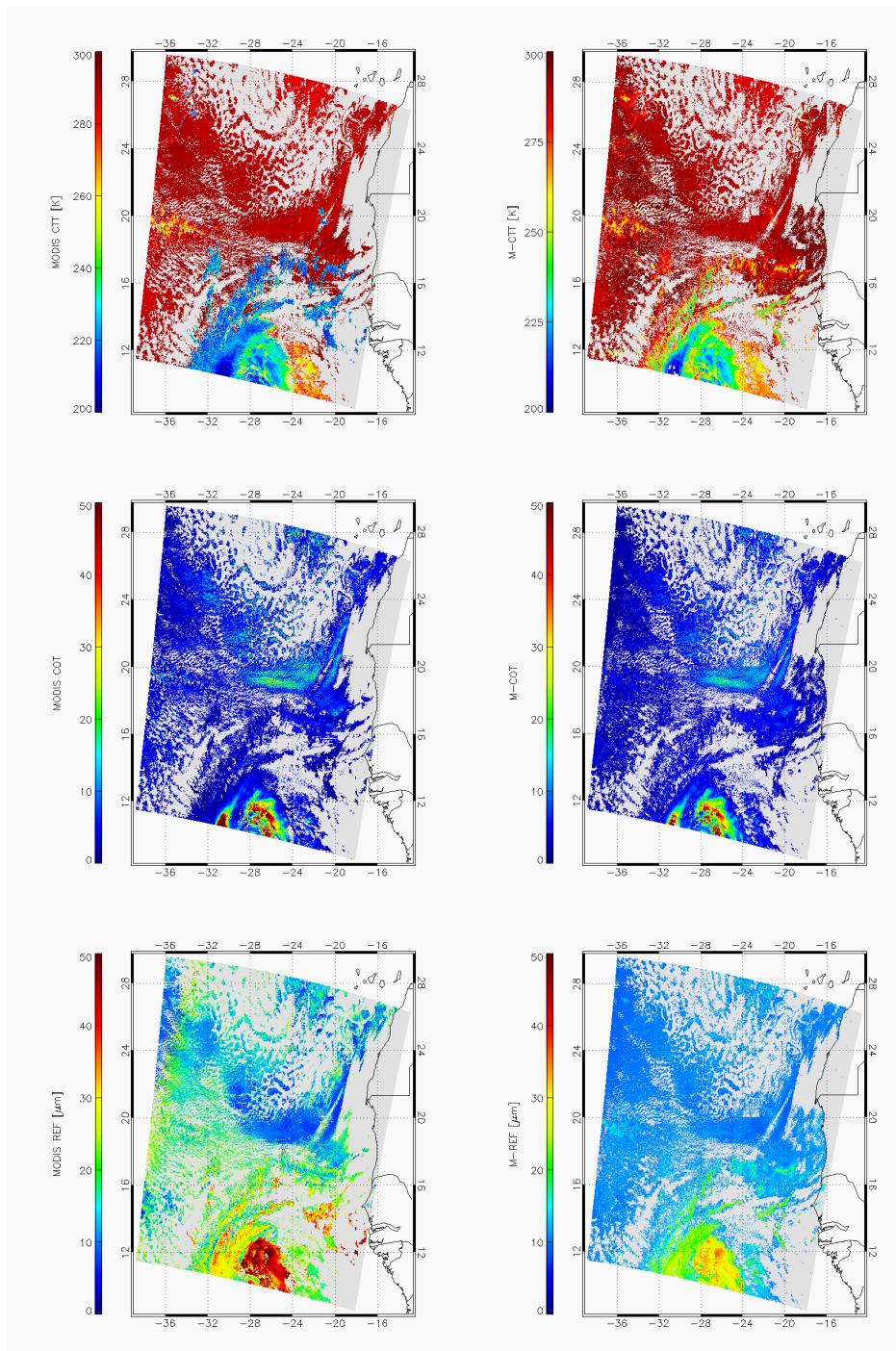
Figure 6. Case study from MODIS Terra granule at 1220UTC, 30 September 2021. The top row shows the cloud top temperature, the middle panel shows the cloud optical thickness and the bottom row shows the cloud effective radius at 1.6 \mu\text{m} , whereby the left column belongs to the MODIS L2 products and the right column to the M-CLD .)
