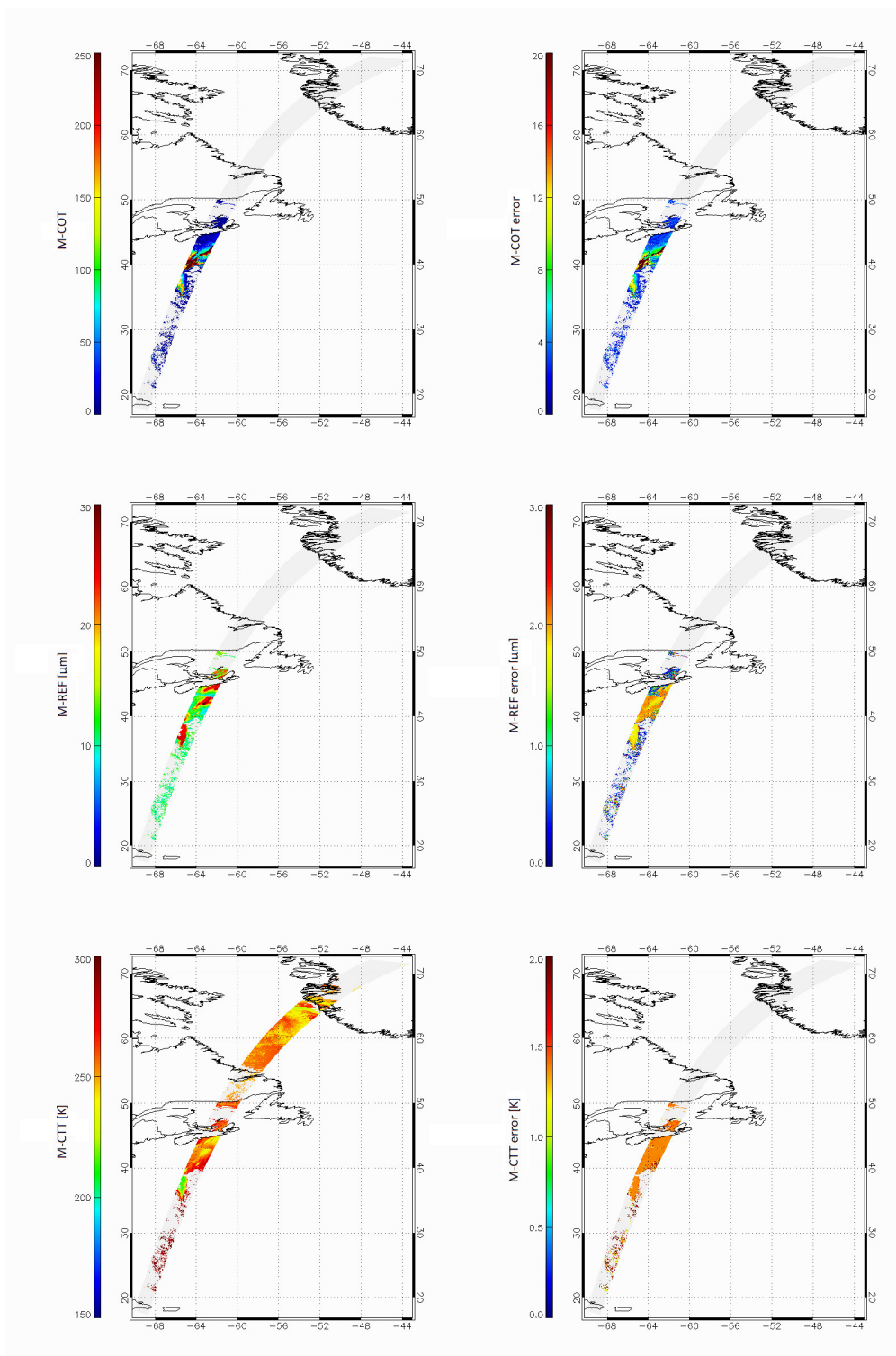
Figure 3. M-COP for the HALIFAX scene with: M-COT (top, left), error of M-COT (top, right), M-REF (middle, left), error of M-REF (middle, right), CTT (bottom, left), error of CTT (bottom, right)
