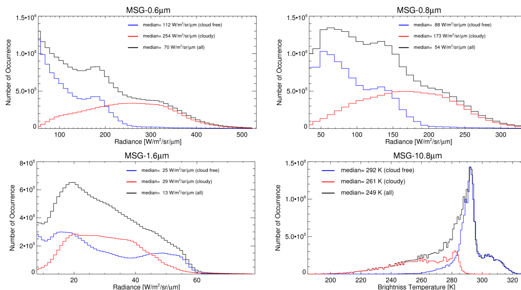
Figure 2. Histogram of the radiance in VIS, NIR, SWIR-1 and the brightness temperature TIR-2 based on SEVIRI measurements
