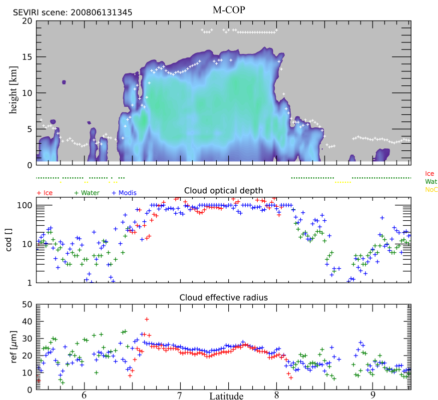
Figure 9. Selected CloudSAT, MODIS and M-COP (based on SEVIRI L1) cloud properties over West Africa with deep convection. Top panel, Cloud radar reflections are shown with the M-CTH (dotted white line). The middle panel gives on the track MODIS-COT(blue) and M-COT (with cloud phase red: ice, green: water) and the lower panel gives similar the cloud effective radius.
