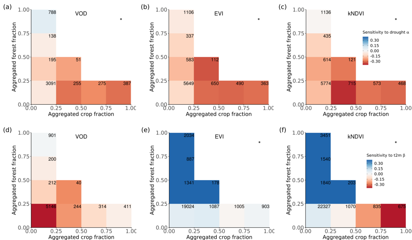
365 Figure 4. Ecosystem resistance to drought and temperature binned for different levels of the aggregated forest and cropland fraction classes from the three land cover products (a) L-VOD, (b) EVI and (c) kNDVI for drought resistance coefficients \alpha and (d-f) for temperature resistance coefficients \beta . Only significant coefficients \alpha in the linear model ( P -value < 0.05 ) are included and groups with less than 20 pixels are excluded. The number in each bin is the number of pixels in this category. Only pixels with no change in 25% bins of the four dominant vegetation categories (forests, shrublands, grasslands and croplands) are analyzed. Star on the upper right corner 370 indicate significantly higher resistance in forest > 75\% than crop > 75\% at the 0.05 significance level from the unpaired two-sample Wilcoxon test.
