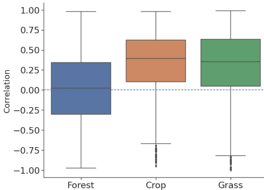
530 Figure 6. Correlation between yearly maximum L-VOD and kNDVI for different land cover types.
