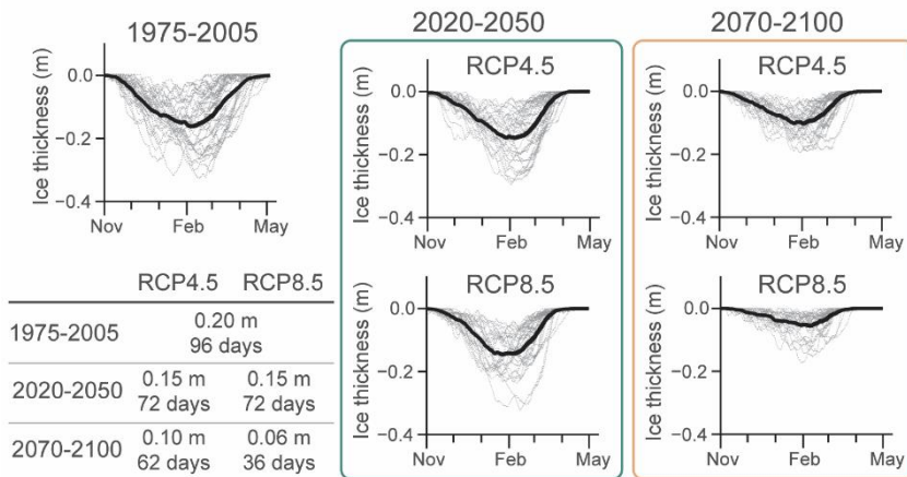
405 Figure 9. Average ice thickness in the Curonian Lagoon. Black line indicates the average ice thickness of each analysis period – historical (1975–2005), short-term (2020–2050), and long-term (2070–2100) under RCP4.5 and RCP8.5 scenarios. Table shows the average maximum ice thickness (m) and a percentage of change ice season duration (days) of the scenario runs compared with the historical period.
