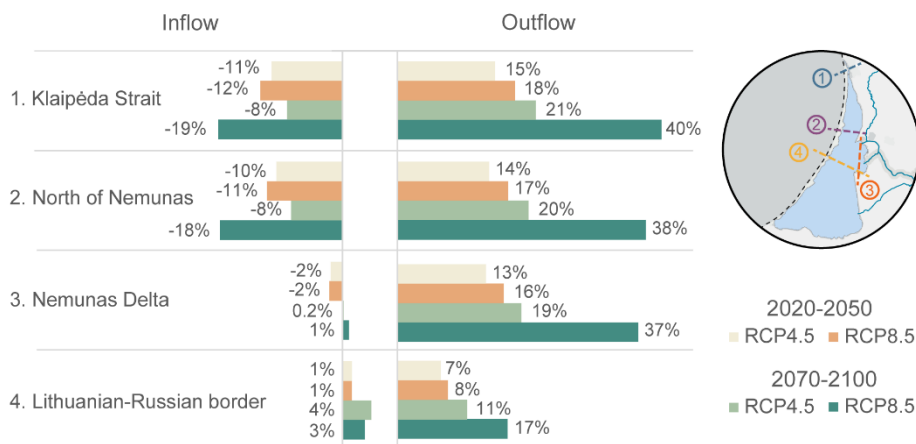
295 Figure 7. The percentage of change of projected (under RCP4.5 and RCP8.5 scenarios) inflowing and outflowing water flux from the historical period (1975–2005). The map insert shows the locations of the predefined cross-sections: 1 – Klaipėda Strait, 2 – North of Nemunas, 3 – Nemunas Delta, 4 – Lithuanian–Russian border. Outflow is from south to north (sections 1,2,4), and from east to west (section 3), inflow - vice versa.
