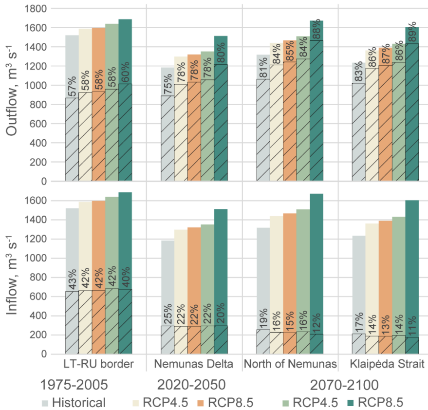
Figure 6. The percentage of the average outflowing and inflowing water volume (hatched pattern) including its percentage of the absolute flux (solid pattern) of each analysis period – historical (1975–2005), short-term (2020–2050), and long-term (2070–2100) under RCP4.5 and RCP8.5 scenarios. The locations of cross-sections are shown in Fig. 7. The bottom graph is for reference, indicating the average water flux in m^3 s^{-1} during the historical period (1975–2005).
