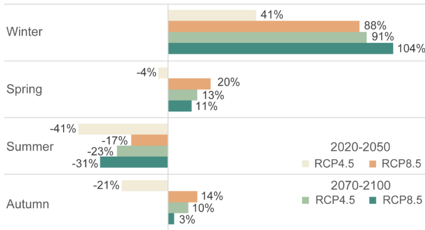
Figure 5. The percentage of change of seasonal average discharge from the Nemunas River for the RCP4.5 and RCP8.5 scenario runs during the short-term (2020–2050) and long-term periods (2070–2100), compared with the historical period (1975–2005).
