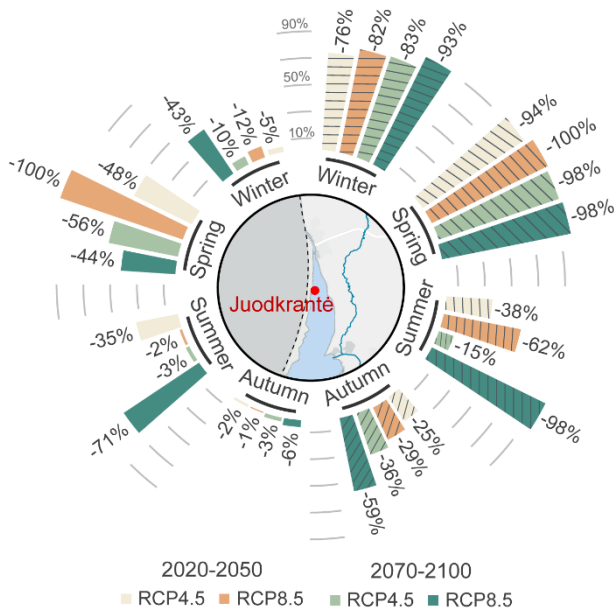
340 Figure 8. The percentage of change of seasonal average salinity of saltwater intrusions (solid pattern – left) and number of days when salinity exceeded the 2 \text{ g kg}^{-1} threshold (hatched pattern – right) in Juodkrantė, approximately 20 km below the strait connecting the Baltic Sea and the Curonian Lagoon. Values denote the percentage of difference of the scenario runs compared with the historical period (1975–2005).
