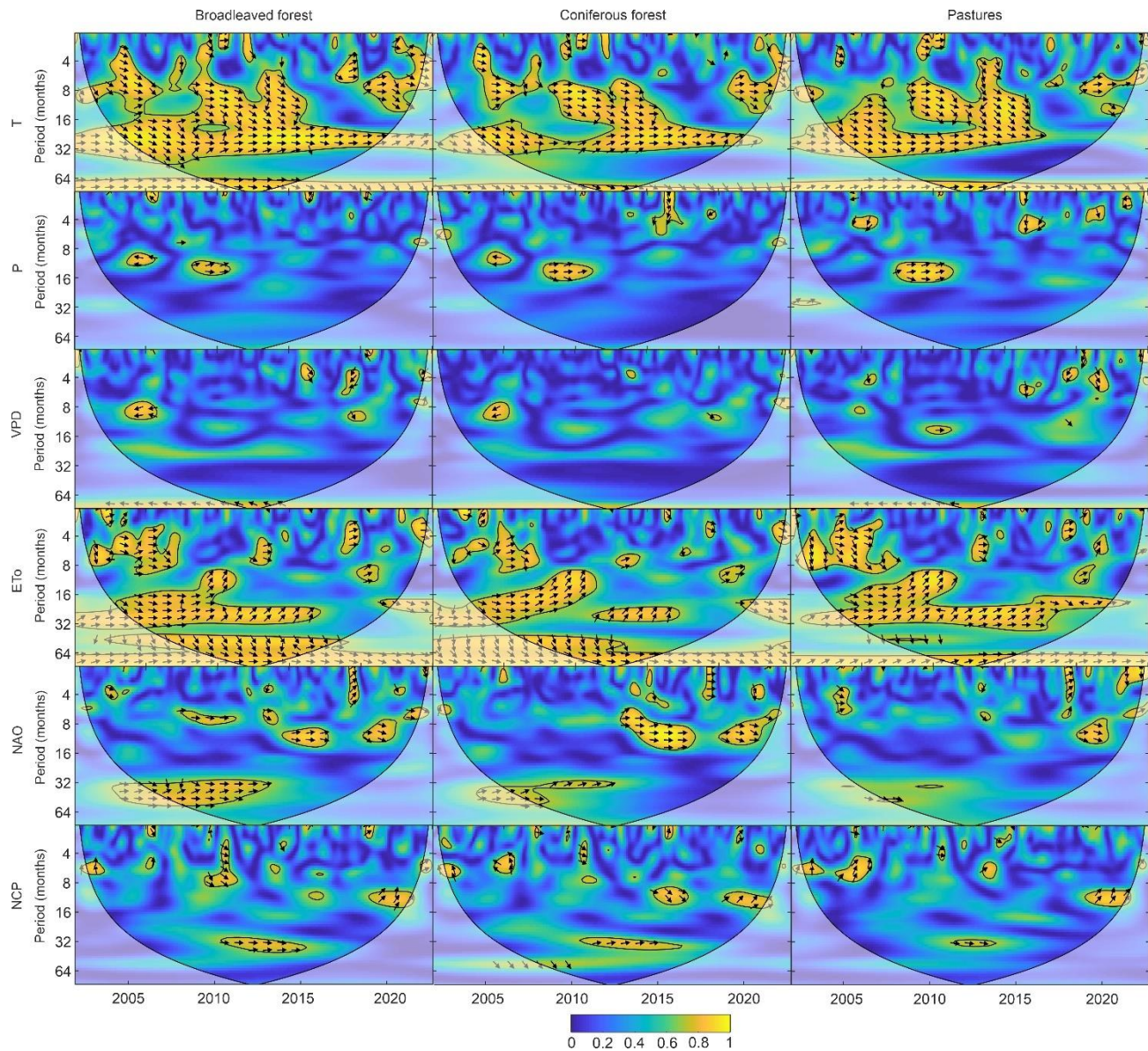
Fig. 6. Wavelet Coherence power spectrum (colour scale) between deseasonalised time series of NDVI and T, P, VPD, ET 0 , NAO and NCP for broadleaved forest (left column), coniferous forest (middle column) and pastures (right column) during the period 2002-2022. Colours range from blue (low correlation) to yellow (high correlation). Arrows indicates the phase difference between signals: right arrows – series are completely in phase, left arrows – series are out of phase. The COI region is below the thick black line. Statistically significant areas at the level of \alpha = 0.05 are indicated by a thin black line.
