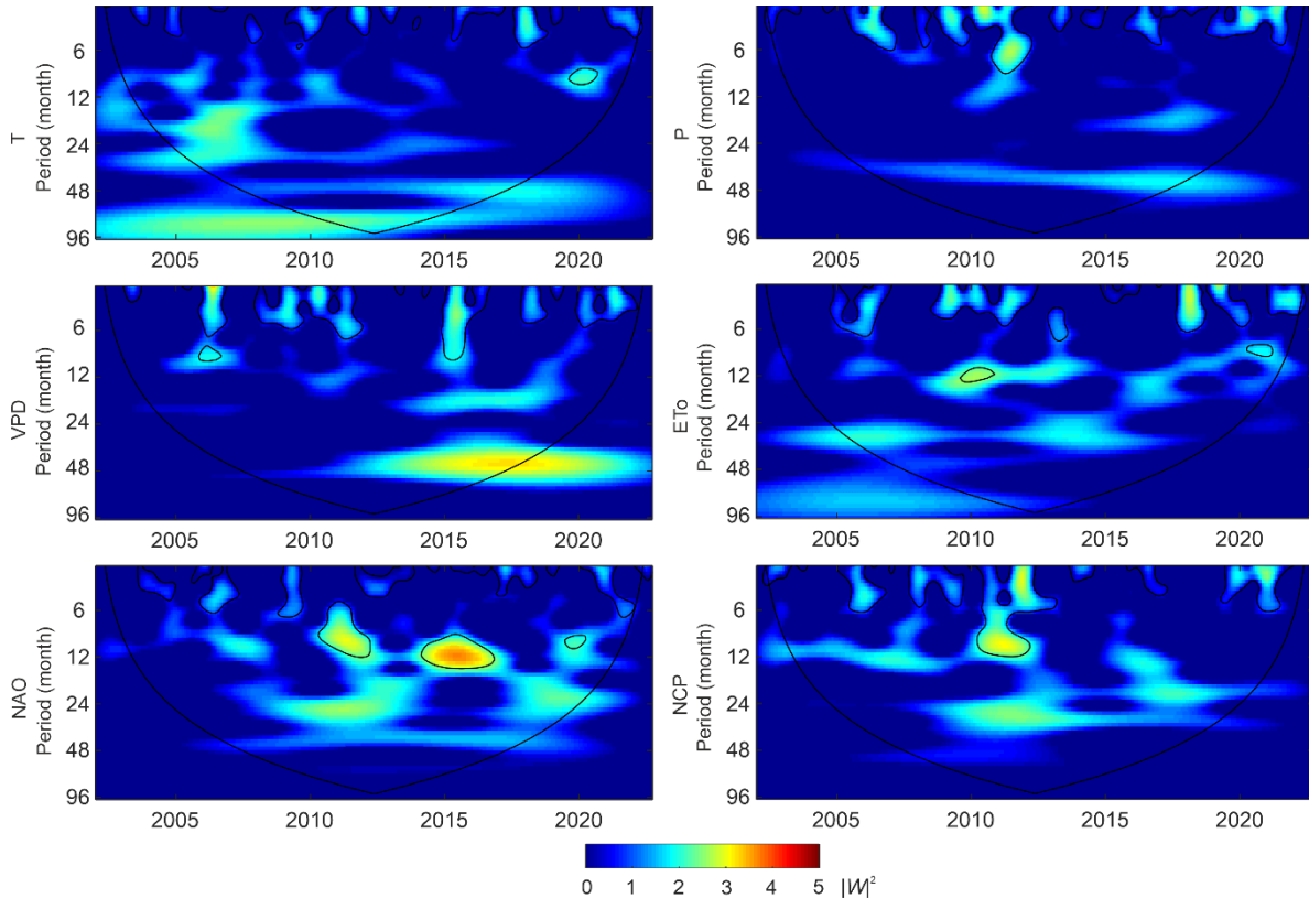
Fig. 5. Wavelet power spectrum ( |W|^2 ) for deseasonalised time series of T, P, VPD, ETo (mean value from three vegetation masks), and NAO and NCP during the period 2002-2022. The COI region is below the thick black line. Statistically significant areas at the level of \alpha = 0.05 are indicated by a thin black line.
